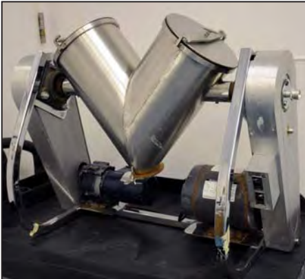
PATTERSON KELLY stainless steel V blender
