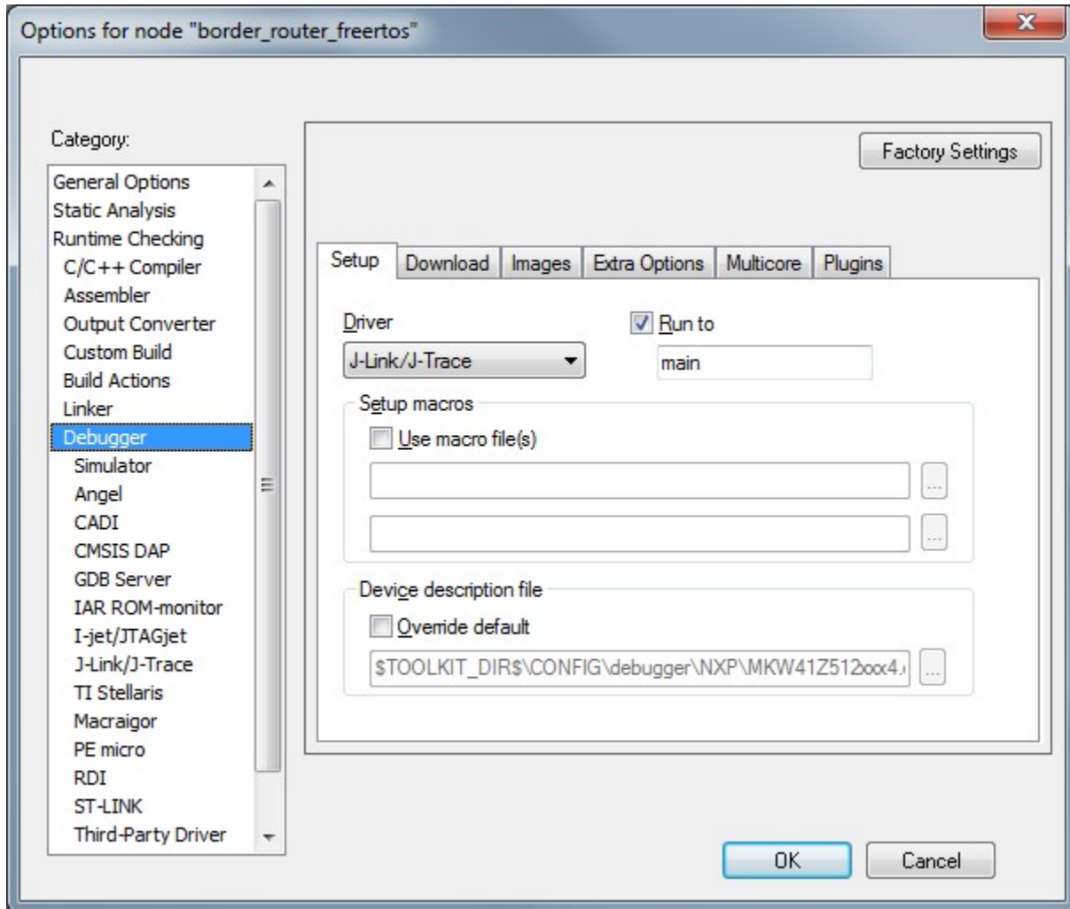
Figure 7. Setting Debugger Options
