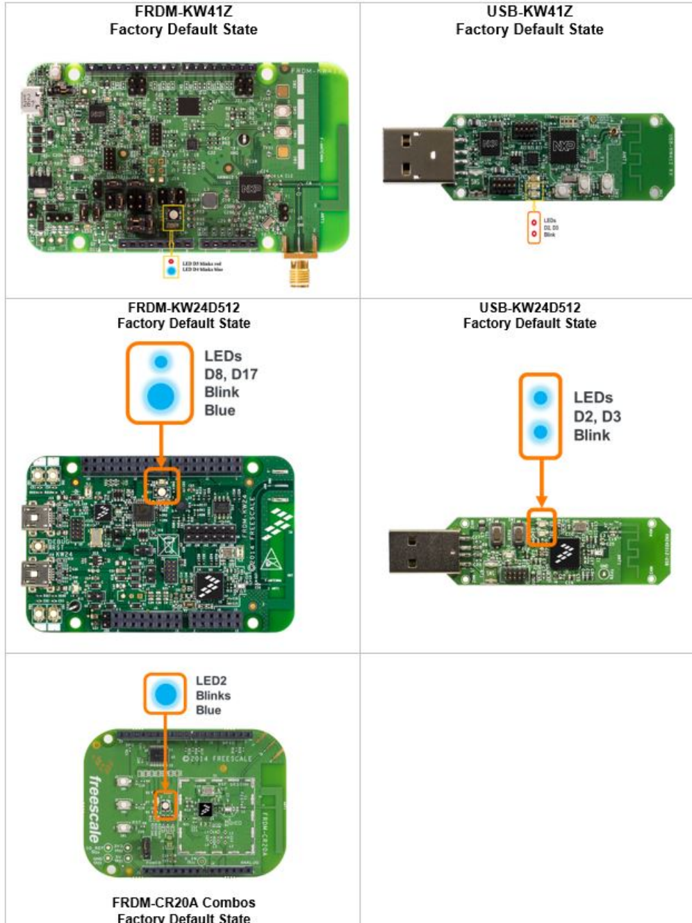
Figure 26. Factory Default State
