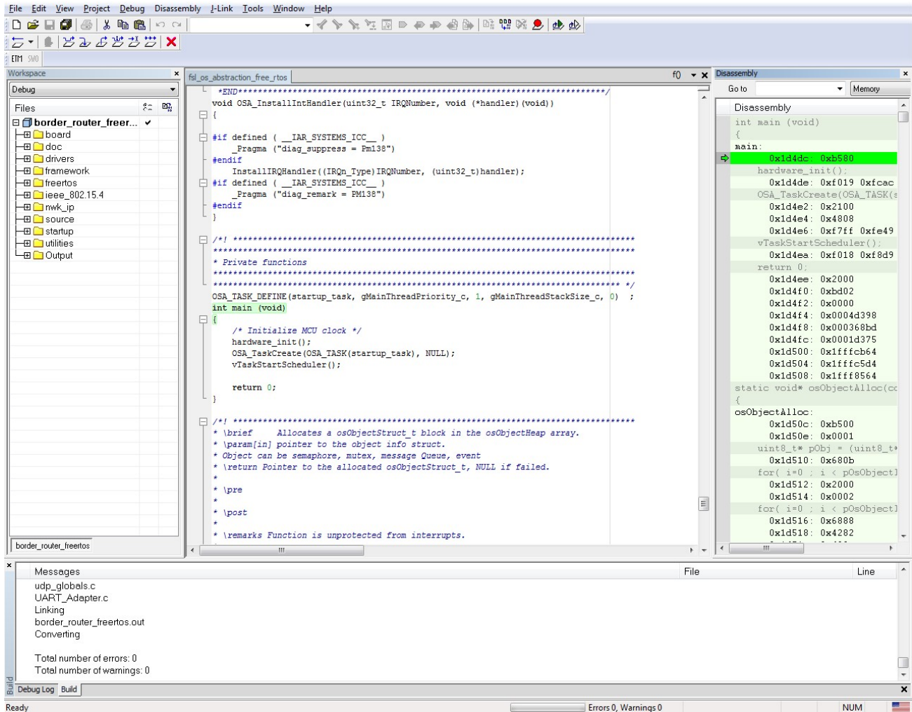
Figure 10. Download and Debug Firmware to Development Board 2
