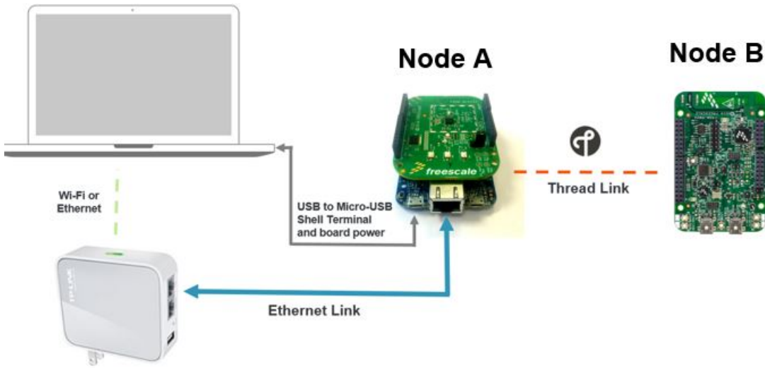
Figure 36. Setup for FRDM-K64F Border Router Application Scenario
