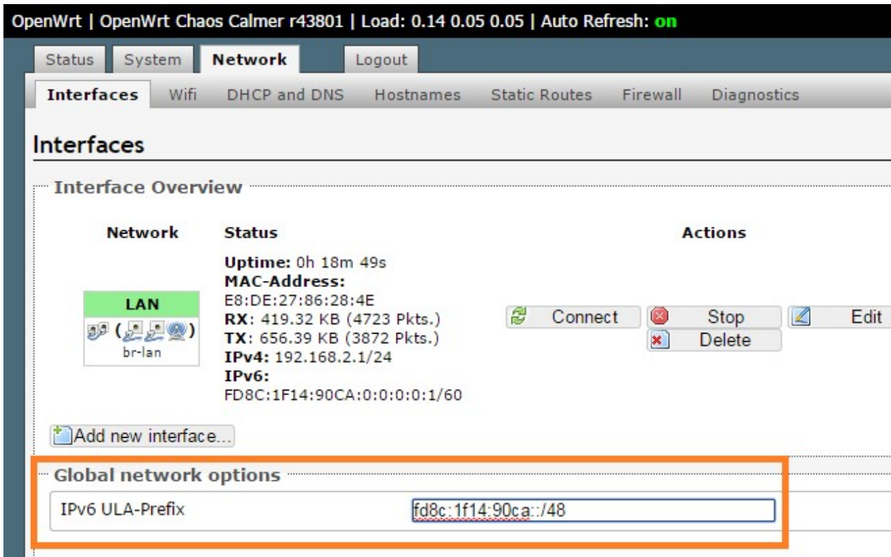
Figure 37. OpenWrt LUCI Web Interface showing IPv6 ULA Prefix Provisioning
