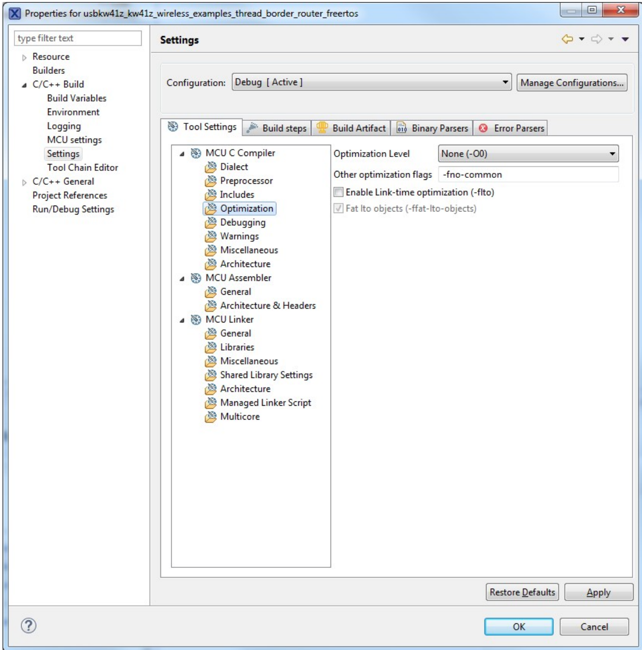
Figure 19. MCUXpresso Debug Configuration Options
