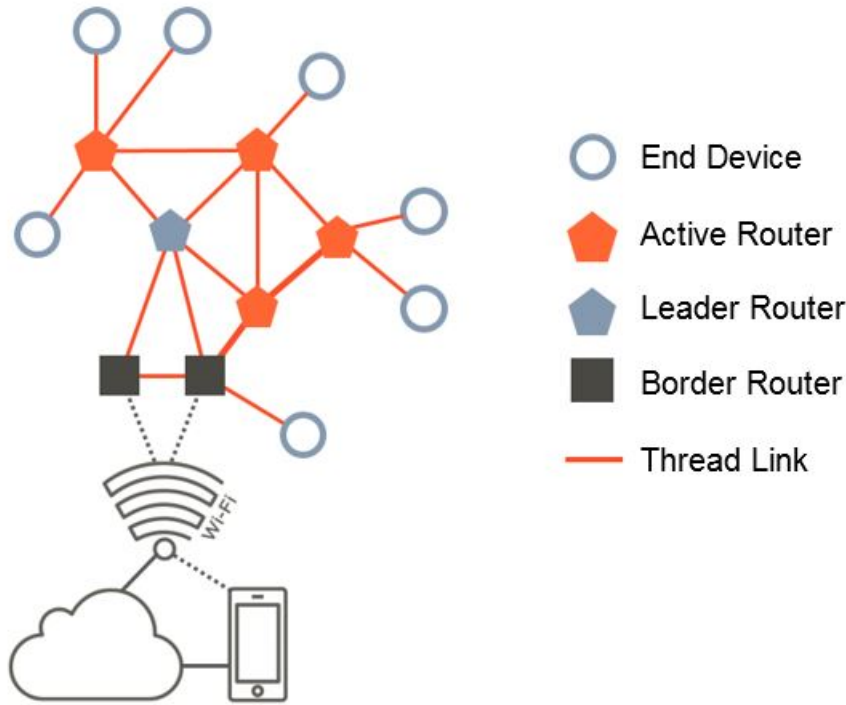
Figure 2. Typical Thread network devices and roles
