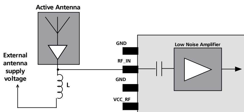
Figure 49: External antenna bias voltage for active antennas
