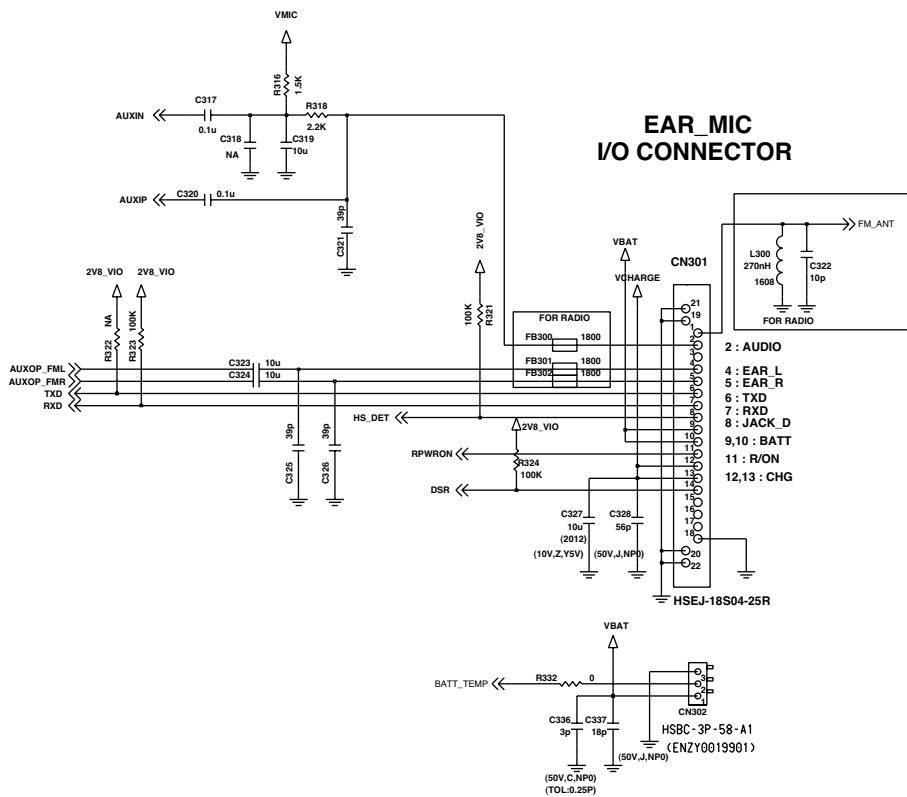
Figure 3-10-5 Headset interface
