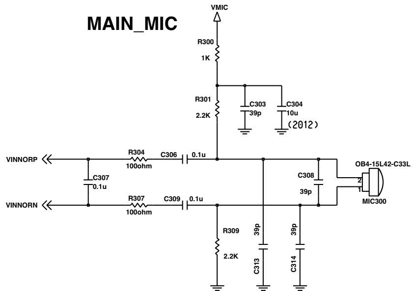
Figure 3-10-4 Main Microphone interface
