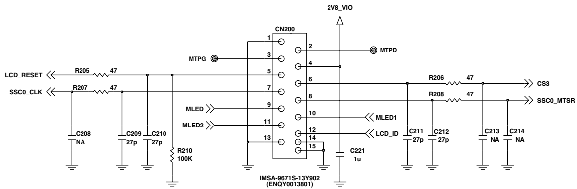
Figure 3-5-1. LCD Interface
