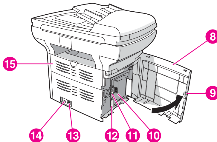
Product hardware components (2 of 2)
