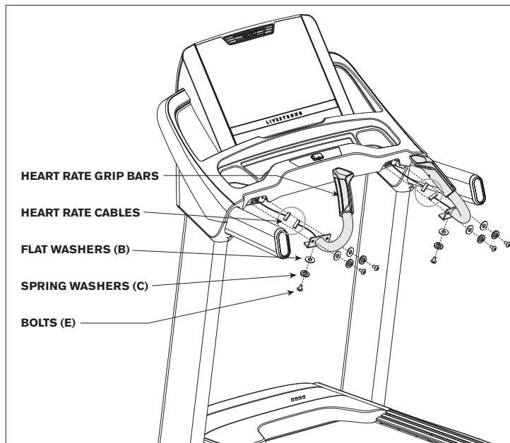
FLAT WASHER (B) 8 mm Qty: 6
