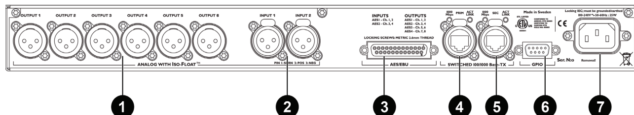
Figure 7-1: Back Panel Interface (LM 26)
