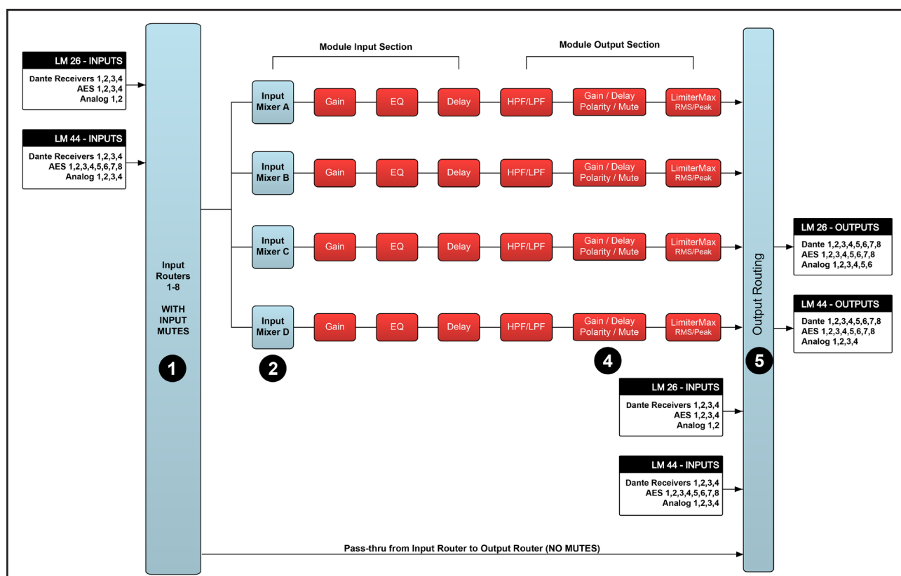
Figure 5-2: LM Series Signal Flow (Mesa Mode)
