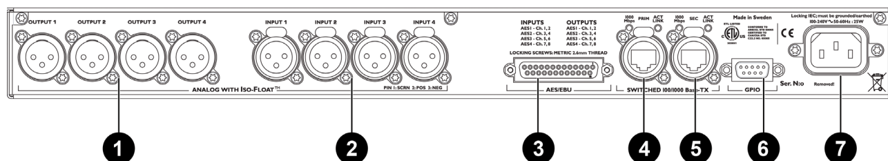
Figure 4-3: LM 44 Back Panel Layout
