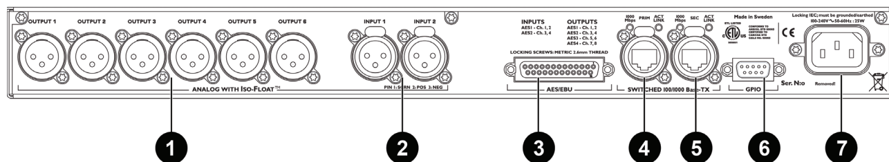
Figure 4-2: LM 26 Back Panel Layout
