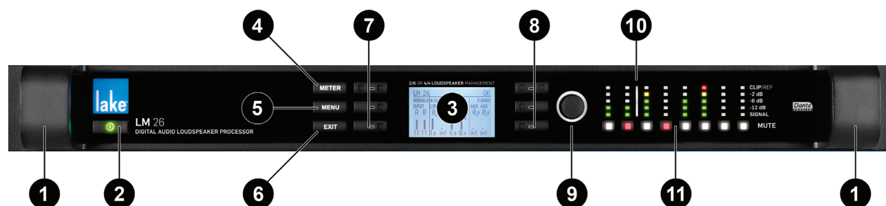
Figure 6-1: Front Panel Interface
