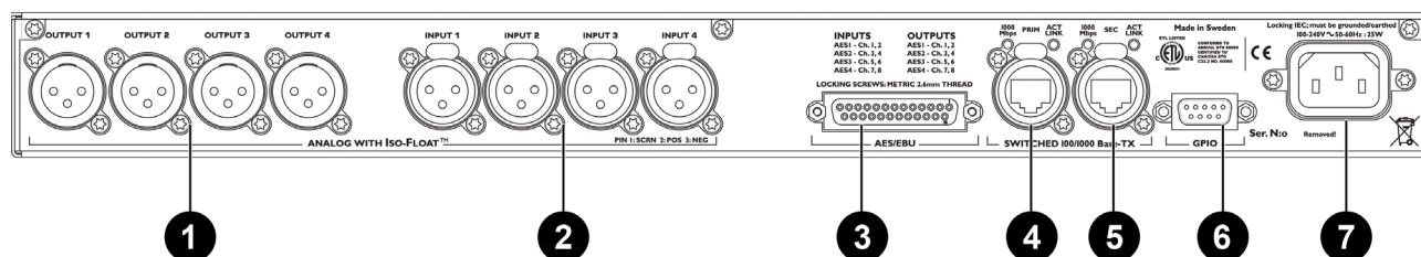
Figure 7-2: Back Panel Interface (LM 44)
