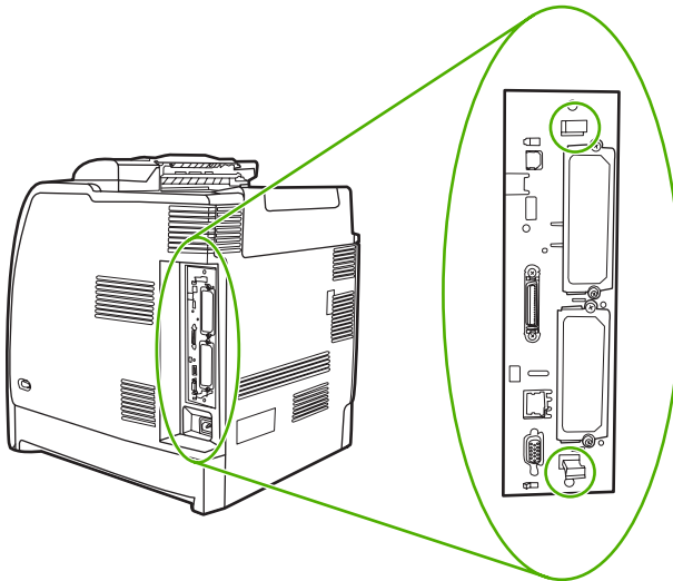
Figure 6-12 Formatter (1 of 2)
