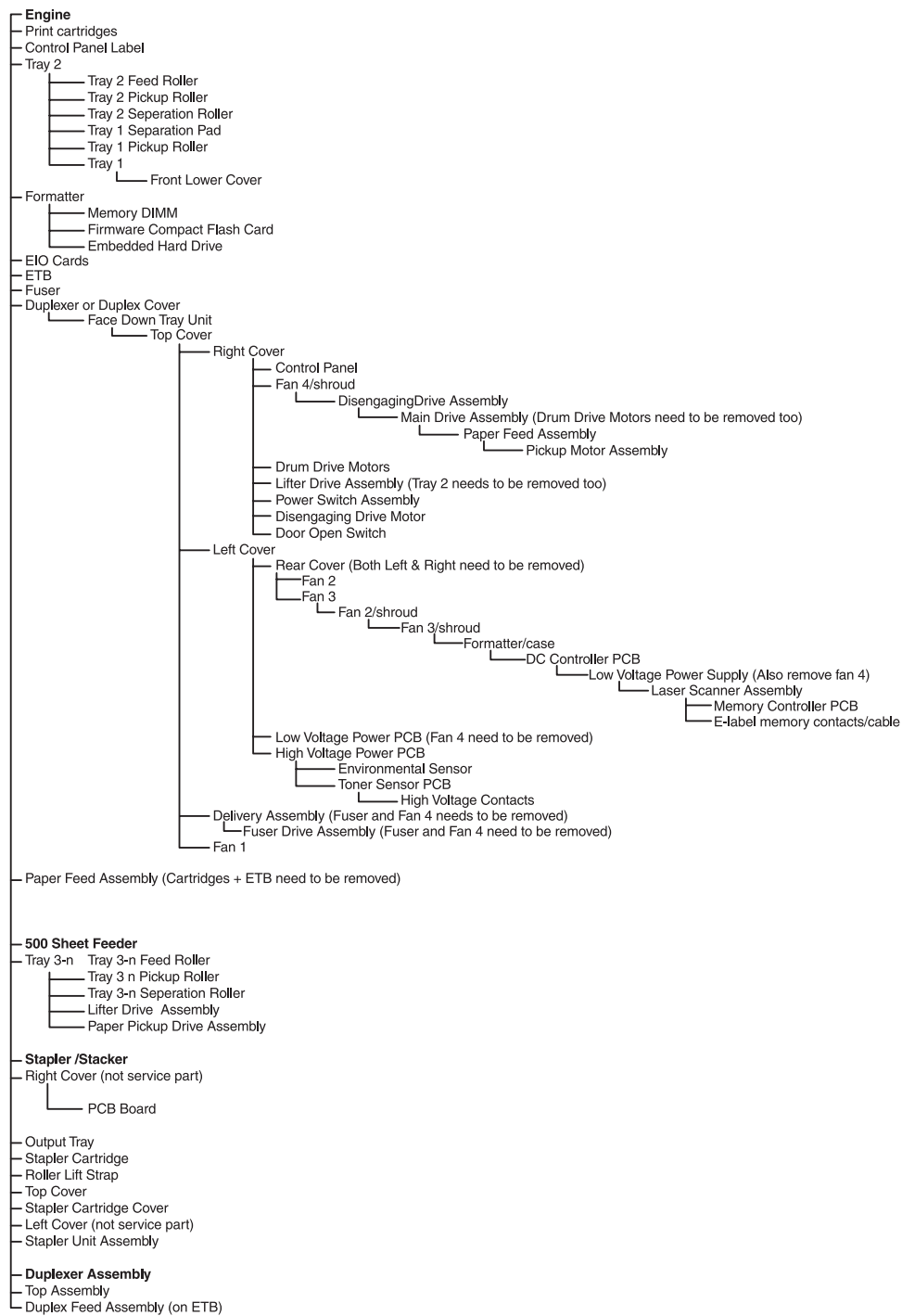
Figure 6-2 Parts-removal tree
