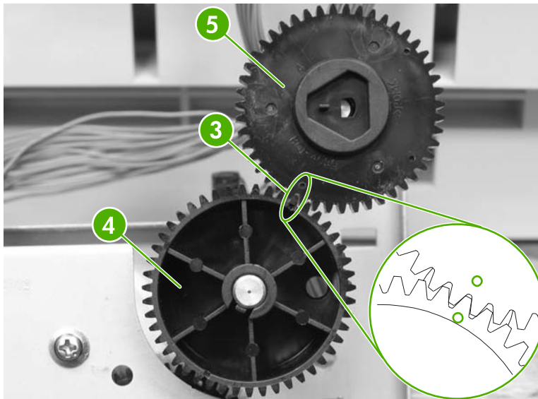
Figure 6-67 Reinstall the main drive assembly (4 of 16)
