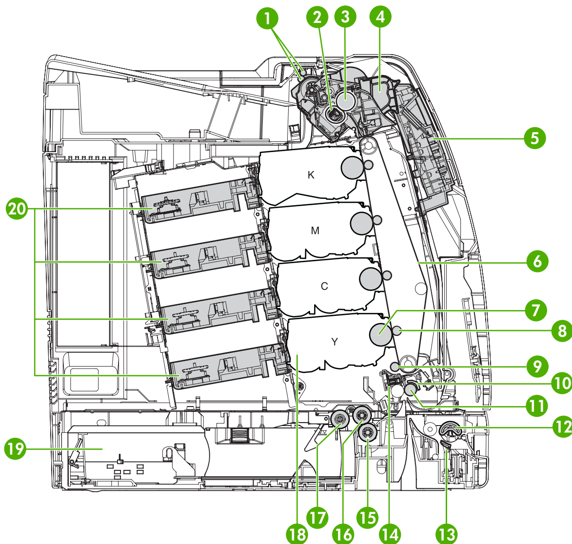
Figure 5-3 Internal components
