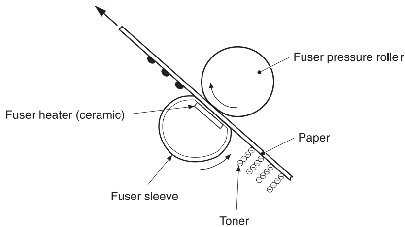
Figure 5-25 Fusing
