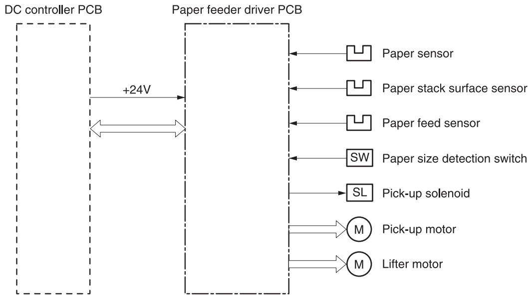
Figure 5-50 Paper feeder driver PCB
