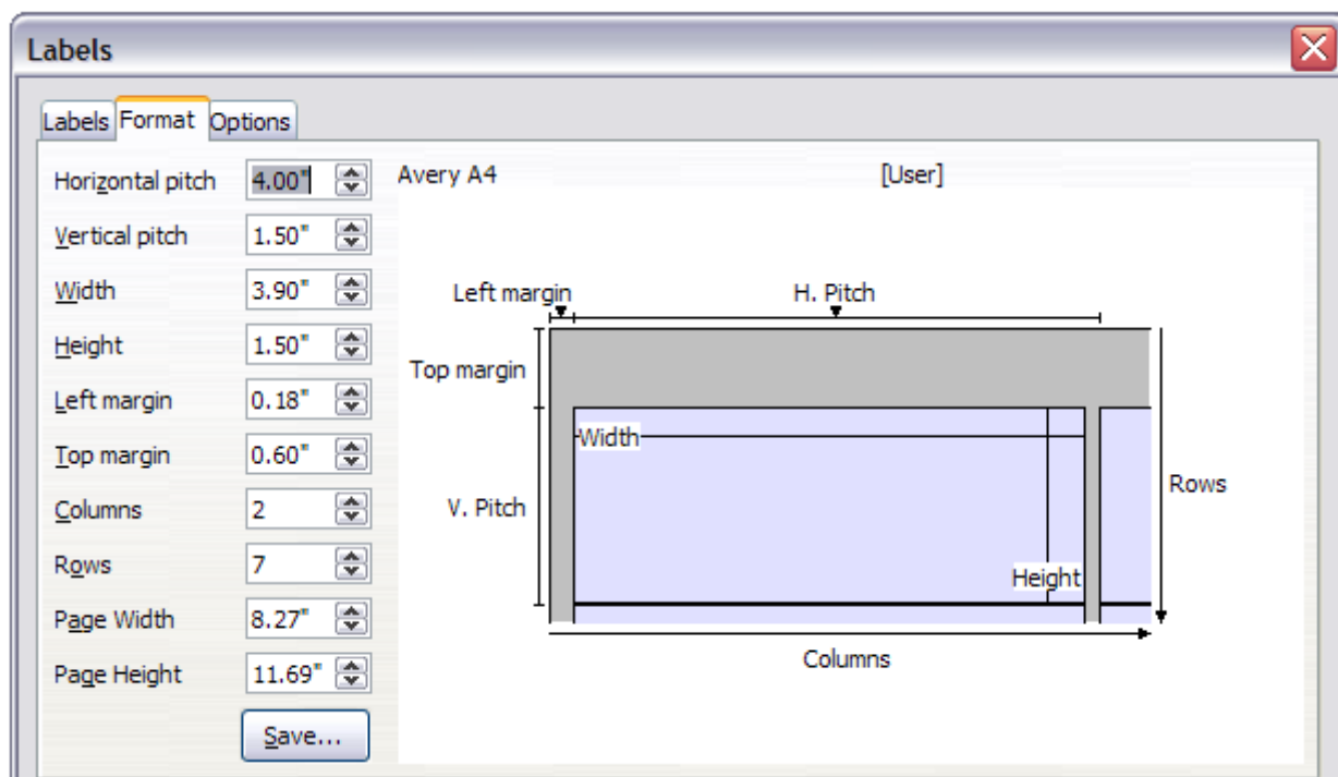
Figure 327: User label default settings
