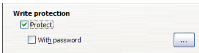
Figure 139: Write-protecting sections
