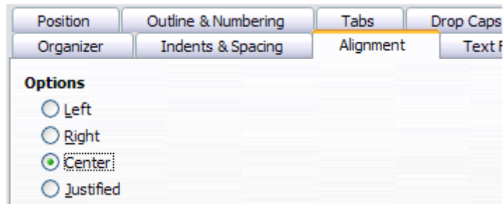
Figure 209: Center Heading 1
