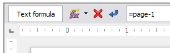
Figure 161: Formula bar
