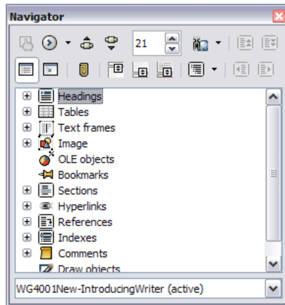
Figure 24: The Navigator
