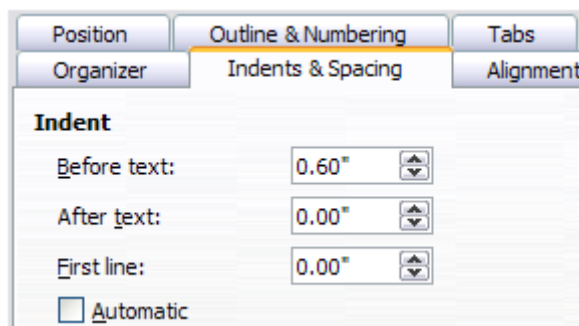
Figure 211: Set indentation
