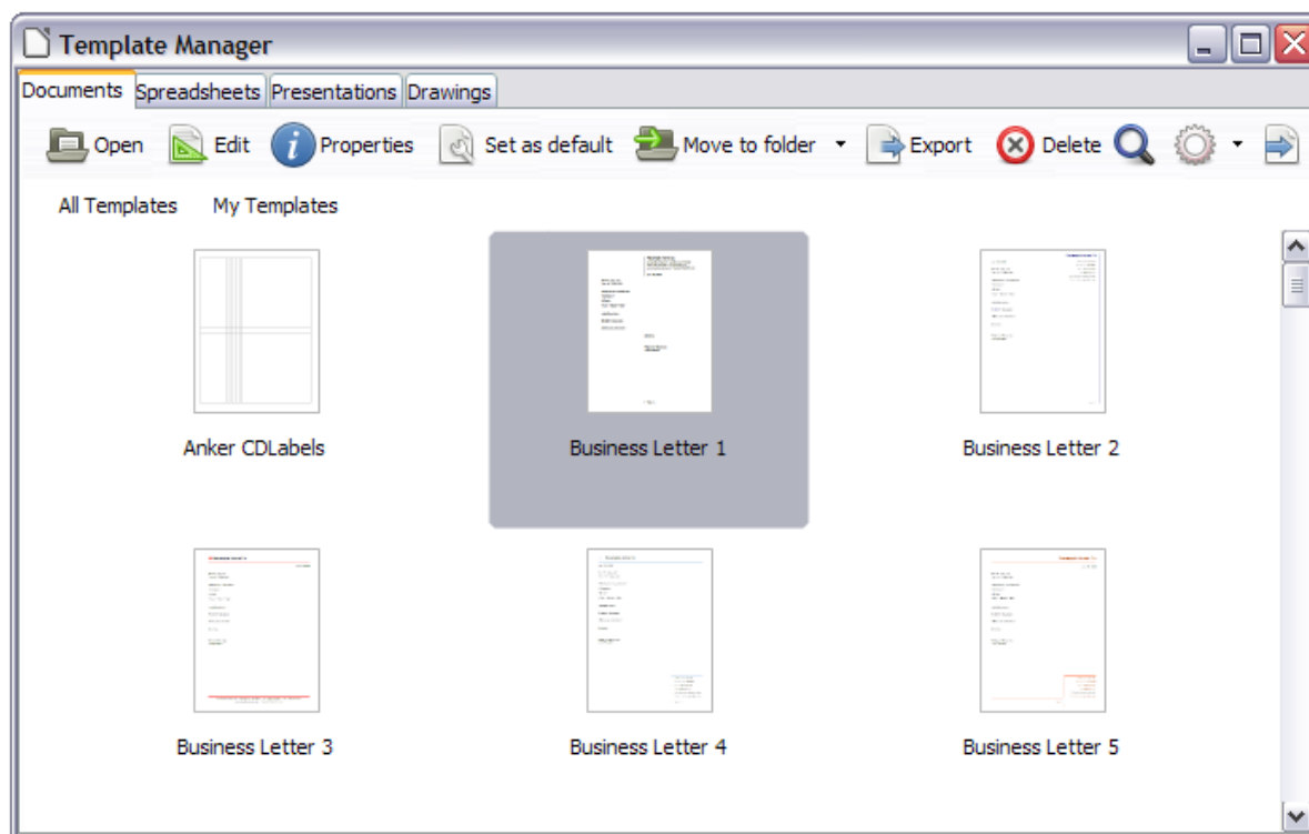
Figure 304: Template Manager
