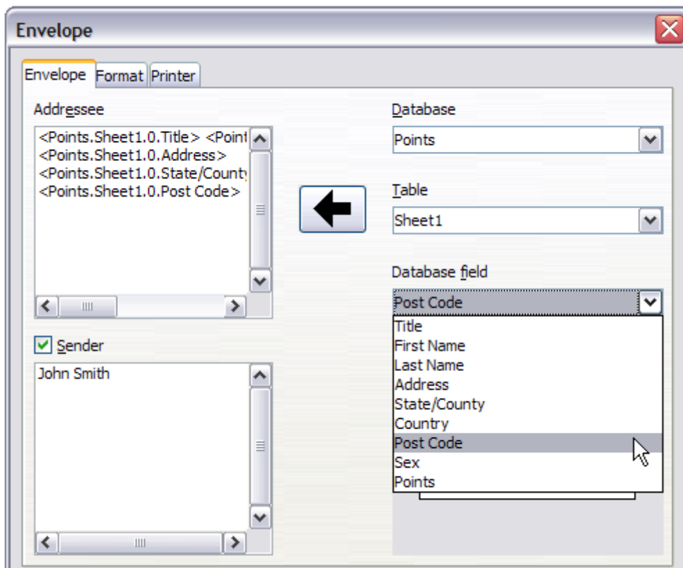
Figure 333: Choosing addressee and sender information for envelopes
