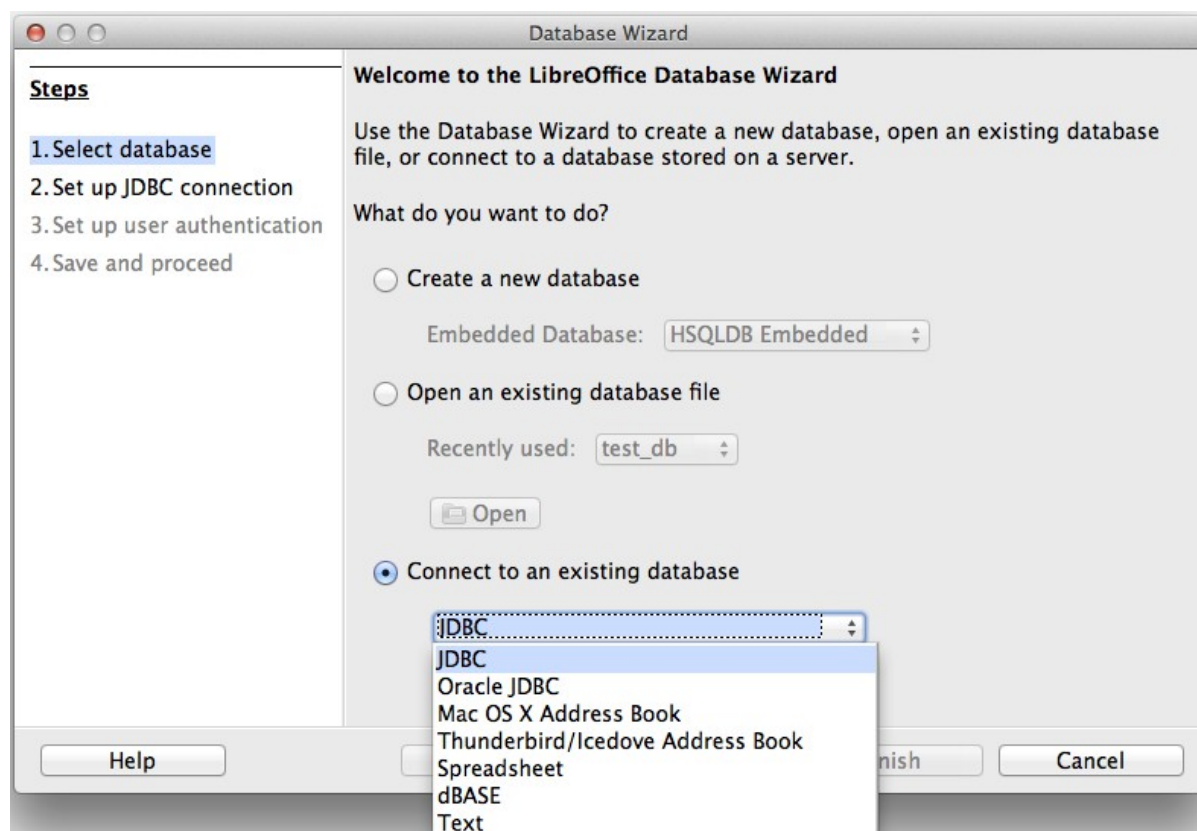
Figure 445: Using the Database Wizard to connect to an existing database
