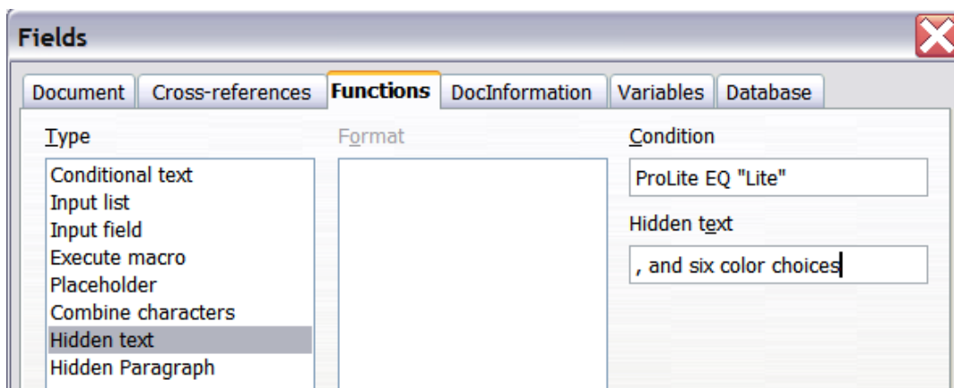
Figure 421: Creating a condition for hidden text
