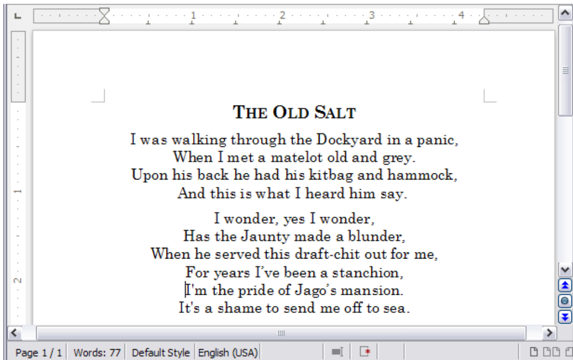
Figure 216: Sample poem
