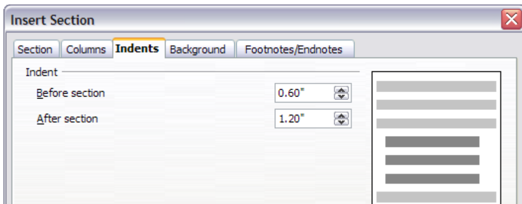
Figure 142: Indenting sections
