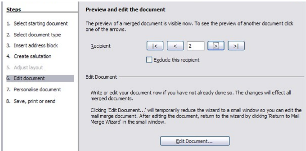
Figure 344: Edit document
