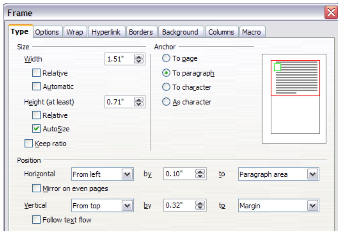
Figure 127: Frame dialog
