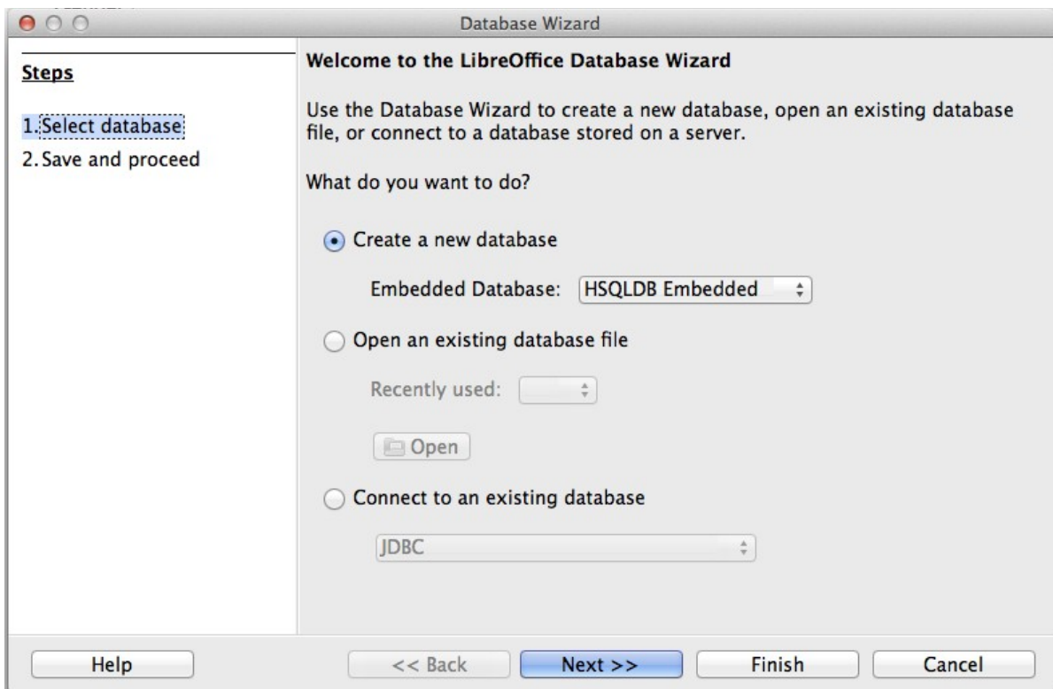
Figure 441: Database Wizard
