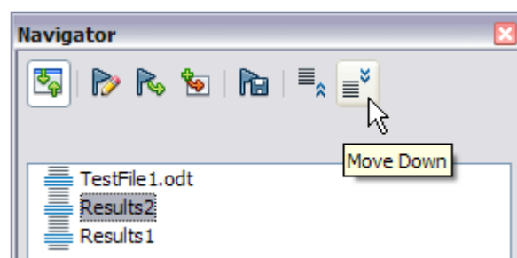
Figure 386: Moving subdocuments
