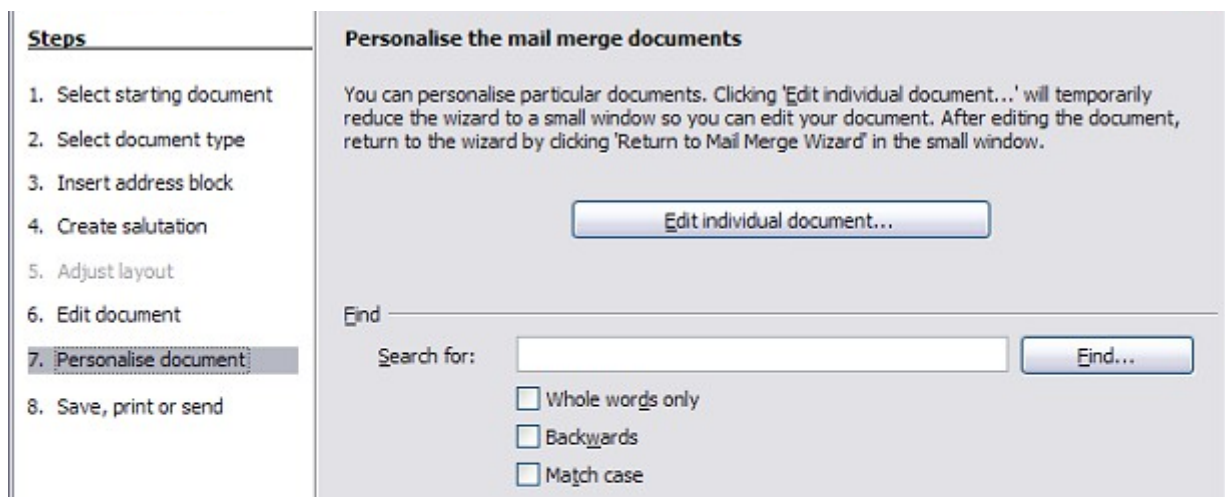
Figure 347: Personalize document
