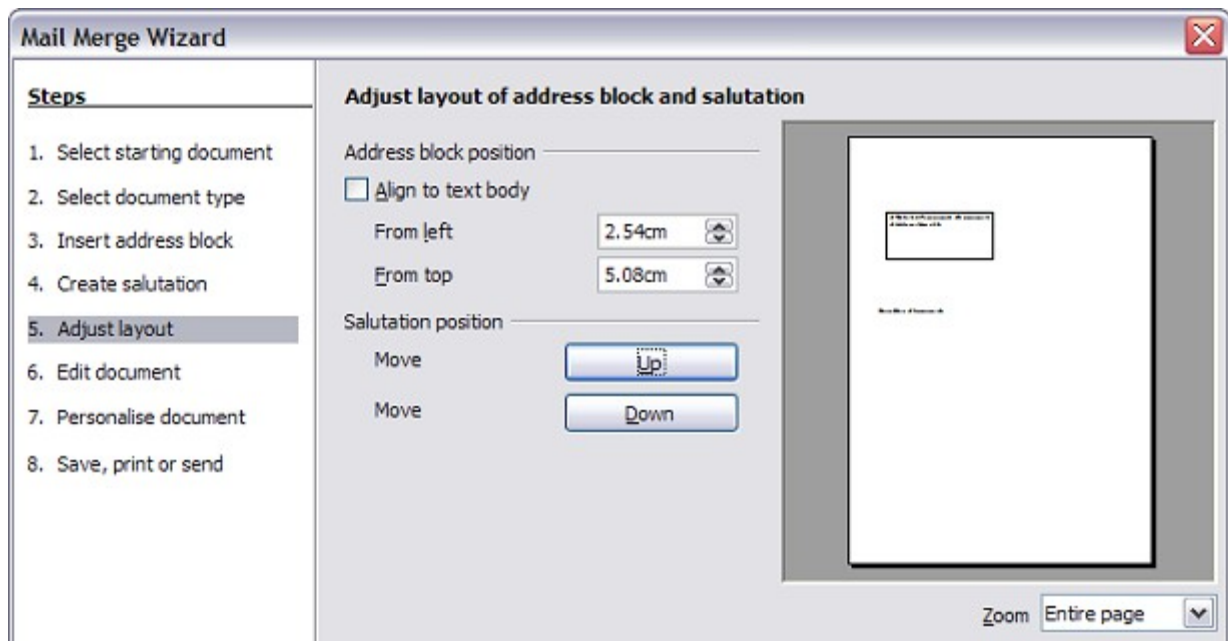
Figure 343: Adjust layout
