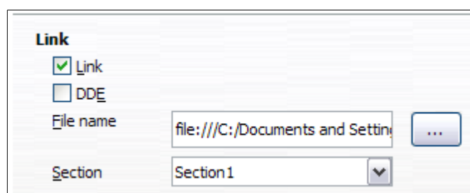
Figure 138: Linking sections
