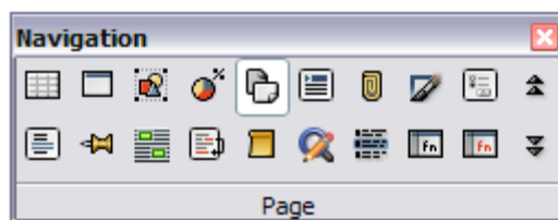
Figure 25: Navigation toolbar
