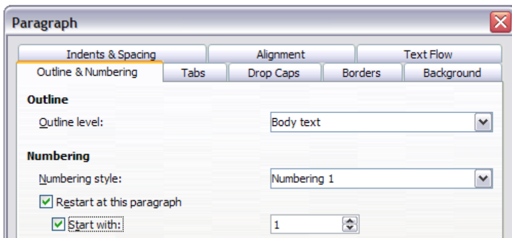
Figure 205: Restarting numbering
