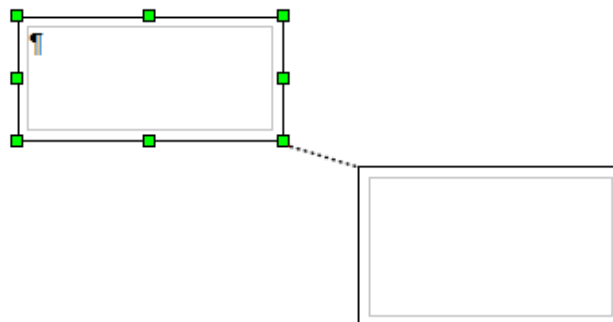
Figure 129: Linked frames
