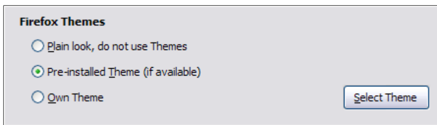
Figure 40: Personalization options
