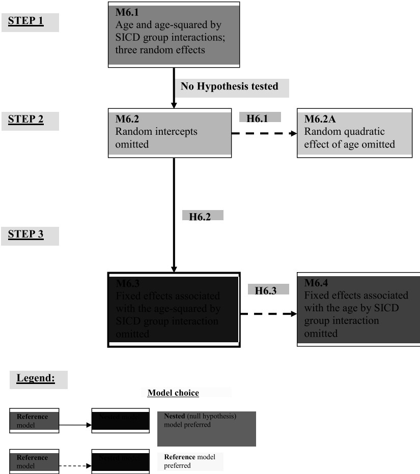
FIGURE 6.3: Model selection and related hypotheses for the analysis of the Autism data.
