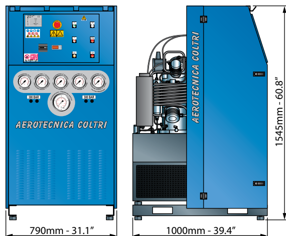
MCH-22-30-36 OPEN
