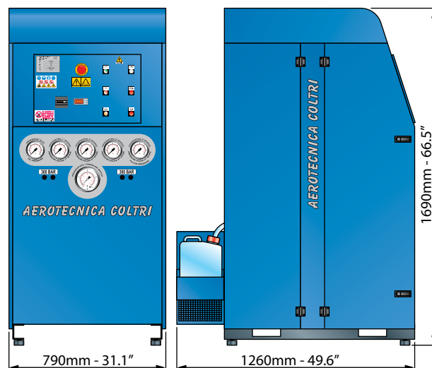
MCH-22-30-36 SILENT
