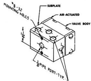
3/8" & 1/2" SUBPLATE DIMENSIONS
