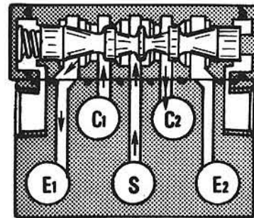
RIGHT CYLINDER PORT NORMALLY OPEN TO SUPPLY
