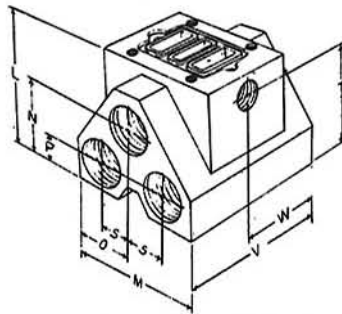
3/8" & 1/2" SUBPLATE DIMENSIONS
