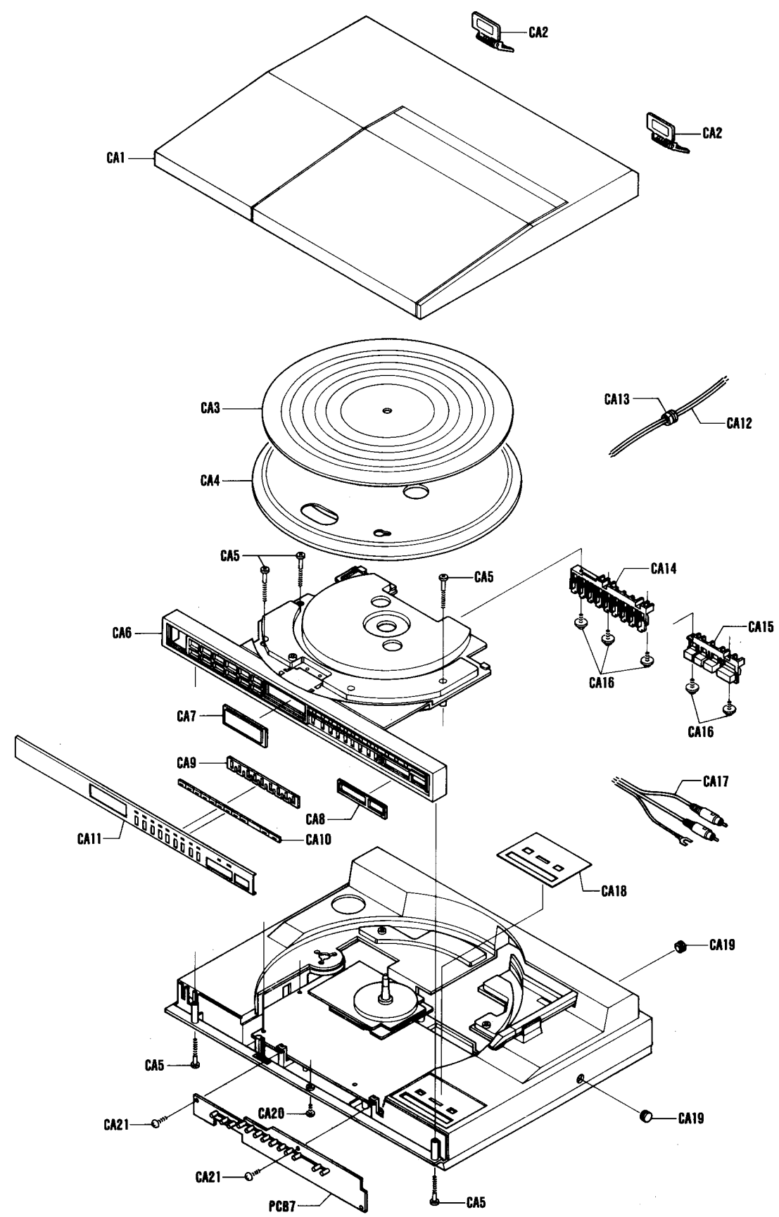
CABINET & TURNTABLE EXPLODED VIEW (1)
