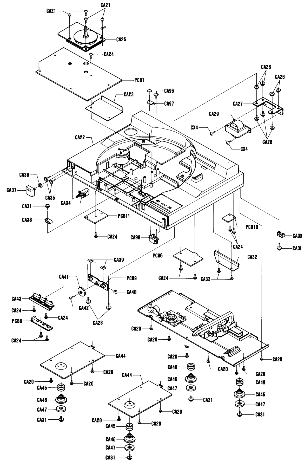
CABINET & TURNTABLE EXPLODED VIEW (2)
