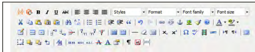
Editor Toolbar
