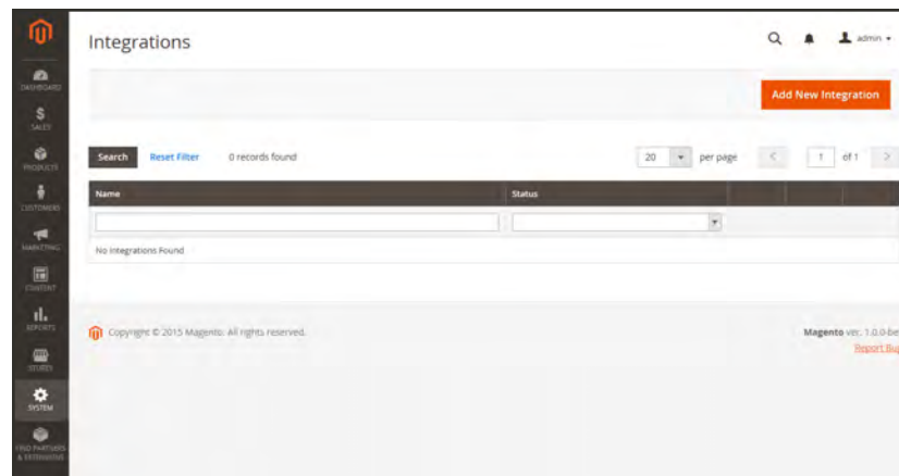
Integrations
