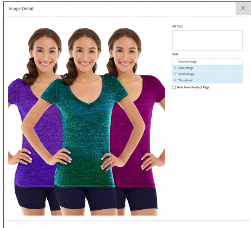
Image Detail
