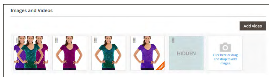
Hidden Image
