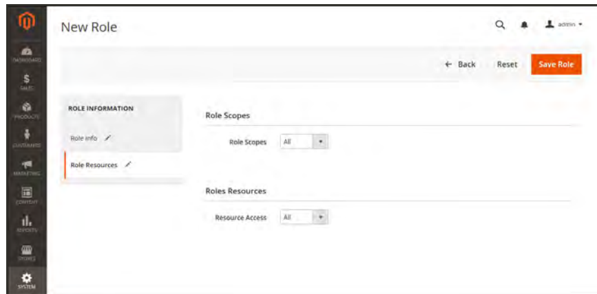
Role Scopes
