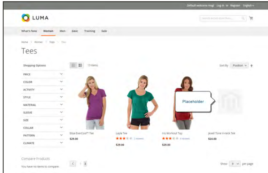
Image Placeholder
