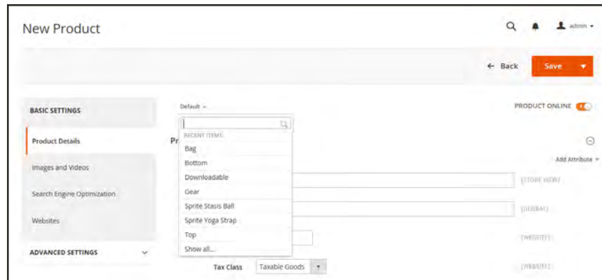
Choose Template
