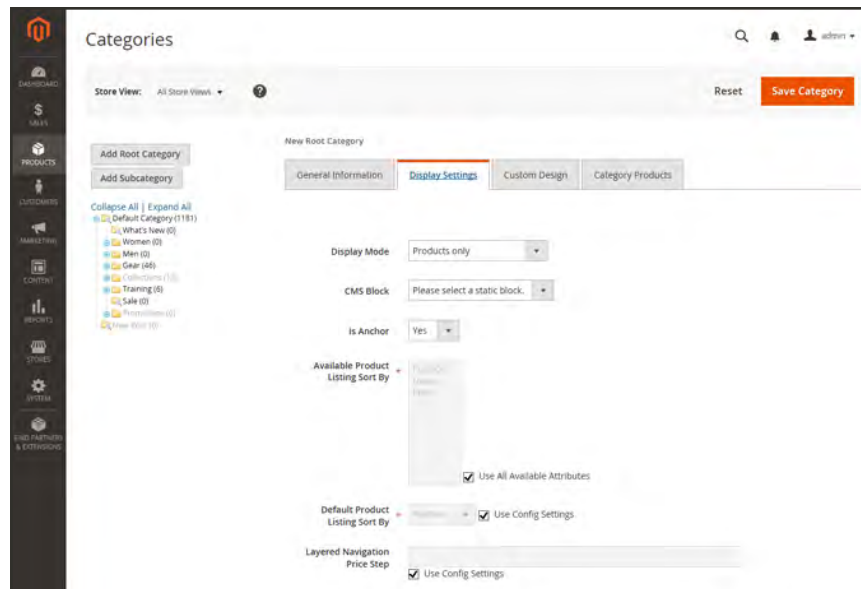
Display Settings
