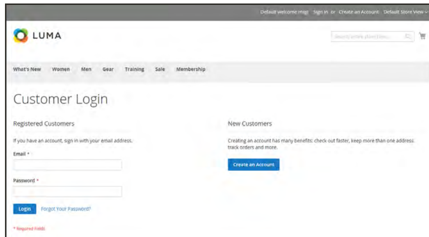
Customer Login
