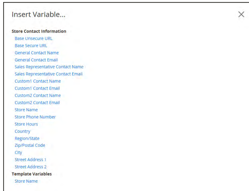
Insert Variable
