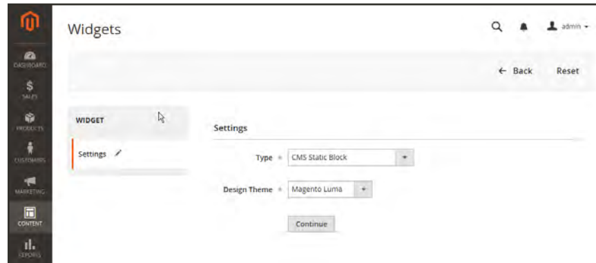
Settings
