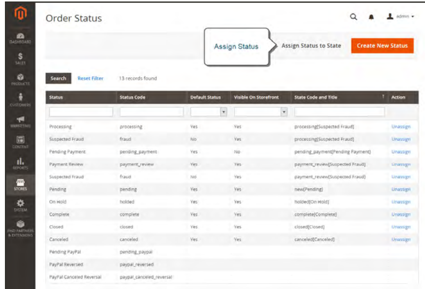
Assign Status
