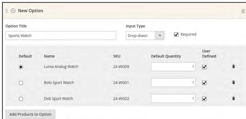
Option Items
