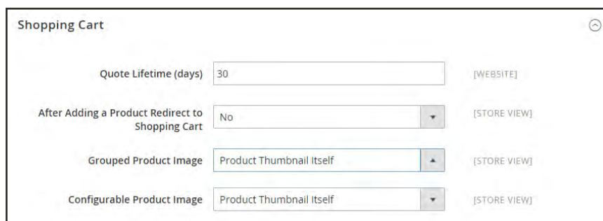
Shopping Cart
