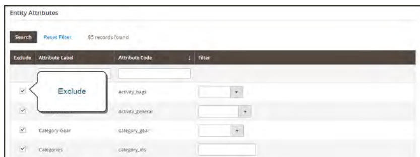
Exclude Attributes
