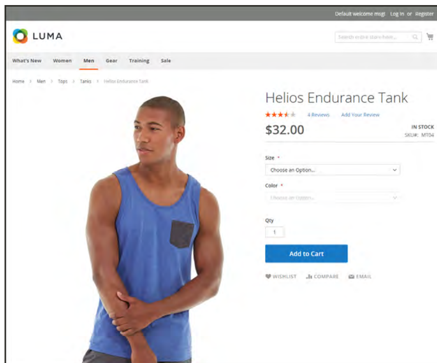
Configurable Product
