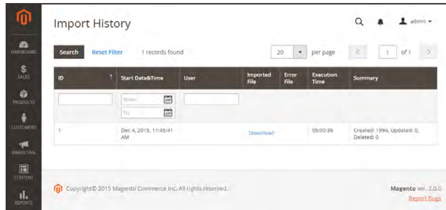
Import History
