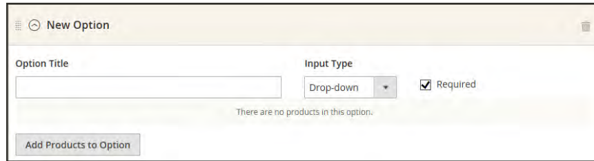
New Option
