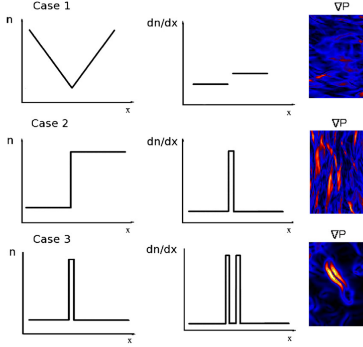
Figure 3: Schematic example of three possible scenarios for enhancements in a generic image “n,” where “n” could be |\vec{P}| , RM, or \rho/N/EM (density, column density, emission measure). Case one (top row) shows an example of a Hölder continuous function that is not differentiable at the origin (applicable to all turbulent fields). Case two (middle row) shows an example of a jump resulting from strong turbulent fluctuations along the LOS or weak shocks. Case three (bottom row) shows a delta function profile resulting from interactions of strong shocks. In this case, the derivative gives a double jump profile which produces morphology that is distinctly different from the previous cases. In all cases we show examples from |\vec{P}| simulations. Figure taken from Burkhart (2012).
