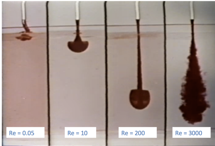
Figure 4: Flows at varying Reynolds number Re . In each panel, a fluid that has been dyed red is injected from the top into the clear fluid on the bottom. The fluids are glycerin-water mixture, for which the viscosity can be changed by altering the glycerin to water ratio. By changing the viscosity and the injection speed, it is possible to alter the Reynolds number of the injected flow. The frames show how the flow develops as the Reynolds number is varied. This image is a still from the National Committee for Fluid Mechanics Film series (Taylor, 1964), which, once you get past the distinctly 1960s production values, are a wonderful resource for everything related to fluids.
