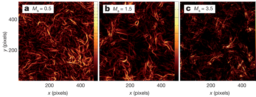
Figure 2: |\vec{\nabla}\vec{P}| derived from propagation of linear radio polarization through three different isothermal simulations of magnetized turbulence. Figure taken from Gaensler (2011).
