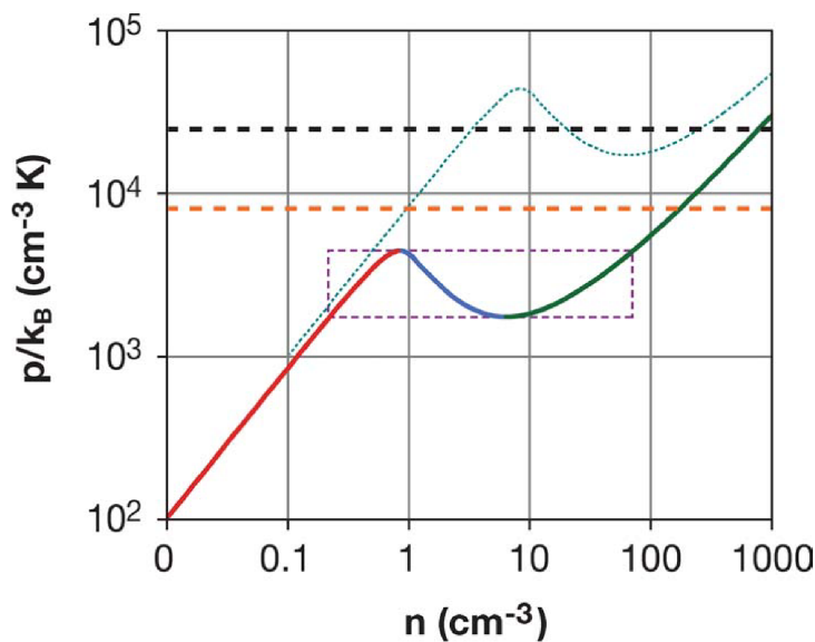
Figure 6: The Two-Phase Medium thermal pressure versus density curve is shown in the red-blue-green curve. The red segment is the thermally stable warm component, the green the corresponding stable cold component, and the blue the thermally unstable regime. The black dashed line is the total midplane pressure, the orange dashed line represents the magnetic pressure, the dashed aqua line shows how the p(n) curve shifts when the heating rate is raised by a factor of 10, and the dashed purple rectangle outlines the regime of essentially zero bulk modulus. Figure taken from Cox (2005).
