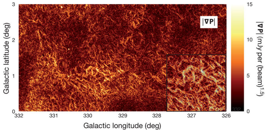
Figure 1: |\vec{\nabla}\vec{P}| for an 18-deg 2 region of the Southern Galactic Plane Survey which reveals a complex network of tangled filaments. In particular, all regions in which |\vec{\nabla}\vec{P}| is high consists of elongated, narrow structures rather than extended patches. In the inset, the direction of |\vec{\nabla}\vec{P}| is shown for a small subregion of the image, demonstrating that |\vec{\nabla}\vec{P}| changes most rapidly along directions oriented perpendicular to the filaments. Figure taken from Gaensler (2011).
