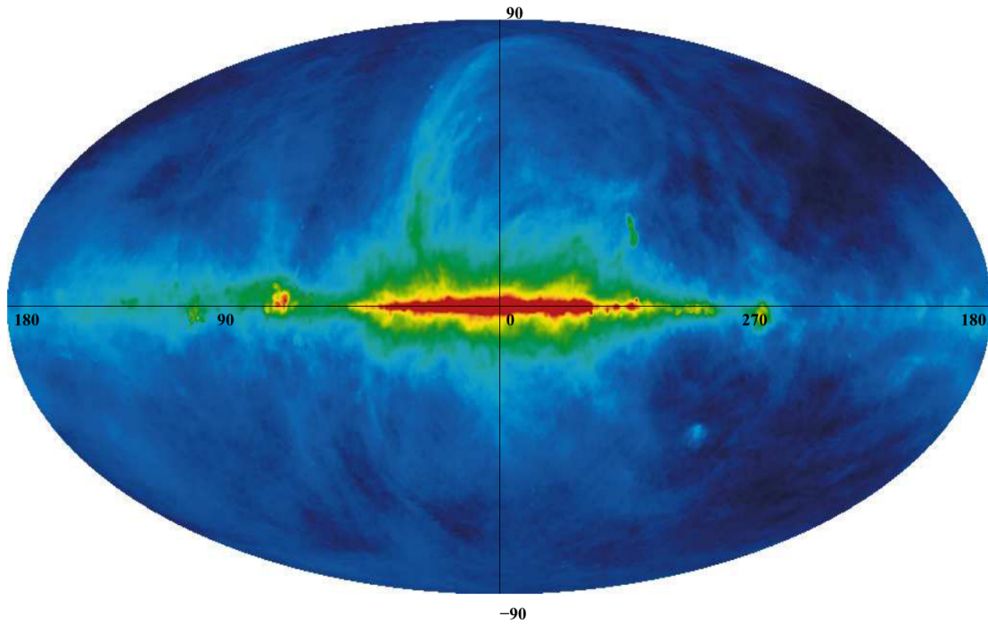
Figure 5: The synchrotron emission at 408 MHz across the entire sky in Galactic coordinates. As expected, the emission is concentrated along the Galactic plane. However, the feature known as Loop I, is clearly arching up from \ell = 55^\circ towards the North Galactic Pole. This Figure is adapted from Haslam et al. (1981). Figure taken from Newton-McGee (2009).
