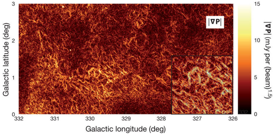
Figure 2: |\vec{\nabla}\vec{P}| for an 18-deg 2 region of the Southern Galactic Plane Survey which reveals a complex network of tangled filaments. In particular, all regions in which |\nabla\vec{P}| is high consists of elongated, narrow structures rather than extended patches. In the inset, the direction of |\nabla\vec{P}| is shown for a small subregion of the image, demonstrating that |\nabla\vec{P}| changes most rapidly along directions oriented perpendicular to the filaments. Figure taken from Gaensler (2011).
