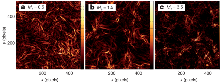
Figure 3: |\vec{\nabla}\vec{P}| derived from propagation of linear radio polarization through three different isothermal simulations of magnetized turbulence. Figure taken from Gaensler (2011).
