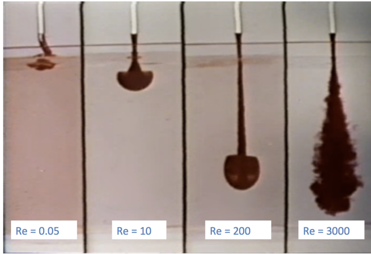
Figure 3: Flows at varying Reynolds number Re . In each panel, a fluid that has been dyed red is injected from the top into the clear fluid on the bottom. The fluids are glycerin-water mixture, for which the viscosity can be changed by altering the glycerin to water ratio. By changing the viscosity and the injection speed, it is possible to alter the Reynolds number of the injected flow. The frames show how the flow develops as the Reynolds number is varied. This image is a still from the National Committee for Fluid Mechanics Film series (Taylor, 1964), which, once you get past the distinctly 1960s production values, are a wonderful resource for everything related to fluids.
