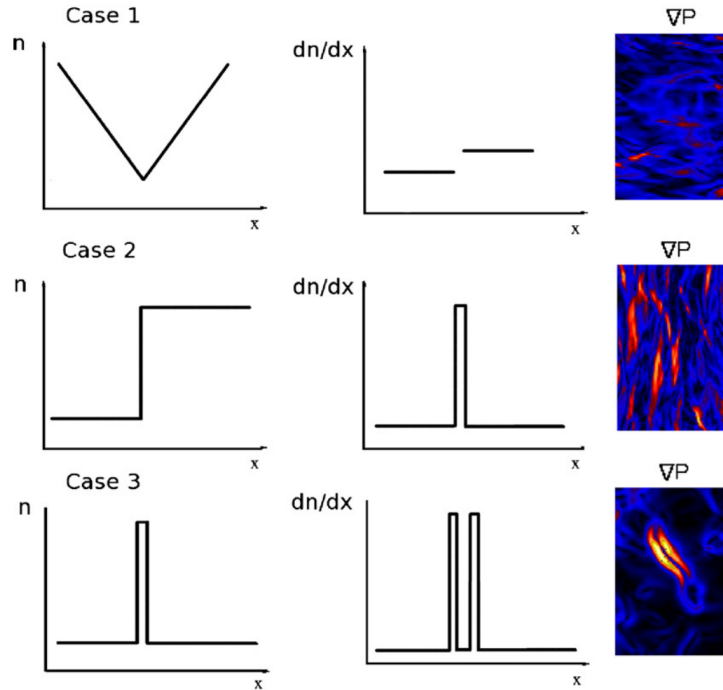
Figure 2: Schematic example of three possible scenarios for enhancements in a generic image “n,” where “n” could be |\vec{P}| , RM, or \rho/N/EM (density, column density, emission measure). Case one (top row) shows an example of a Hölder continuous function that is not differentiable at the origin (applicable to all turbulent fields). Case two (middle row) shows an example of a jump resulting from strong turbulent fluctuations along the LOS or weak shocks. Case three (bottom row) shows a delta function profile resulting from interactions of strong shocks. In this case, the derivative gives a double jump profile which produces morphology that is distinctly different from the previous cases. In all cases we show examples from |\vec{P}| simulations. Figure taken from Burkhart (2012).
