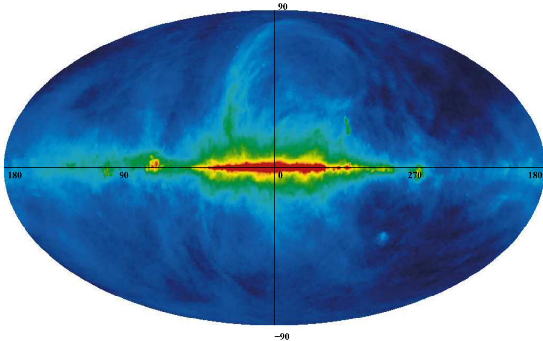
Figure 4: The synchrotron emission at 408 MHz across the entire sky in Galactic coordinates. As expected, the emission is concentrated along the Galactic plane. However, the feature known as Loop I, is clearly arching up from \ell = 55^\circ towards the North Galactic Pole. This Figure is adapted from Haslam et al. (1981). Figure taken from Newton-McGee (2009).
