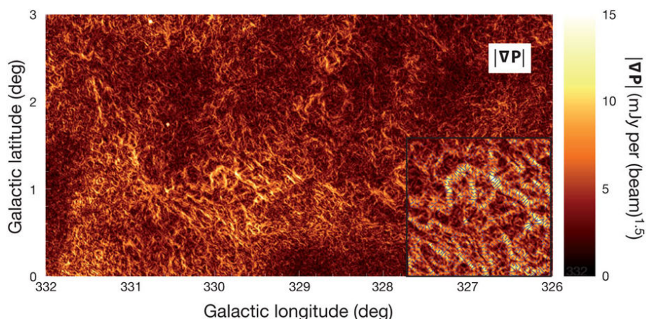
Figure 1: |\nabla P| for an 18-deg 2 region of the Southern Galactic Plane Survey which reveals a complex network of tangled filaments. In particular, all regions in which |\nabla\vec{P}| is high consists of elongated, narrow structures rather than extended patches. In the inset, the direction of |\nabla\vec{P}| is shown for a small subregion of the image, demonstrating that |\nabla\vec{P}| changes most rapidly along directions oriented perpendicular to the filaments. Figure taken from Gaensler (2011).
