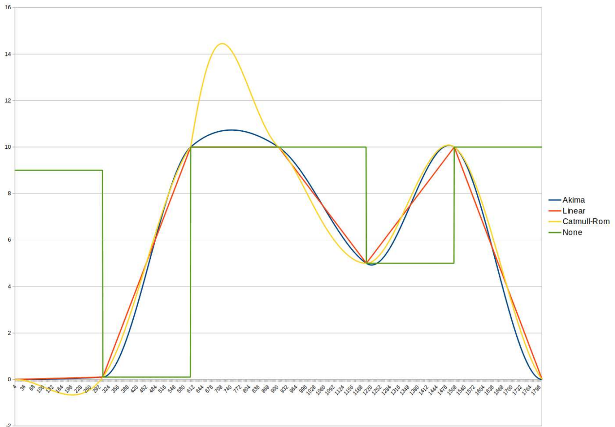
Figure 7.1: Interpolation types
