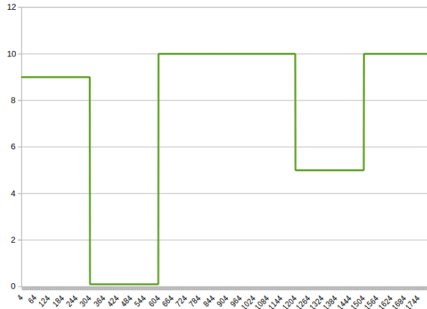
Figure 7.2: Interpolation - None
