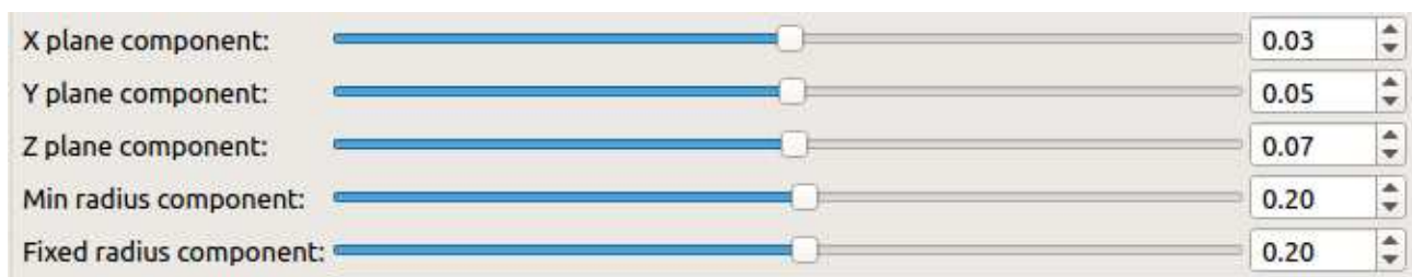
Figure 13.4: Aux.color parameters
