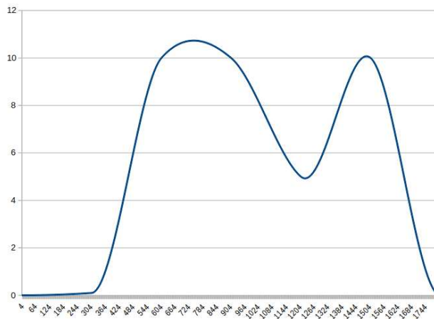
Figure 7.4: Interpolation - Akima
