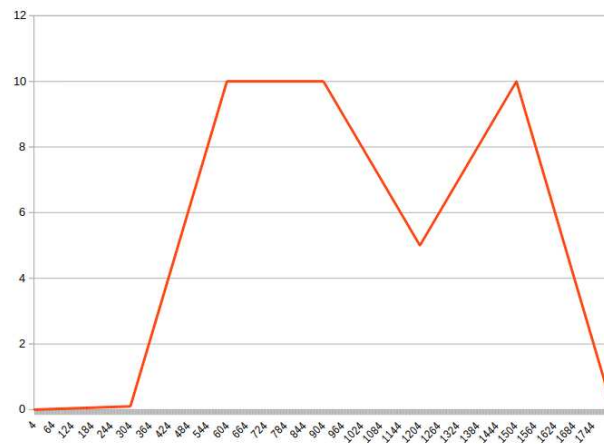
Figure 7.3: Interpolation - Linear
