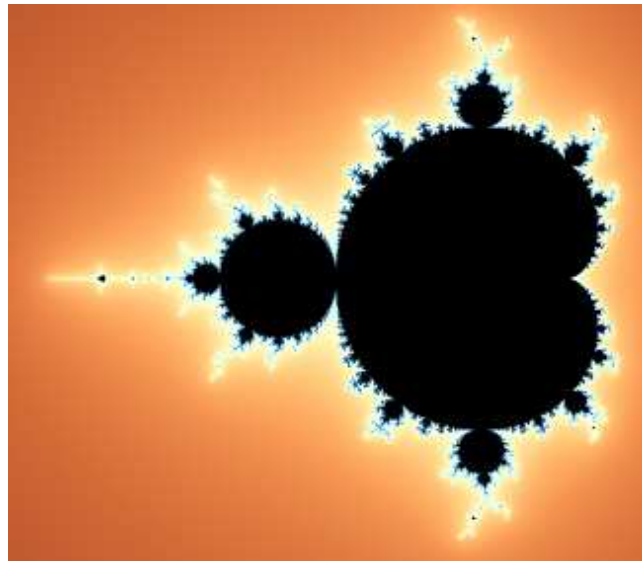
Figure 2.1: Mandelbrot Set
