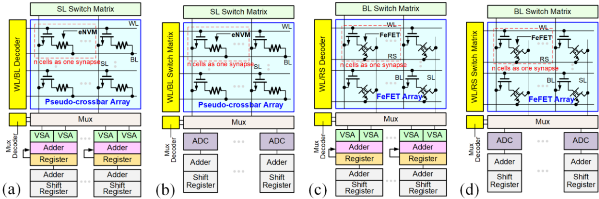
Fig. 7. (a) sequential-read-out and (b) parallel-read-out analog eNVM pseudo-1T1R synaptic arrays; (c) sequential-read-out and (d) parallel-read-out analog FeFET synaptic arrays;
