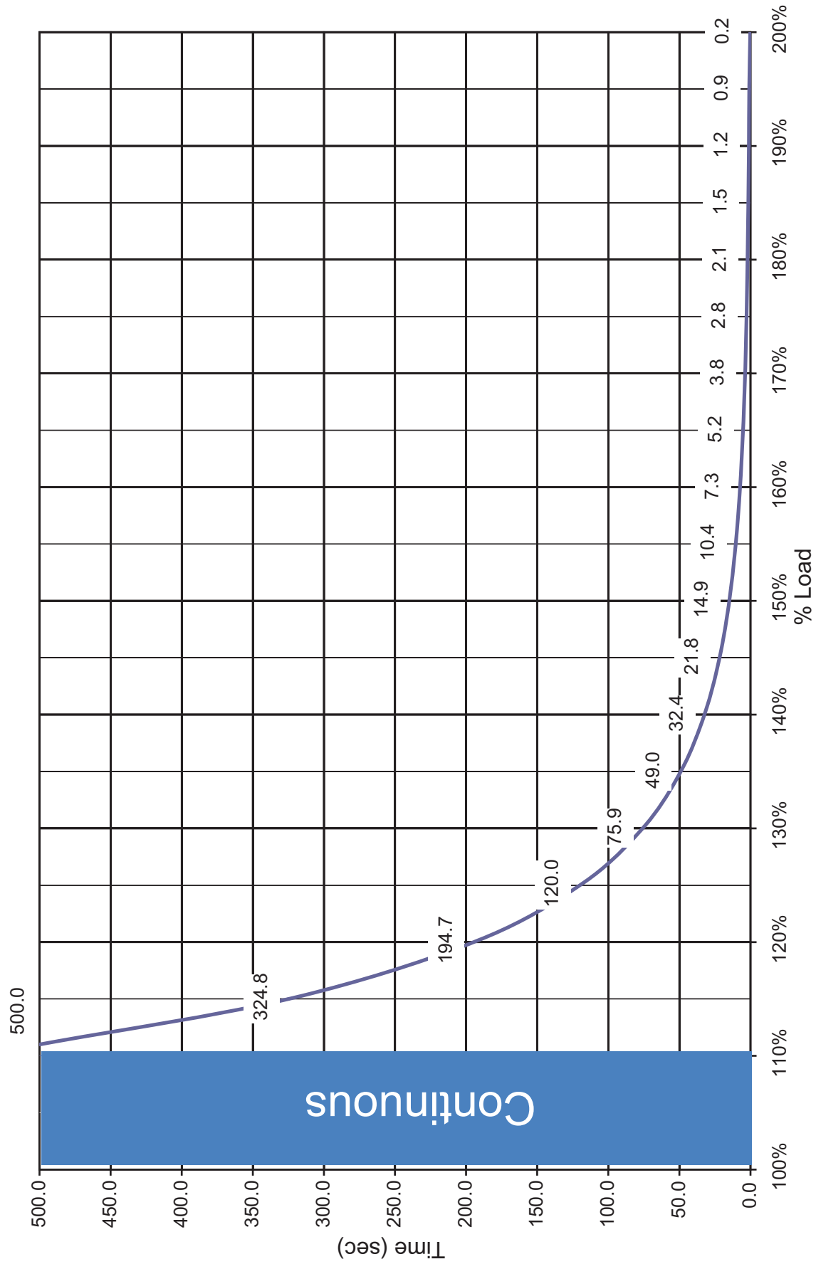
Figure 20 Bypass overload data
