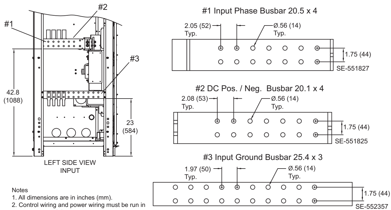
Figure 8 Input and battery terminal detail, 625-800kVA Liebert eXL single-module UPS
