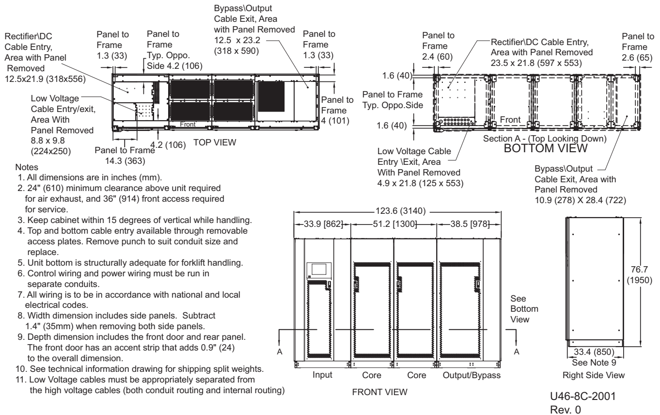
Figure 7 Base drawing, 625-800kVA Liebert eXL single-module UPS
