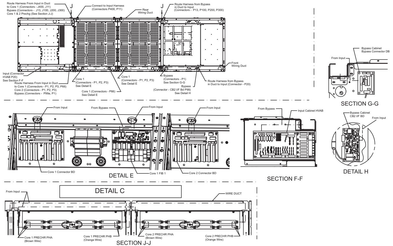
Figure 13 Shipping split, 625-800kVA Liebert eXL single-module UPS, continued
