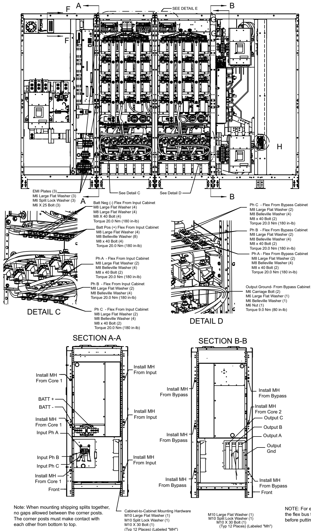
Figure 12 Shipping split, 625-800kVA Liebert eXL single-module UPS
