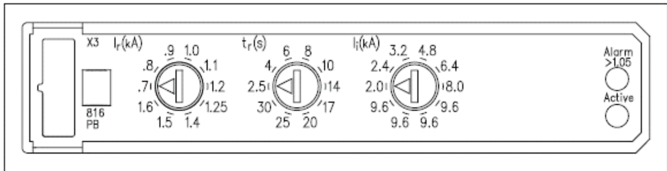
Figure 4 Internal Breaker settings
