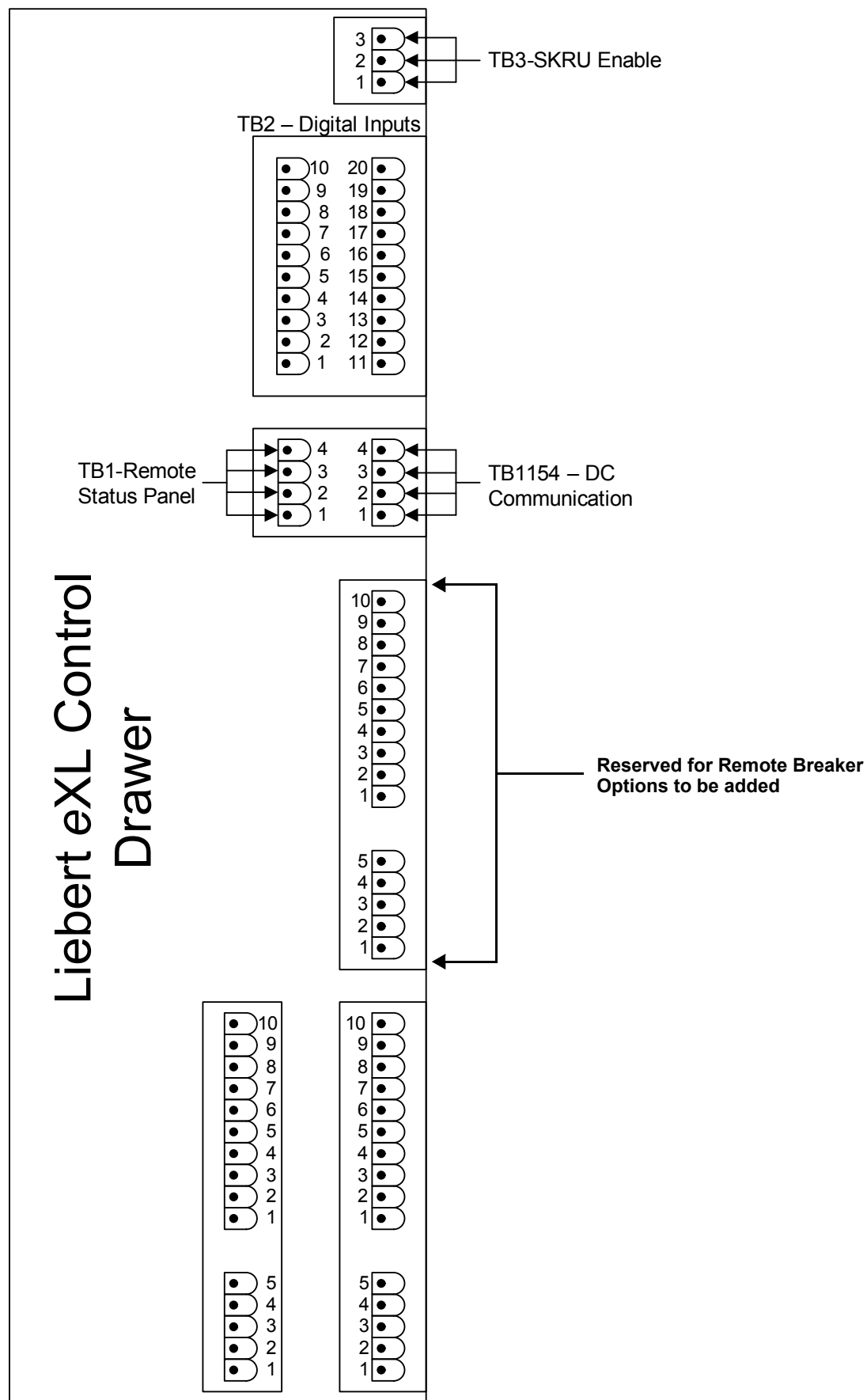
Figure 2 Liebert eXL customer connections
