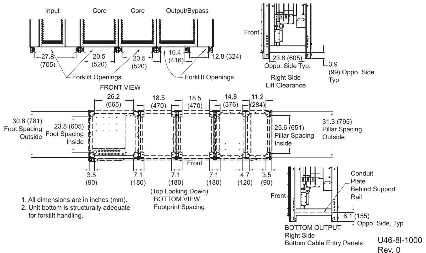
Figure 7 Base drawing, 625-800kVA Liebert eXL single-module UPS
