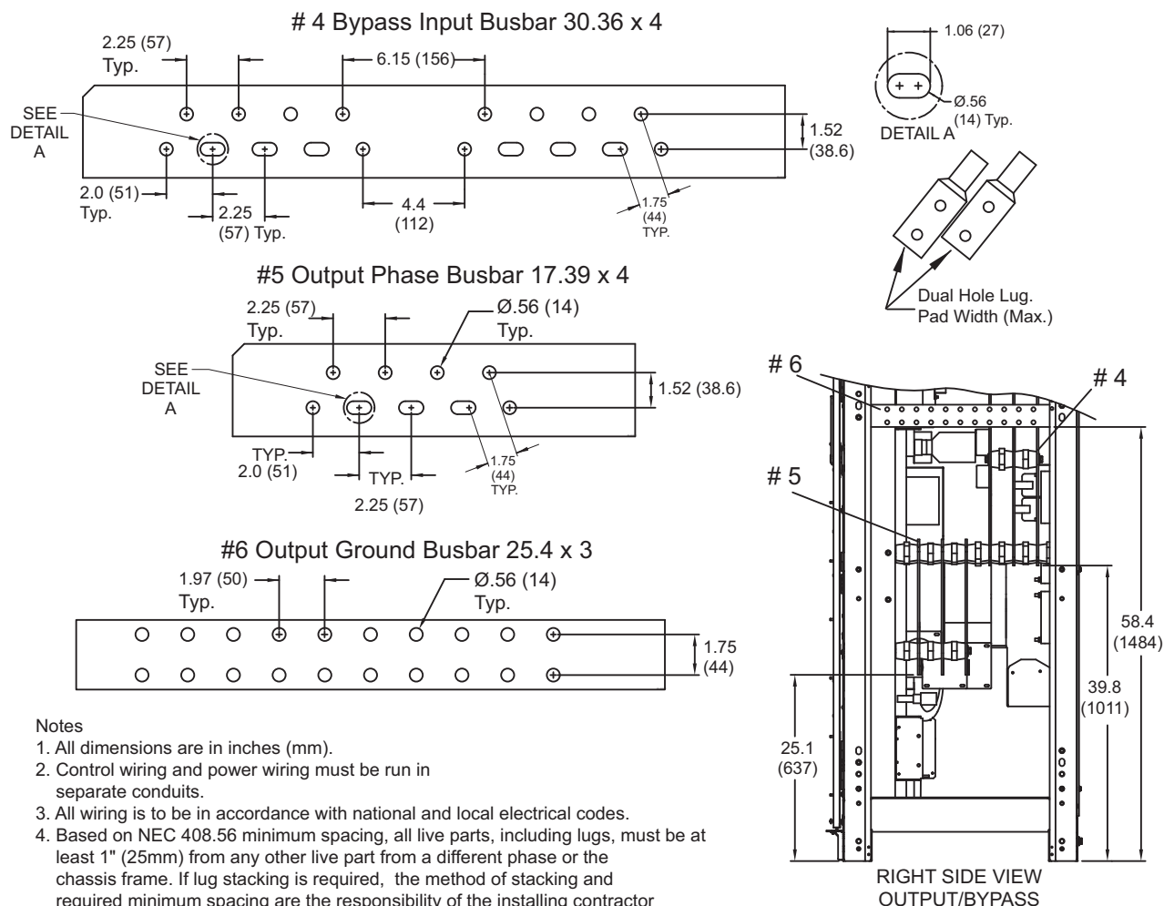
Figure 9 Output and bypass terminal detail, 625-800kVA Liebert eXL single-module UPS
