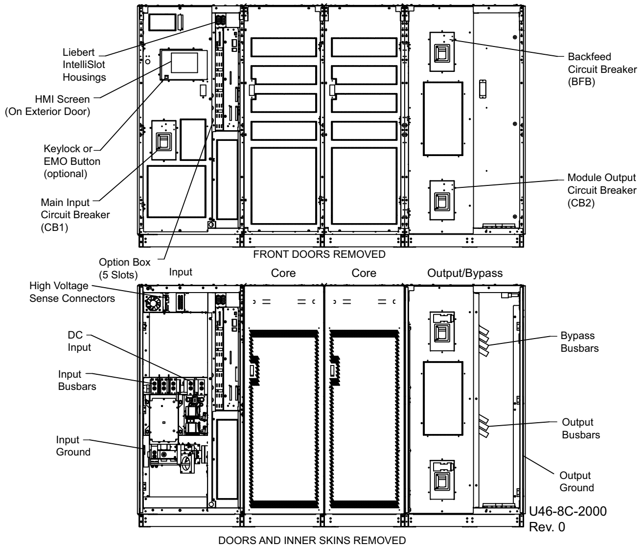
Figure 5 Typical main components, 625-800kVA Liebert eXL single-module UPS
