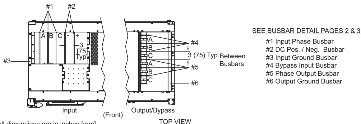
Figure 10 Input, output and bypass terminal spacing details, 625-800kVA Liebert eXL single-module UPS
