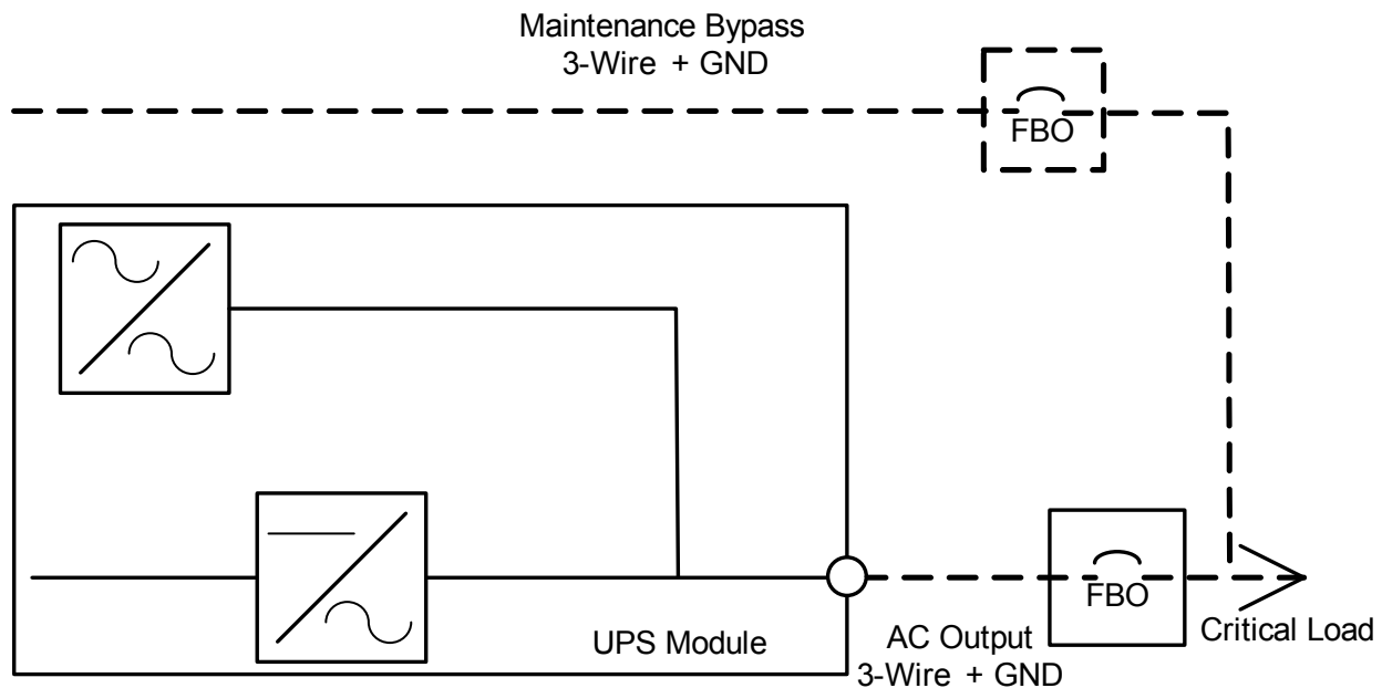
Figure 3 No CB2 option
