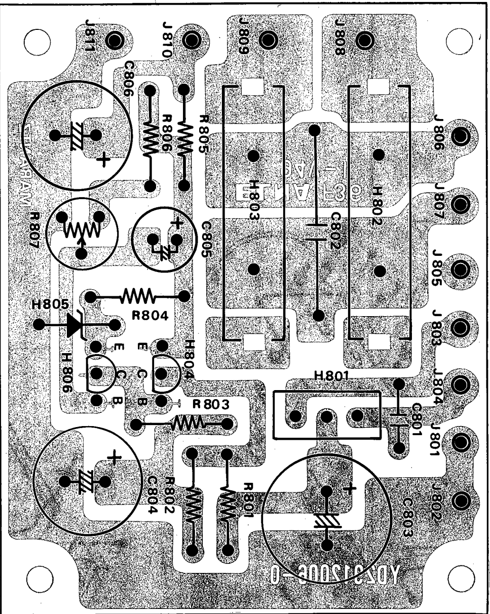
Figure 9. Power Supply Circuit Assembly P800 Component Locations
