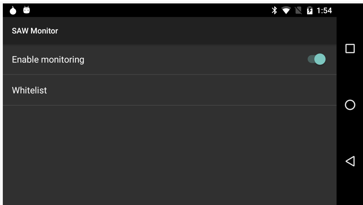
Figure 633: SAWMonitor SettingsFragment
