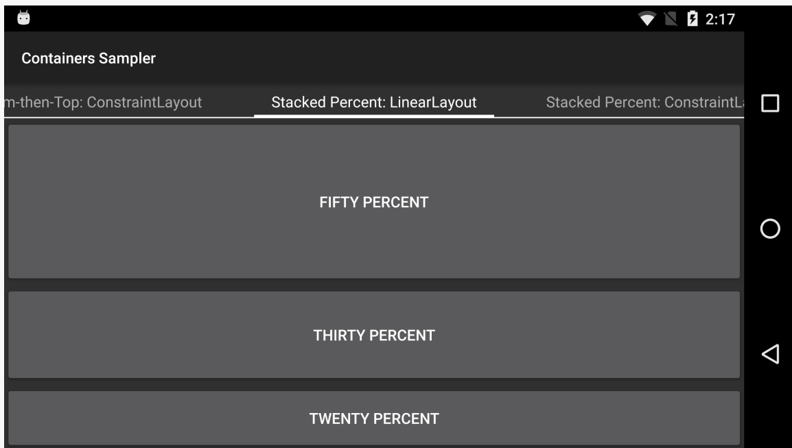
Figure 113: Stacked-Percent Layout, Using LinearLayout
