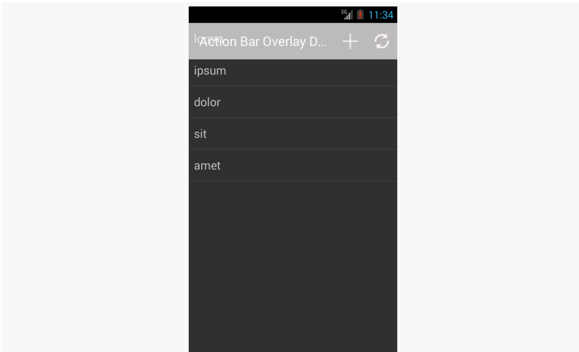
Figure 500: AppCompatActivity with FEATURE_ACTION_BAR_OVERLAY on an Android 4.3 Emulator
