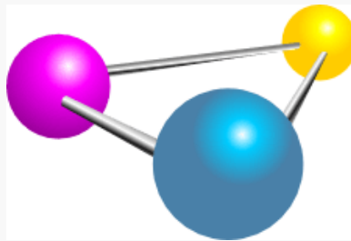
Figure 57: CommonsWare
