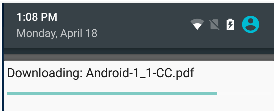
Figure 431: Custom Notification
