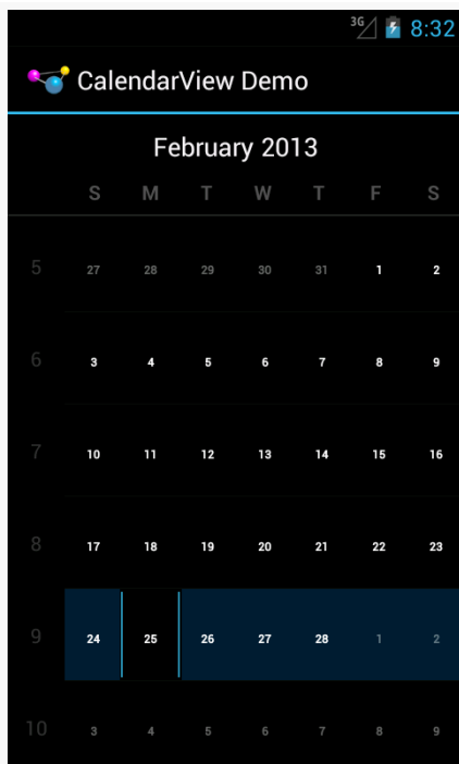
Figure 1072: Android 4.1
