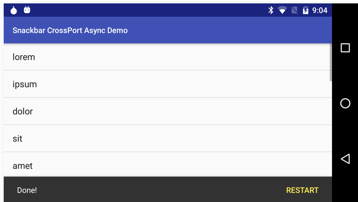
Figure 507: CWAC-CrossPort Snackbar
