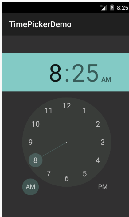
Figure 1094: Android 5.0
