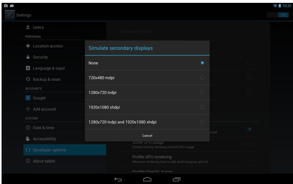
Figure 813: Nexus 10 “Simulate secondary displays” Options
