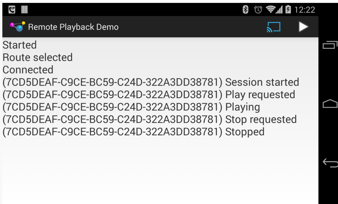
Figure 811: RemotePlaybackClient Demo, on a Nexus 4, After Playback Has Stopped
