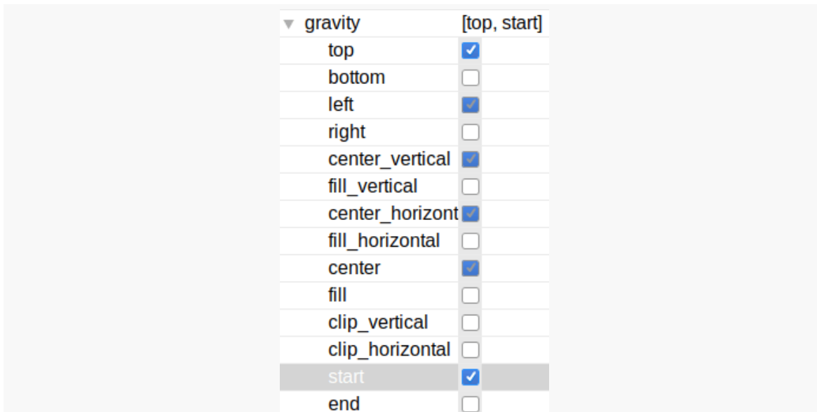
Figure 154: Layout Editor Attributes Pane, Showing Gravity Options
