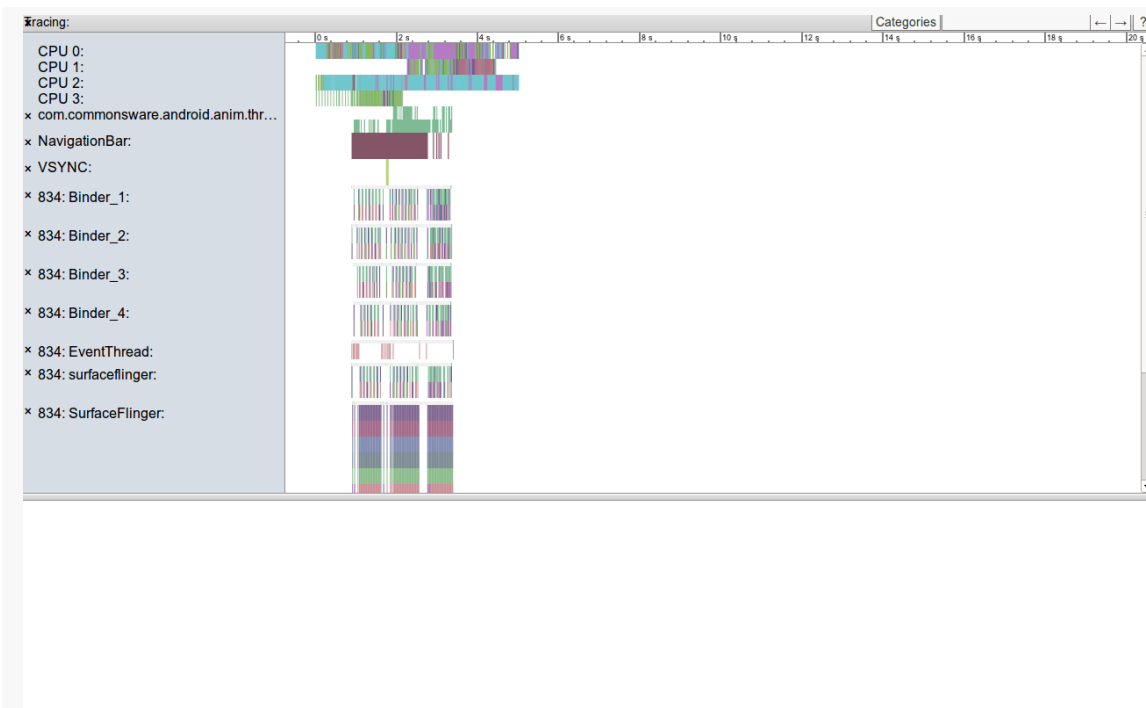
Figure 995: Systrace Output, As Initially Viewed
