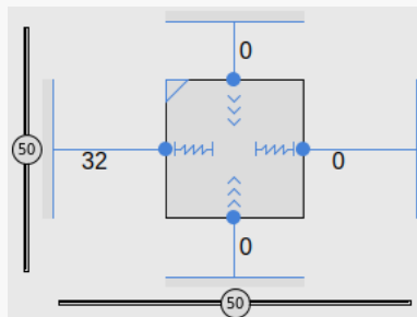
Figure 187: Constraint Configuration Thing, Showing "Match Constraints" Sizing
