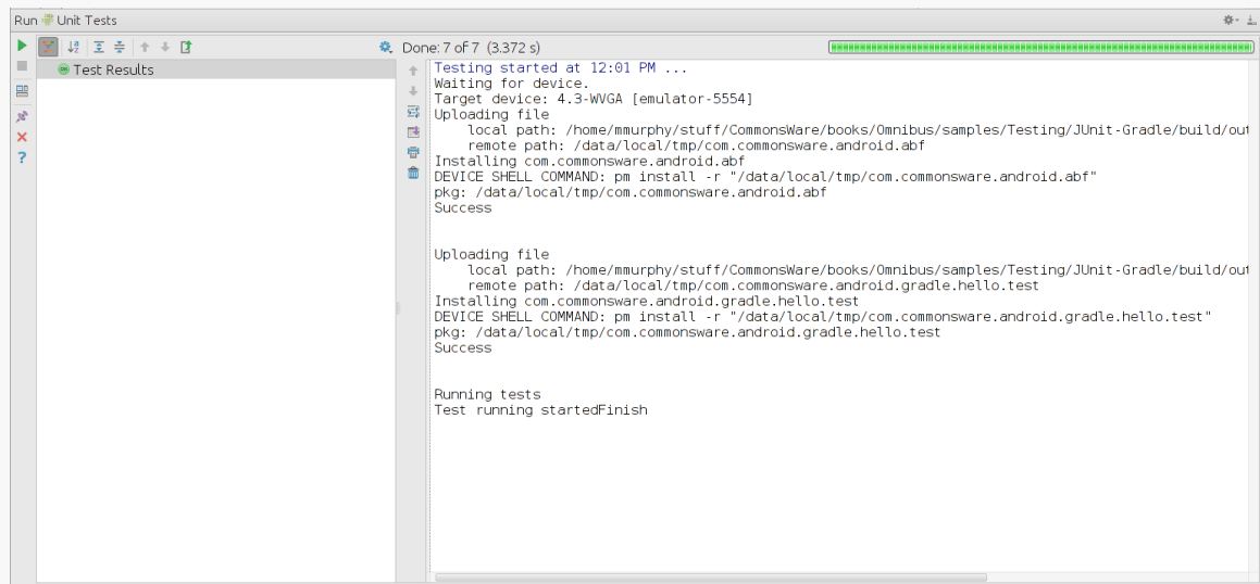
Figure 352: Android Studio, Showing Run Unit Tests Results
