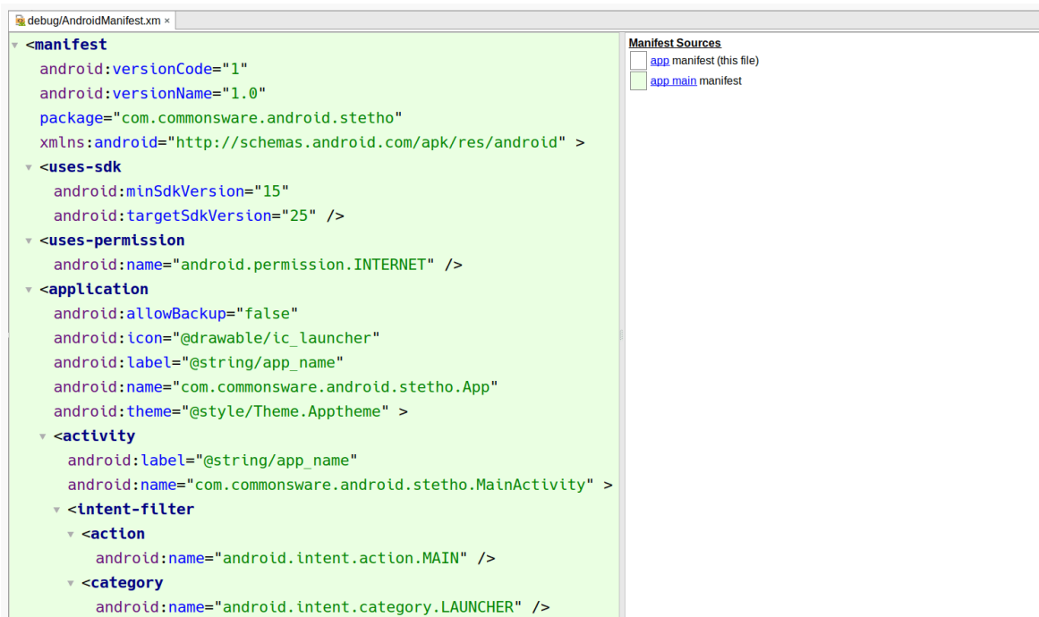
Figure 969: Merged Manifest for Release Build, Showing No StethoApp
