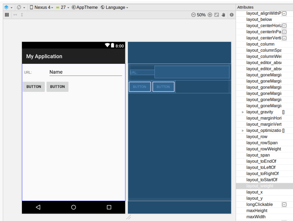
Figure 122: Two Smaller Buttons in Lower Horizontal LinearLayout
