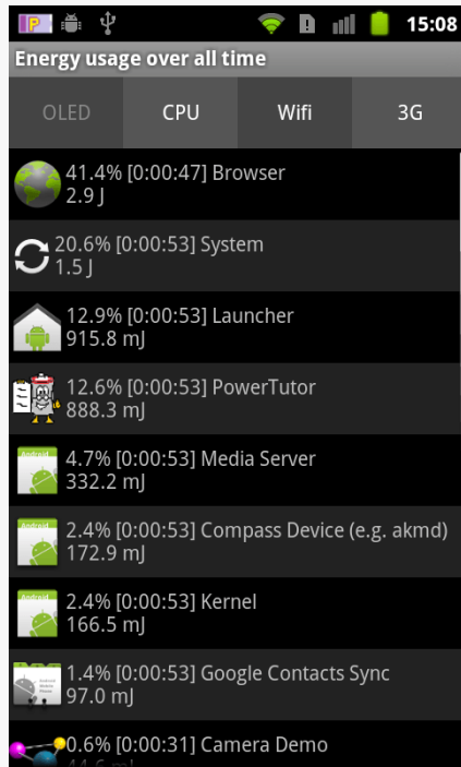
Figure 1052: The PowerTutor application roster
