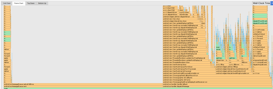
Figure 987: Method Tracing, Flame Chart, As Initially Launched
