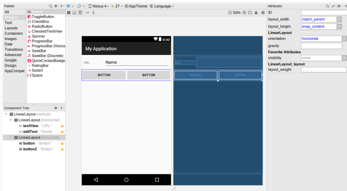
Figure 121: Two Buttons in Lower Horizontal LinearLayout
