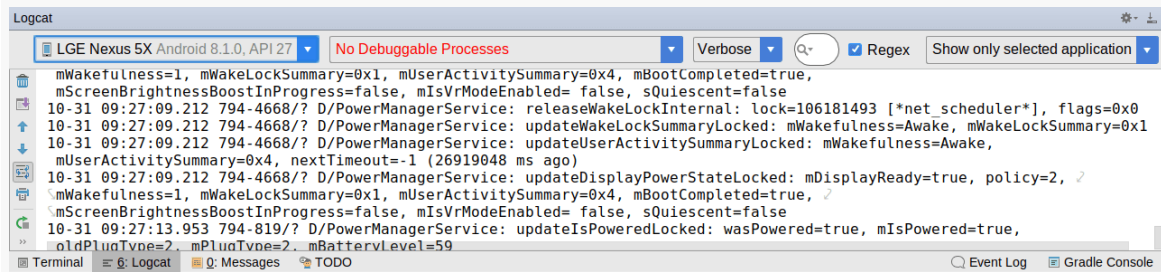
Figure 103: Android DDMS Tool Window, Showing Logcat
