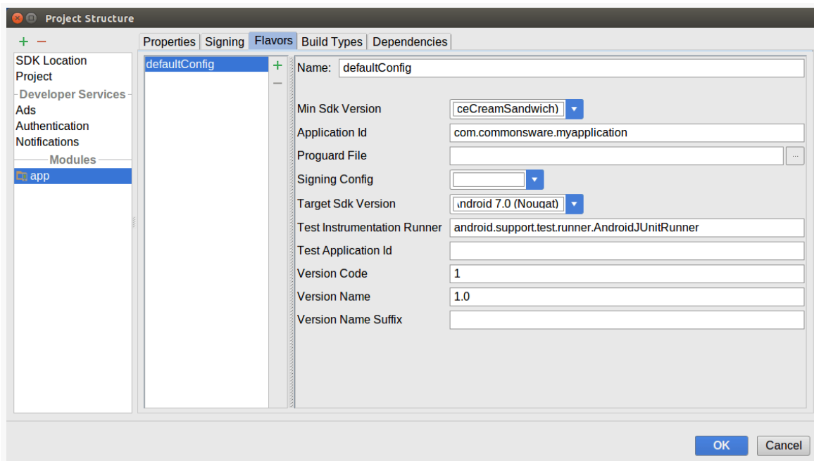
Figure 922: Project Structure Dialog, Module Category, Flavors Tab
