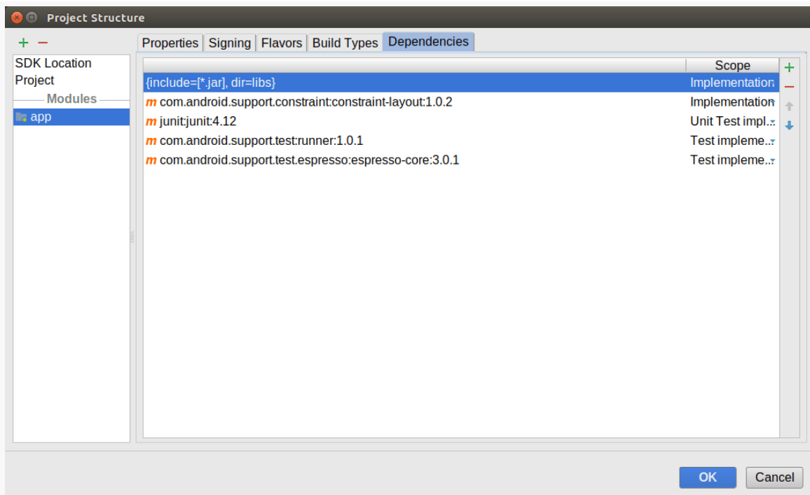
Figure 924: Project Structure Dialog, Module Category, Dependencies Tab
