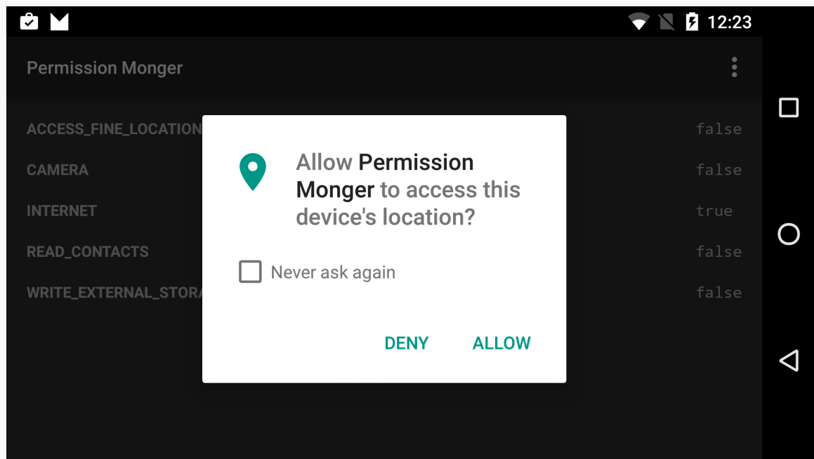
Figure 266: Permission Monger, Requesting ACCESS_FINE_LOCATION Permission (Again)
