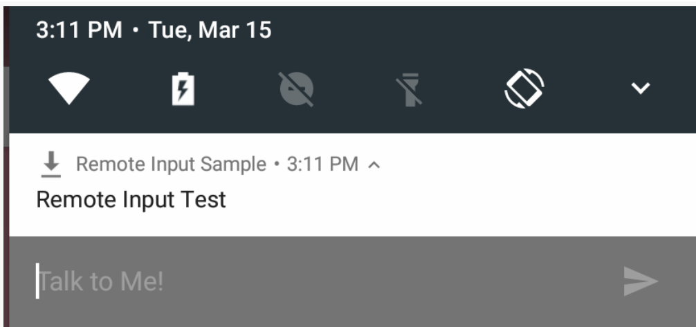
Figure 419: Notification with Remote Input
