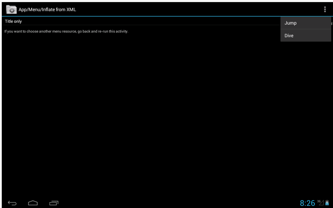
Figure 199: Action Bar with Open Overflow Menu
