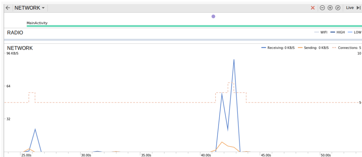
Figure 1018: Android Studio, Android Profiler, Detailed Network Graph
