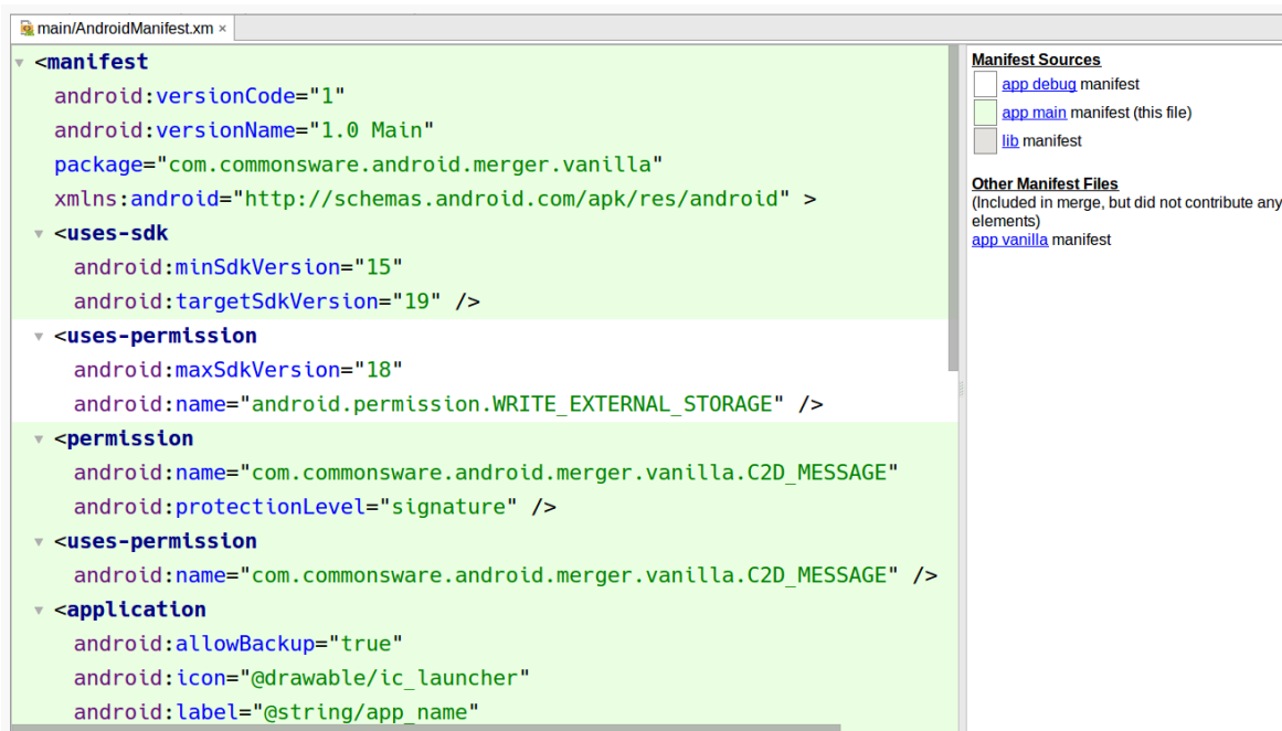
Figure 331: Merged Manifest Tab
