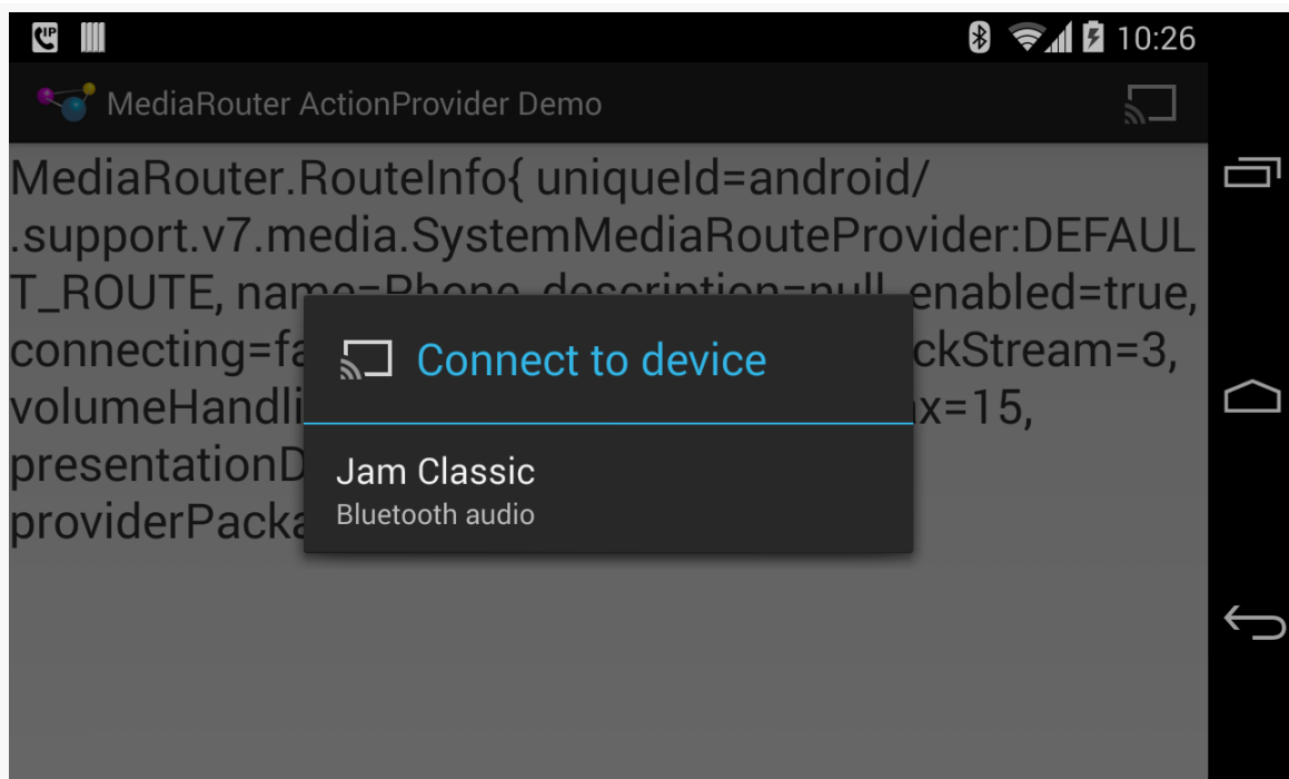
Figure 800: MediaRouter ActionProvider Demo, on a Nexus 4, Showing Available Routes
