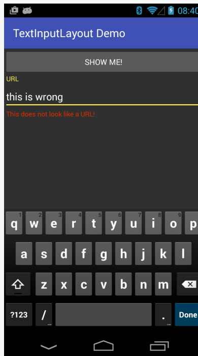
Figure 525: FloatingLabel Sample, After Erroneous Data Entry
