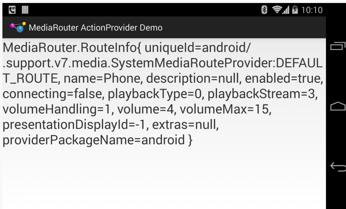
Figure 796: MediaRouter ActionProvider Demo, on a Nexus 4, Showing Default Route
