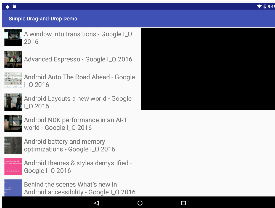
Figure 710: Simple Drag-and-Drop Demo, As Initially Launched
