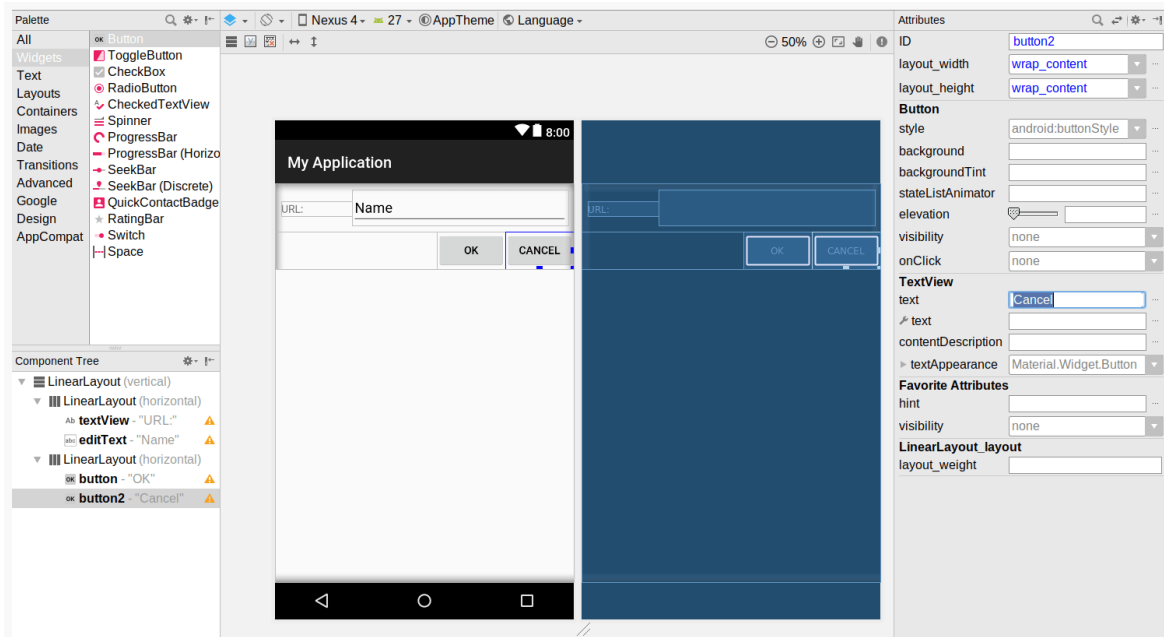
Figure 124: Buttons with Desired Captions
