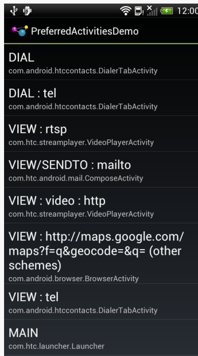
Figure 897: Preferred Activities on a Stock HTC One S
