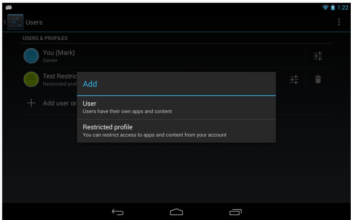
Figure 841: Add Dialog in Users Screen in Settings
