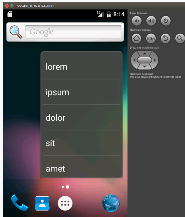
Figure 747: Resized LoremWidget on Android Home Screen
