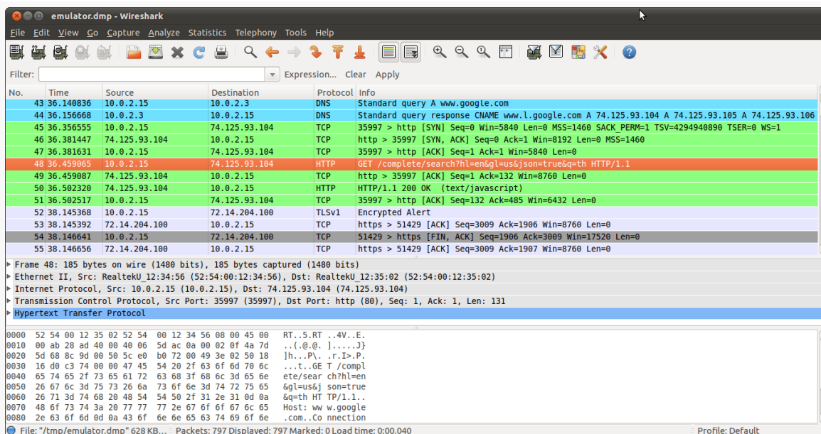
Figure 1016: Wireshark examining captured emulator packets
