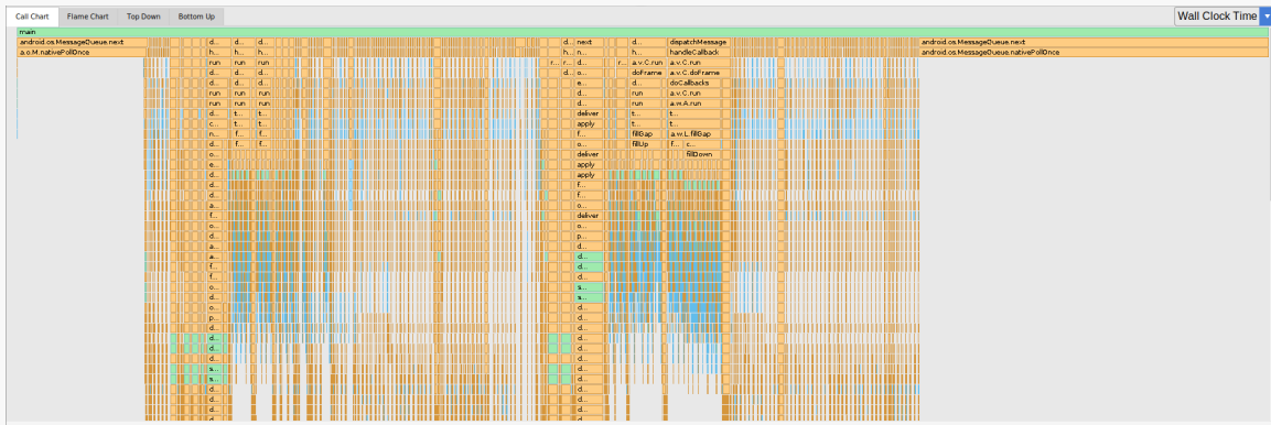
Figure 986: Method Tracing, Call Chart, As Initially Launched
