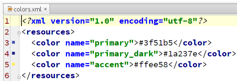
Figure 211: Color Resources in Android Studio
