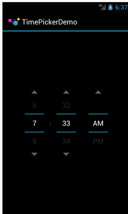
Figure 1093: Android 4.0.3
