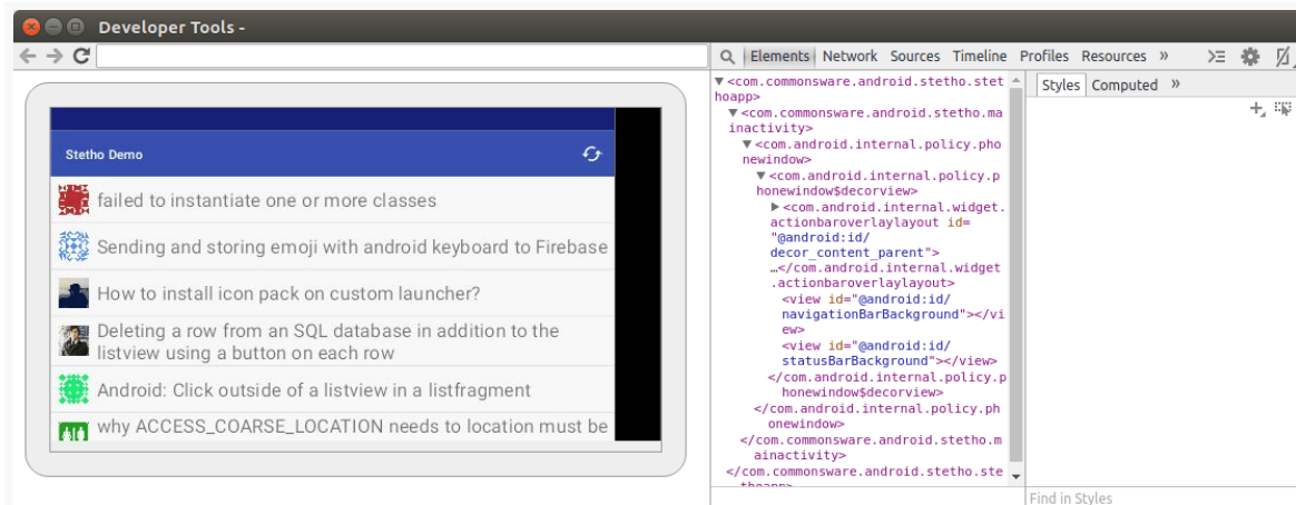
Figure 977: Stetho Screenshot
