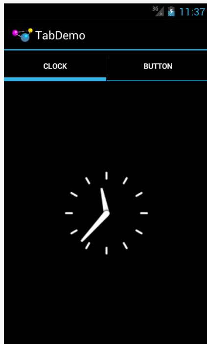
Figure 1091: Android 4.0.3
