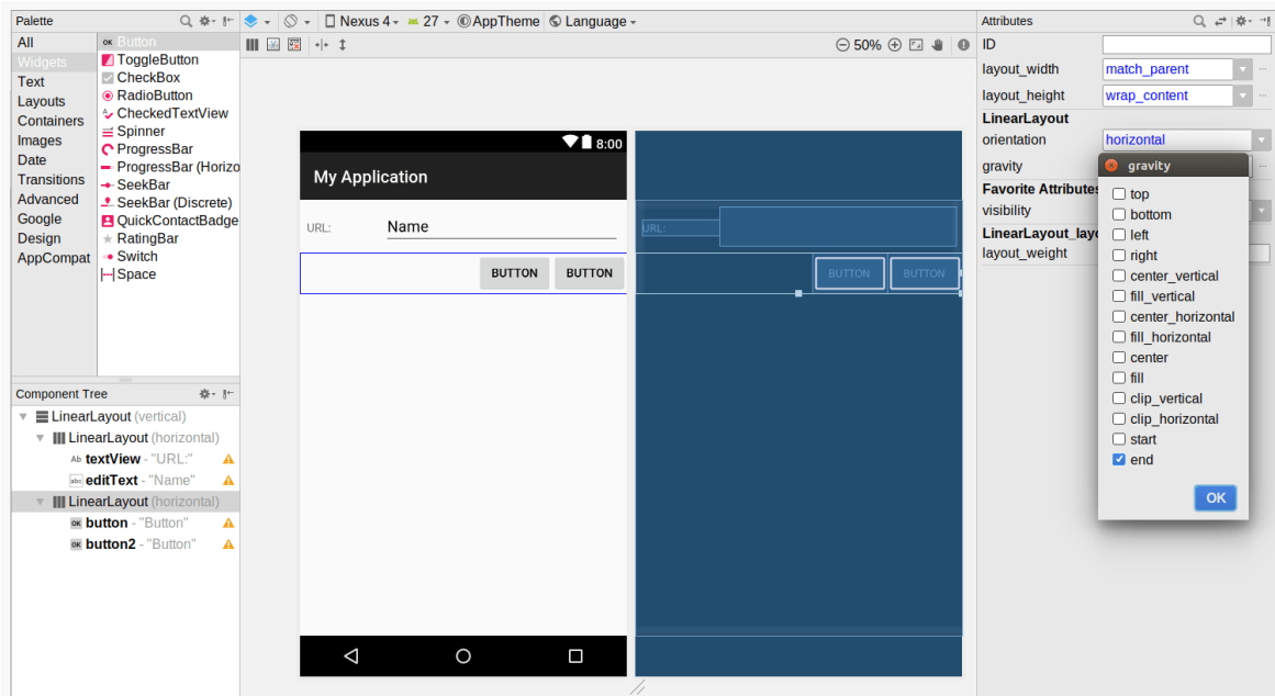
Figure 123: Two Smaller Right-Flush Buttons in Lower Horizontal LinearLayout
