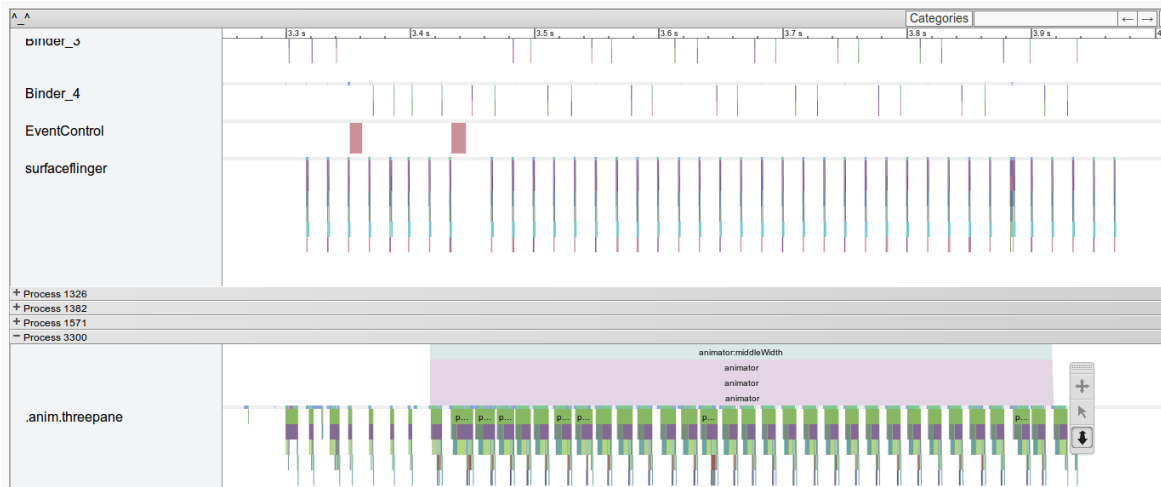
Figure 996: Systrace Output, Zoomed In on 0.7 Seconds of Profiling
