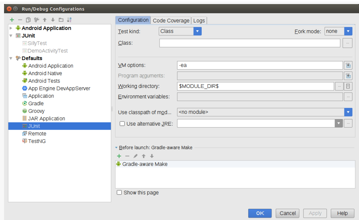
Figure 375: Run/Debug Configurations, JUnit Defaults, Modified
