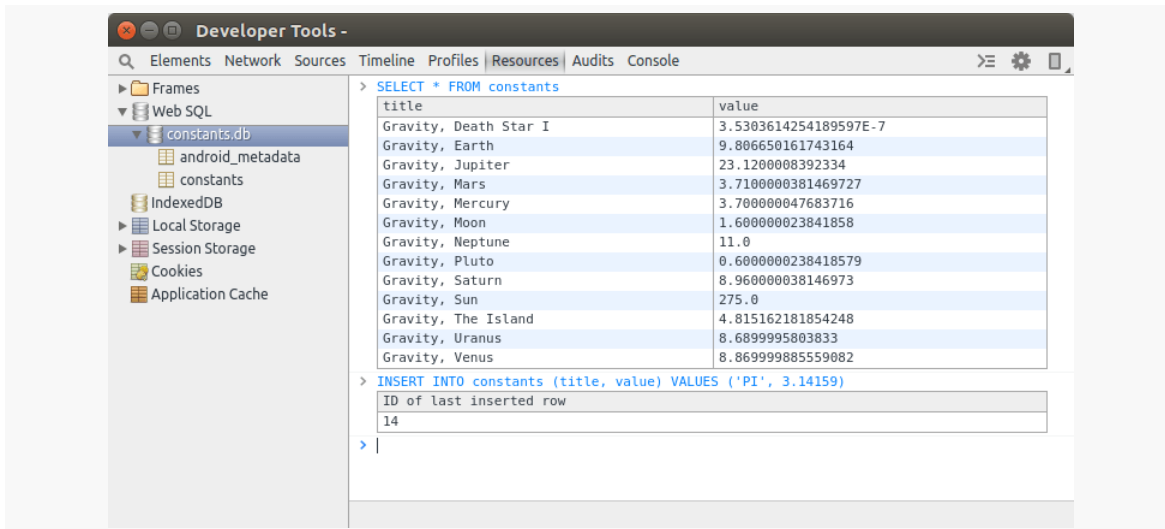
Figure 979: Resources Tool, Showing Interactive SQL
