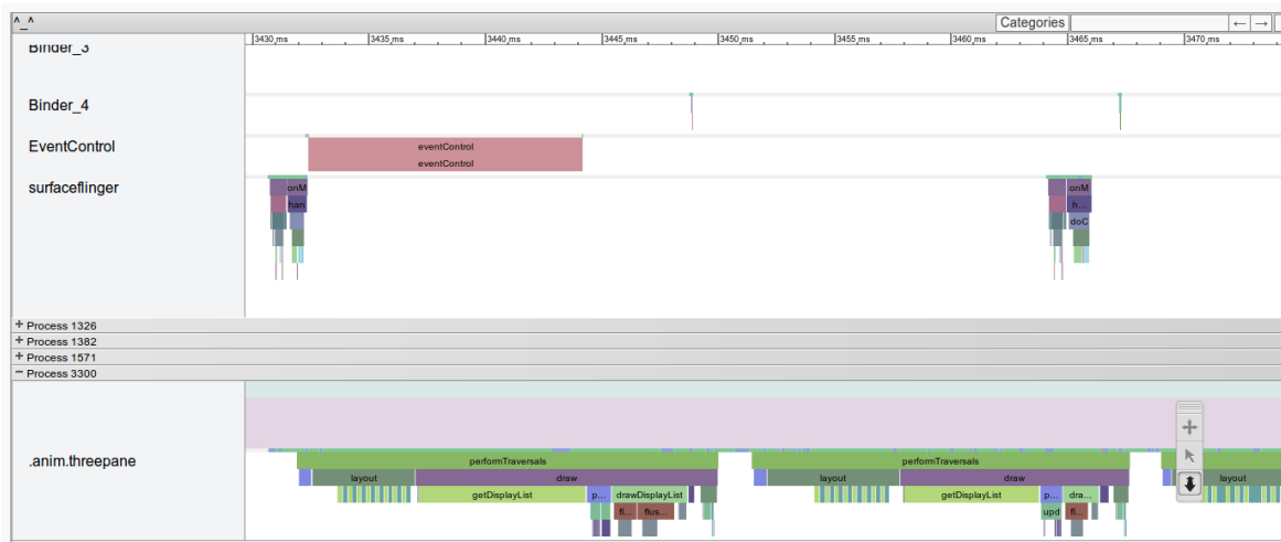
Figure 997: Systrace Output, Zoomed In on 40 Milliseconds of Profiling
