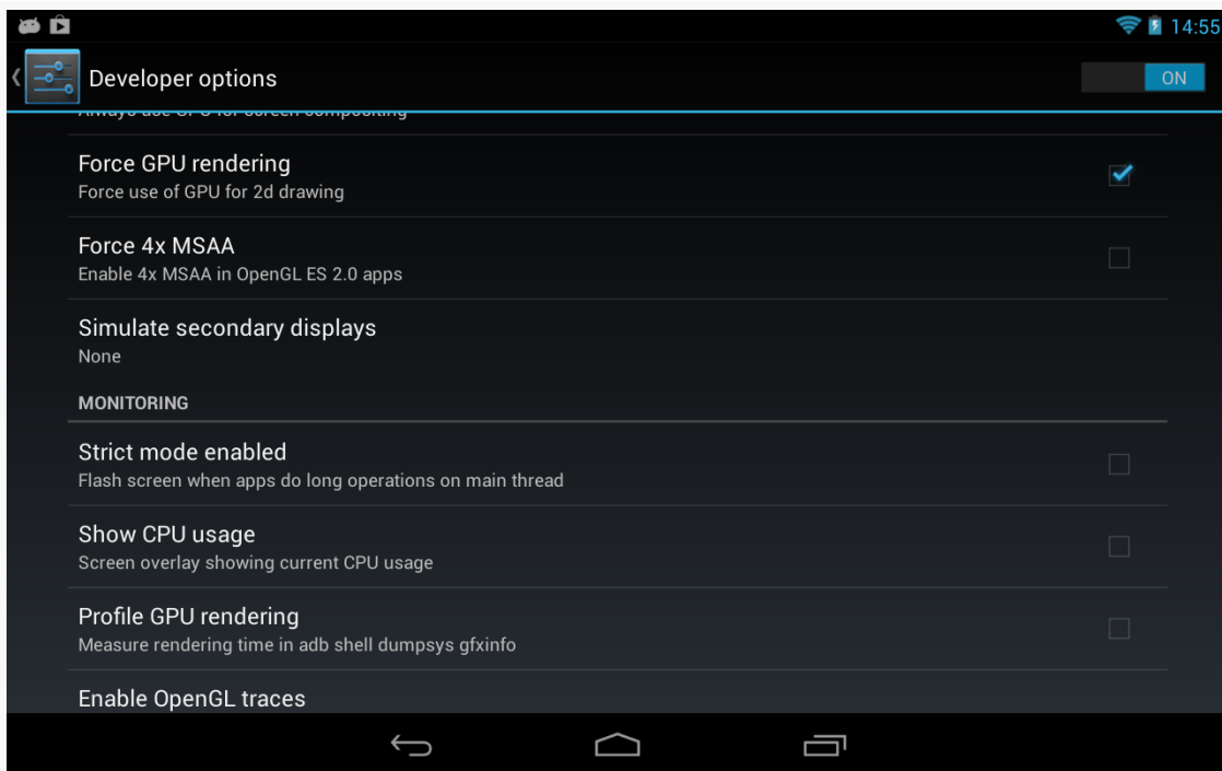
Figure 990: Developer Options, Showing “Force GPU rendering” and “Profile GPU rendering”
