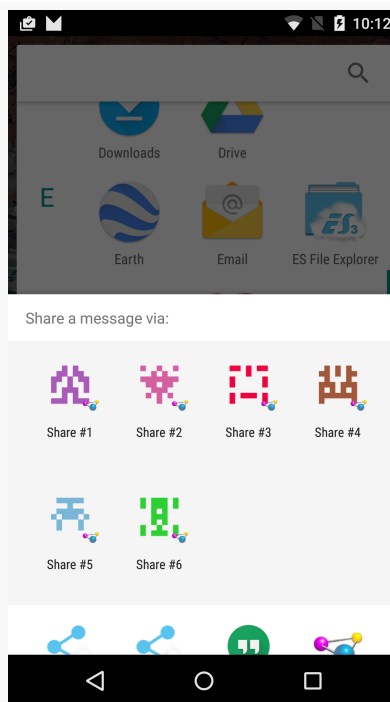
Figure 901: Chooser, Showing Direct-Share Targets
