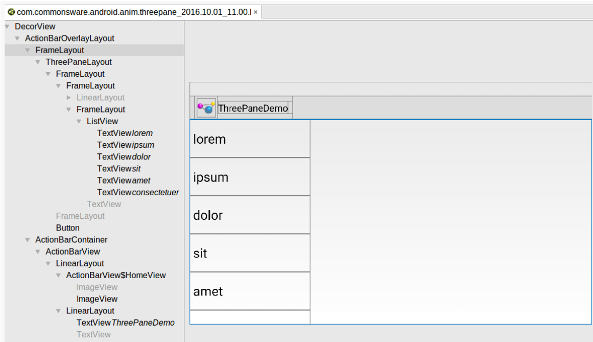
Figure 1008: Three-Pane Demo in Layout Inspector, Showing More Hierarchy
