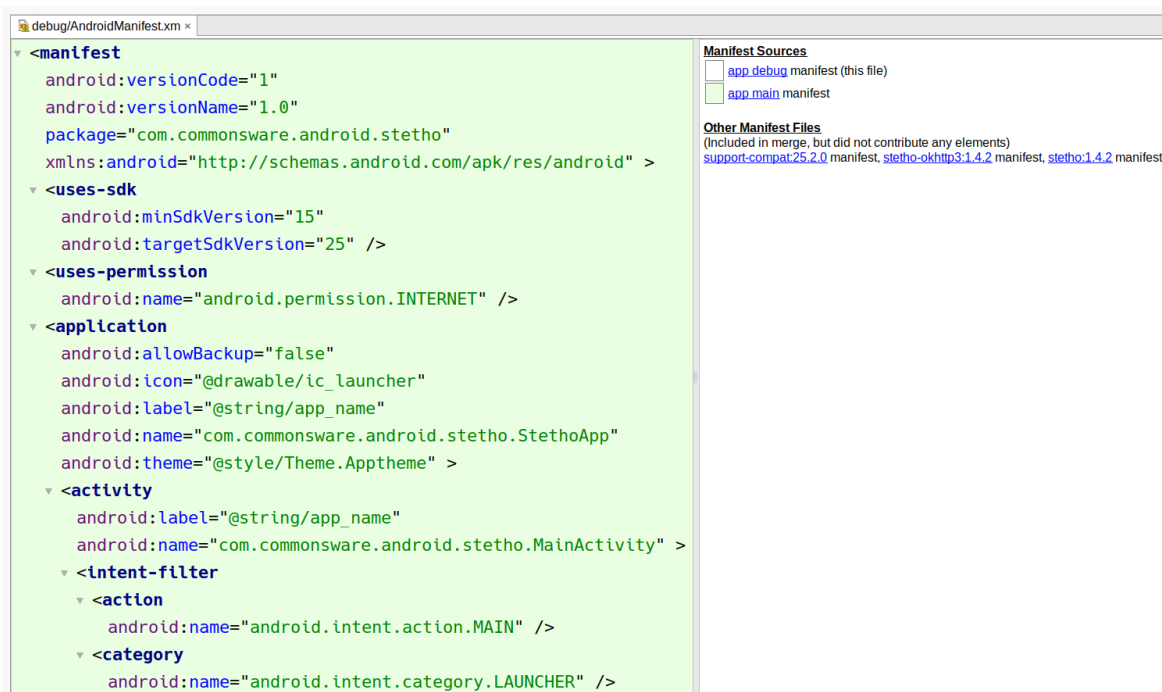
Figure 968: Merged Manifest for Debug Build, Showing StethoApp
