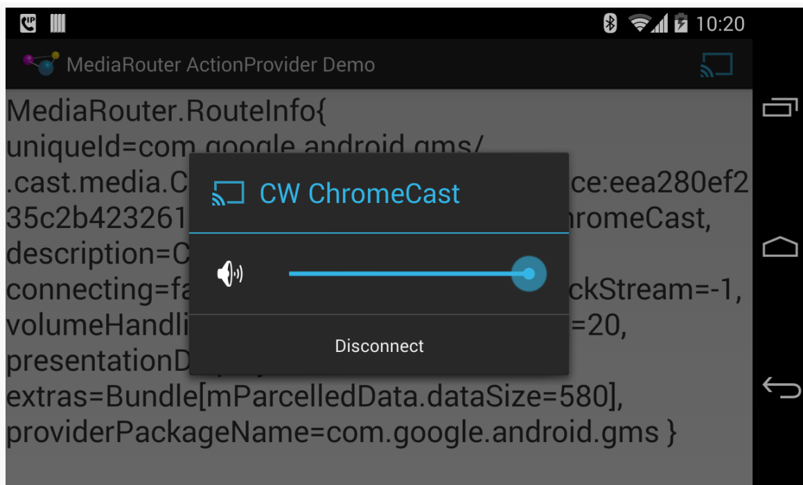
Figure 8o6: MediaRouter ActionProvider Demo, on a Nexus 4, Showing Route Dialog
