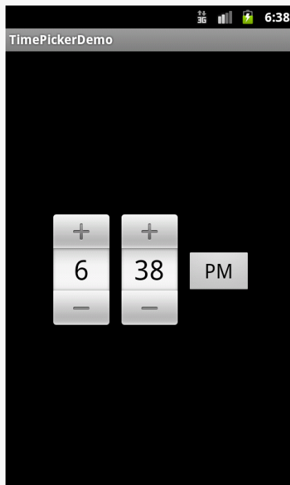
Figure 1092: Android 2.3.3
