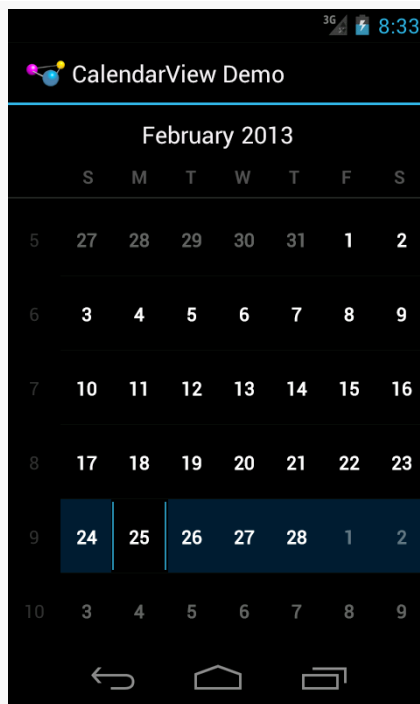
Figure 1071: Android 4.0
