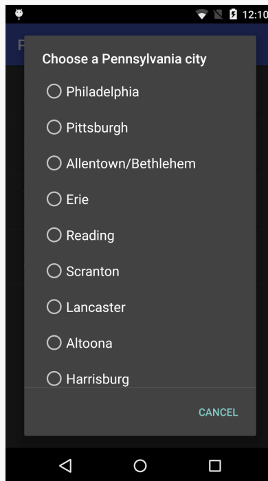
Figure 287: ListPreference UI
