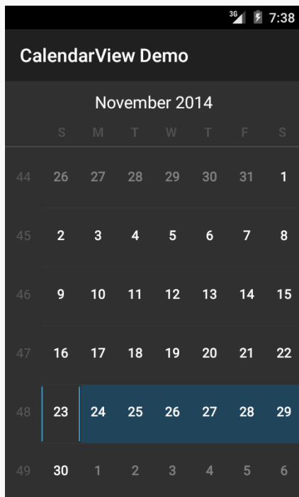
Figure 1073: Android 5.0
