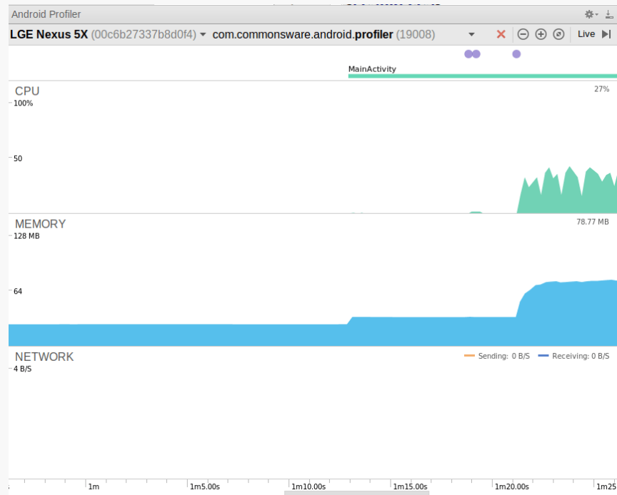
Figure 983: Android Profiler
