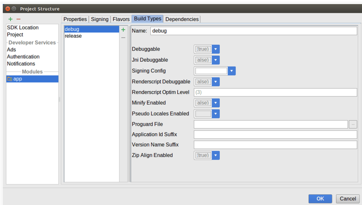
Figure 923: Project Structure Dialog, Module Category, Build Types Tab
