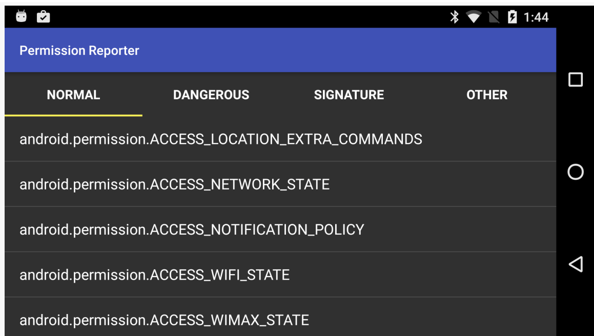
Figure 838: PermissionReporter, Normal Tab, on Android 6.0
