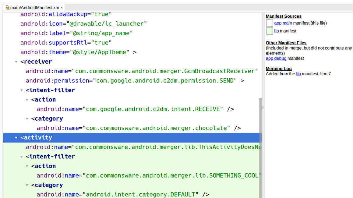
Figure 334: Merged Manifest View, Showing Merged Element
