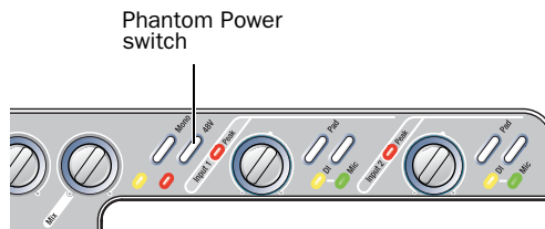
Phantom Power switch
