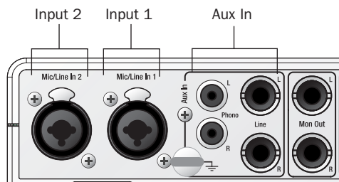
Inputs on back of Mbox 2 Pro
