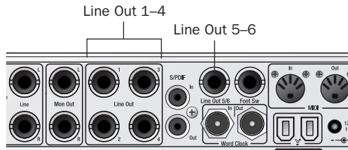
Additional outputs on Mbox 2 Pro (back panel)
