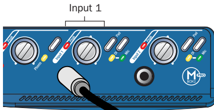
Connecting a 1/4-inch microphone cable to the Input 1 DI connector
