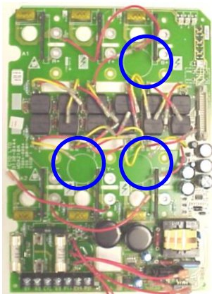
(16) MDA210R Power Board P/N 9204-0555
