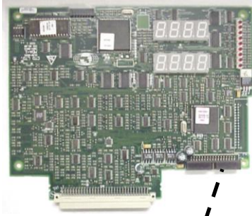
(9) MDA1 CPU PN: 9200-0784
