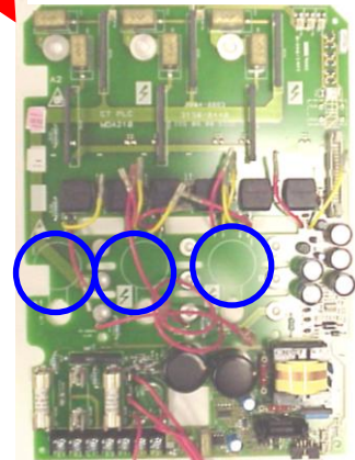
(18) MDA210 Power Board P/N 9200-0619
