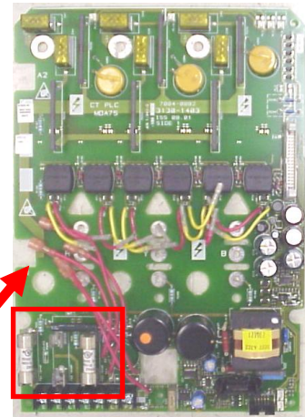
(15) MDA75 Power Board P/N 9200-0624
