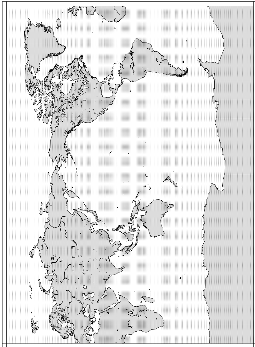
Figure 10: GFS 3,4,193, (dots correspond to the 1.0° NAM 3 grid)
