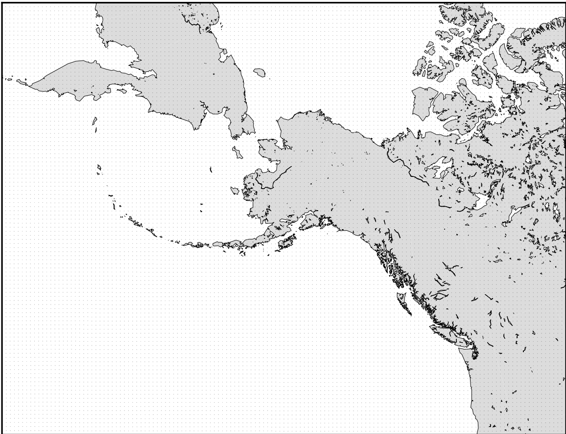
Figure 3: NAM 216, AK 45.0 km Polar Stereographic
