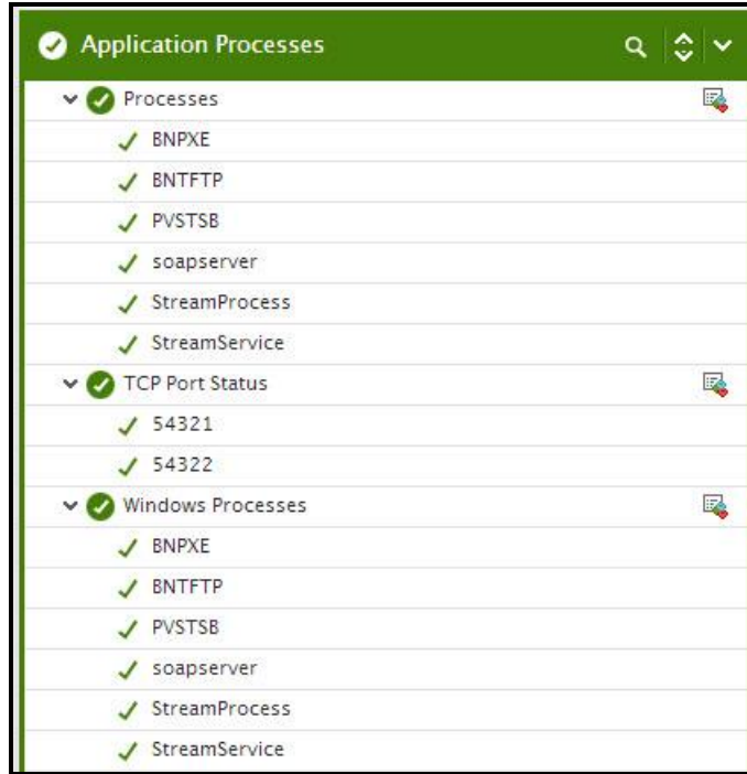
Figure 11: The tests mapped to the Application Processes layer
