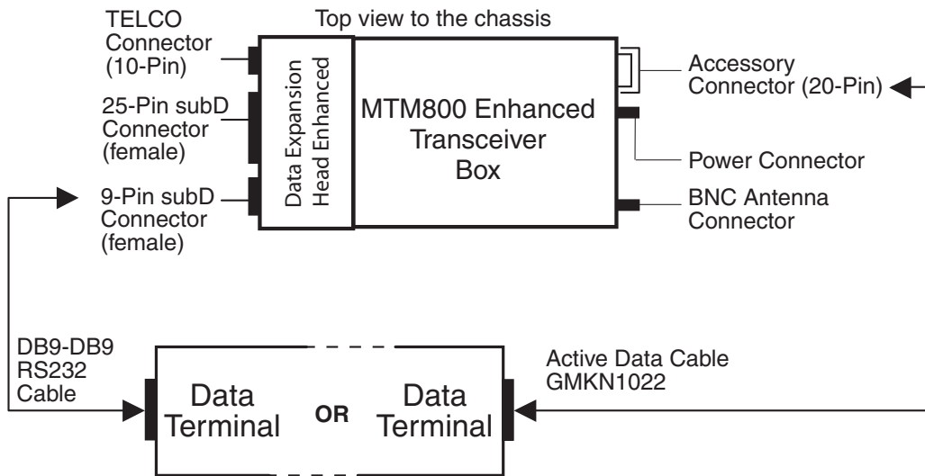
Figure 22 Data Box Radio Configuration
