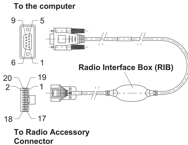
Figure 36 Active Data Cable GMKN1022
