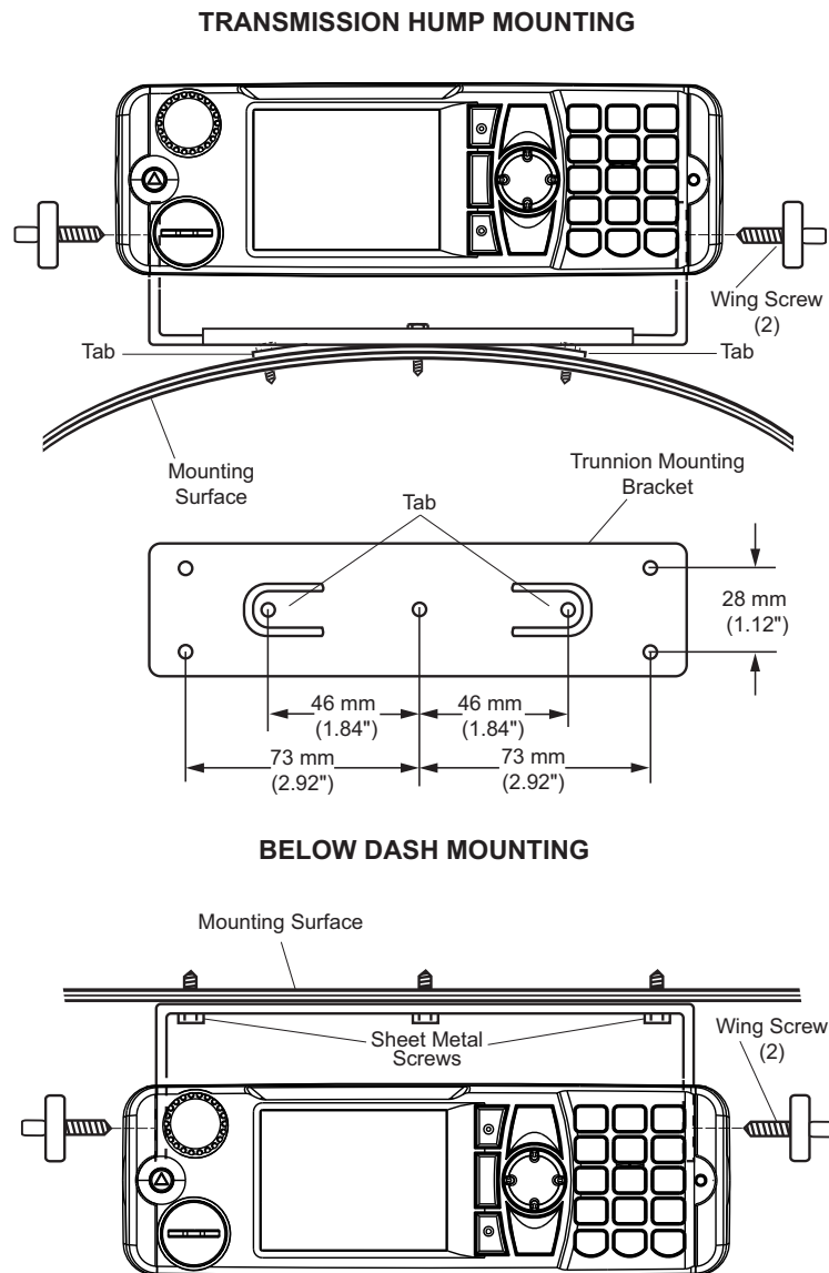
Figure 7 Transmission Hump Mounting (Top) and Below Dash Mounting (Bottom)
