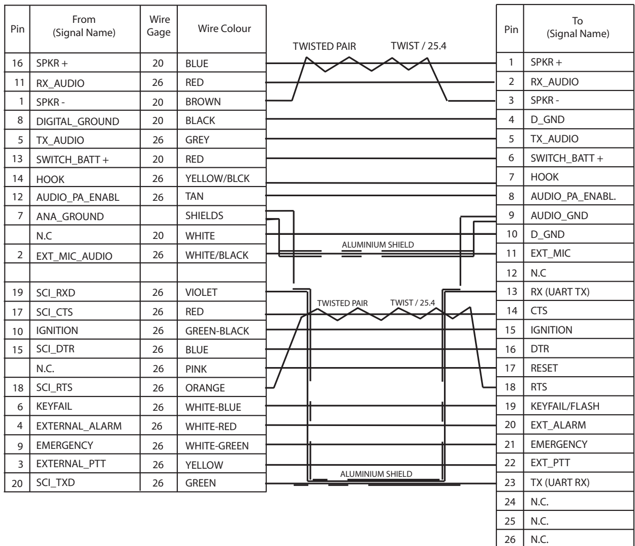
Figure 33 Connecting Cable - Radio-to-Junction Box
