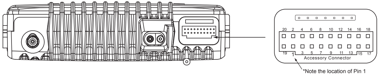
Figure 26 Location of Accessory Connector - Rear Side
