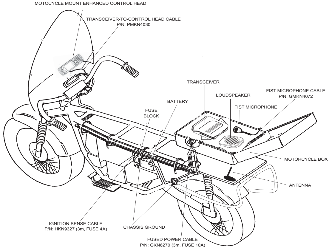
Figure 17 Motorcycle Installation
