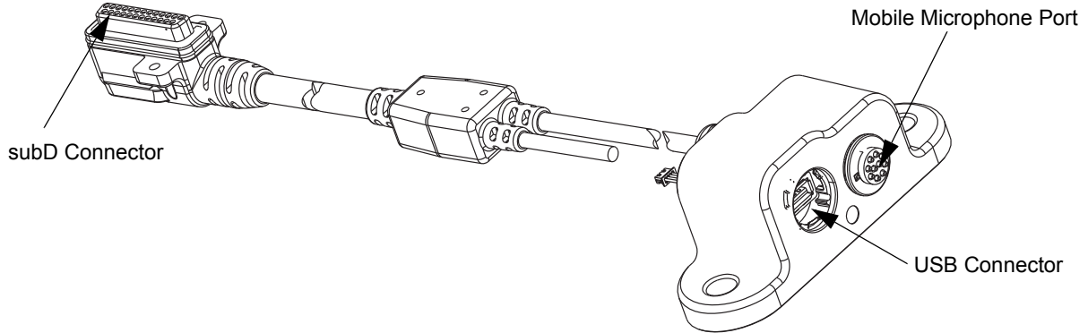
Figure 32 Connecting Cable - Accessories Expansion Cable
