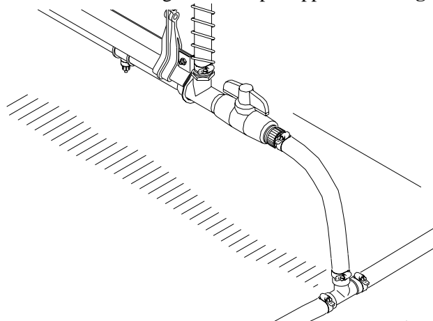
Figure 21. Flush System Component Connection Diagram
