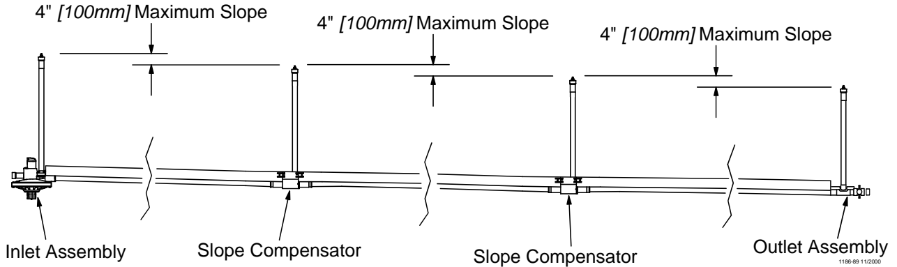
Figure 16. Slope Compensator Assembly Installation
