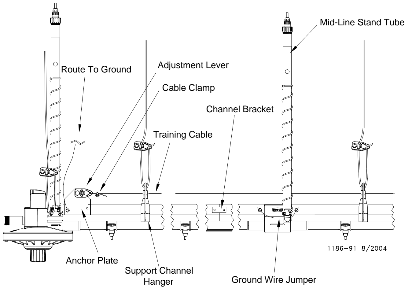
Figure 19. Anti-Roost Components
