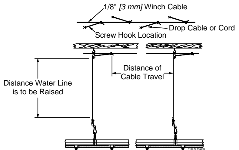
Figure 5. Offset the Screw/Ceiling Hooks
