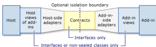
Add-in pipeline
