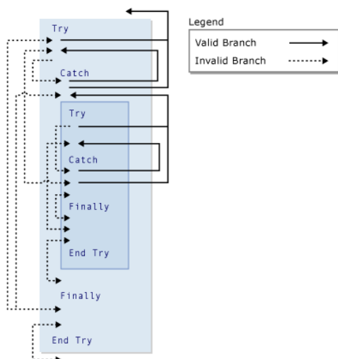
Valid and invalid branches in Try constructions
