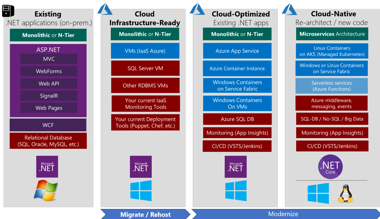
Figure 1-3. Internal technologies for each modernization maturity level
