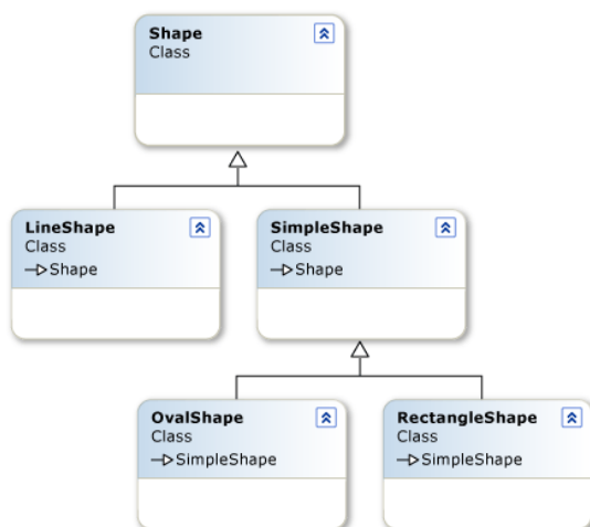
Line and Shape object hierarchy
