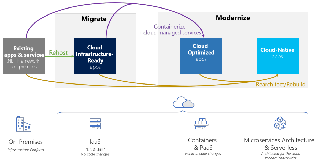
Figure 1-1. Modernization paths for existing .NET applications and services
