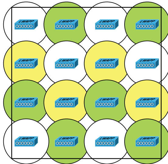
FIGURE 12.18 Enterprise design
