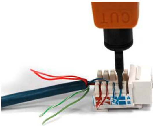
FIGURE 18.23 Using a punch-down tool on a small keystone connector
