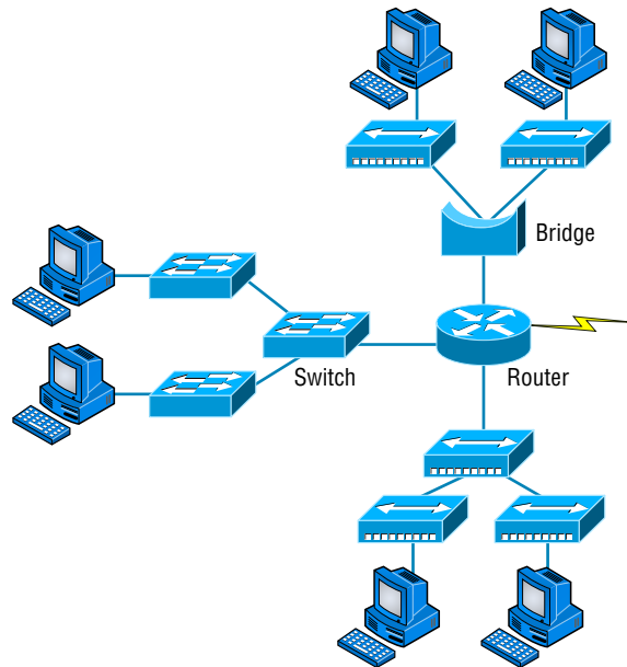
FIGURE 5.26 Internetworking devices
