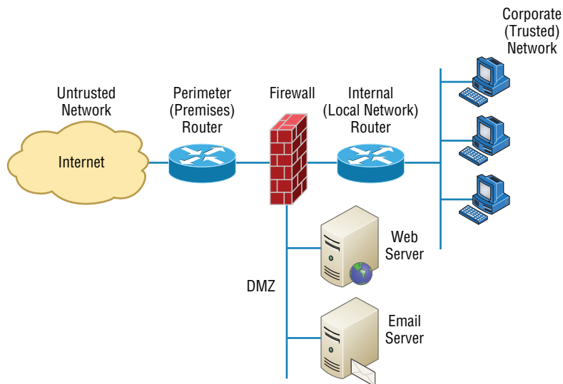
FIGURE 15.1 A typical secured network
