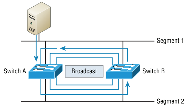
FIGURE 11.9 Multiple frame copies
