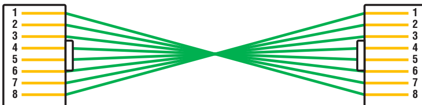
FIGURE 3.25 Rolled Ethernet cable
