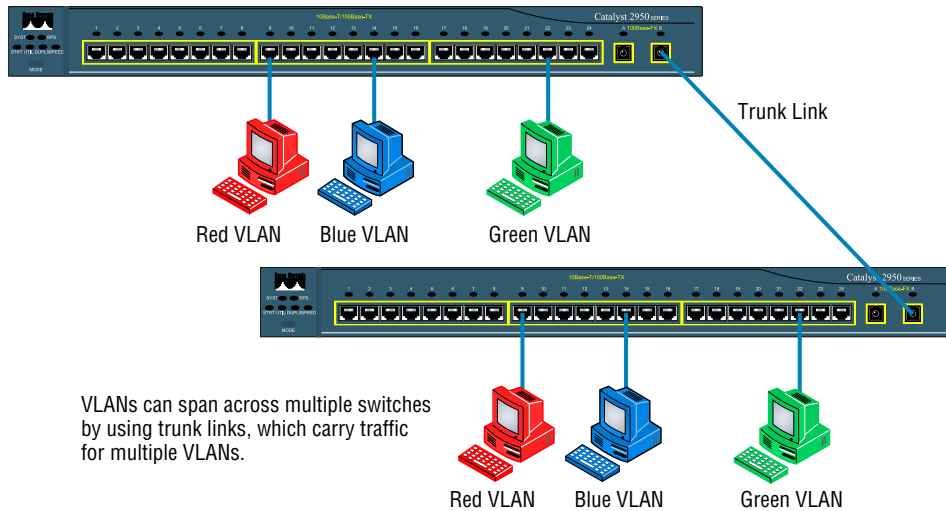
FIGURE 11.16 Access and trunk links in a switched network
