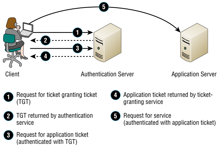
FIGURE 13.13 The Kerberos authentication process
