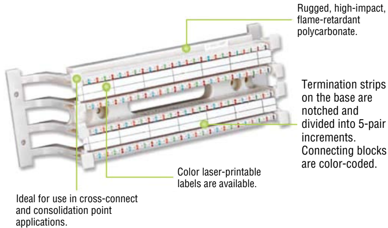
FIGURE 3.27 A 110 block
