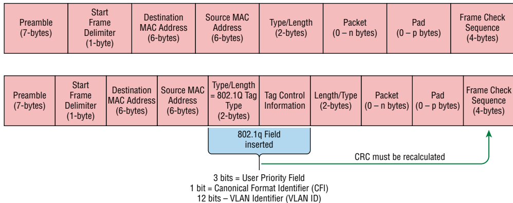
FIGURE 11.17 IEEE 802.1q encapsulation with and without the 802.1q tag
