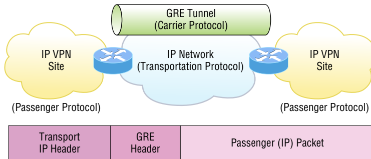
FIGURE 13.5 GRE encapsulation
