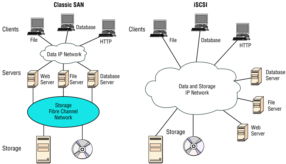
FIGURE 20.12 Classic SAN vs iSCSI
