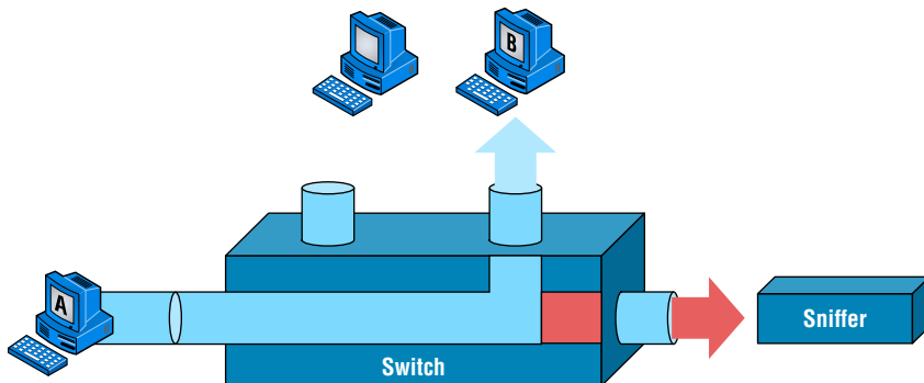
FIGURE 11.26 Port spanning/mirroring
