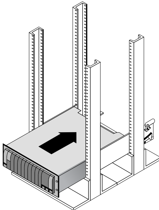
FIGURE 20.17 Four-post rack
