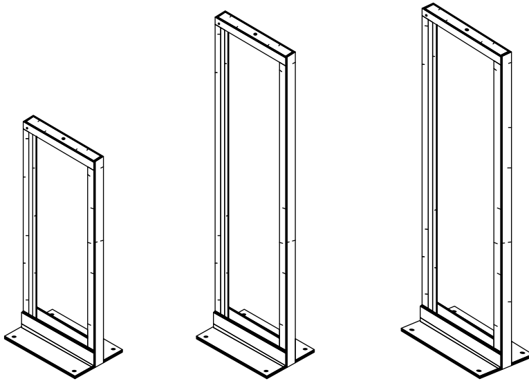
FIGURE 20.16 Two-post racks
