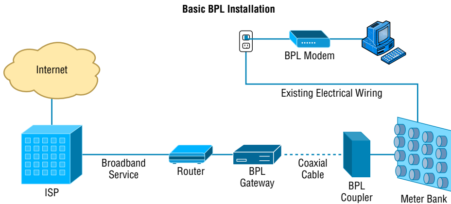
FIGURE 4.8 Basic BPL installation
