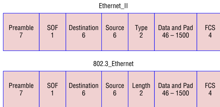
FIGURE 4.5 802.3 and Ethernet frame formats
