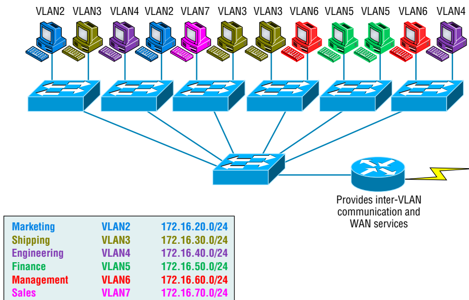
FIGURE 11.15 Switches removing the physical boundary
