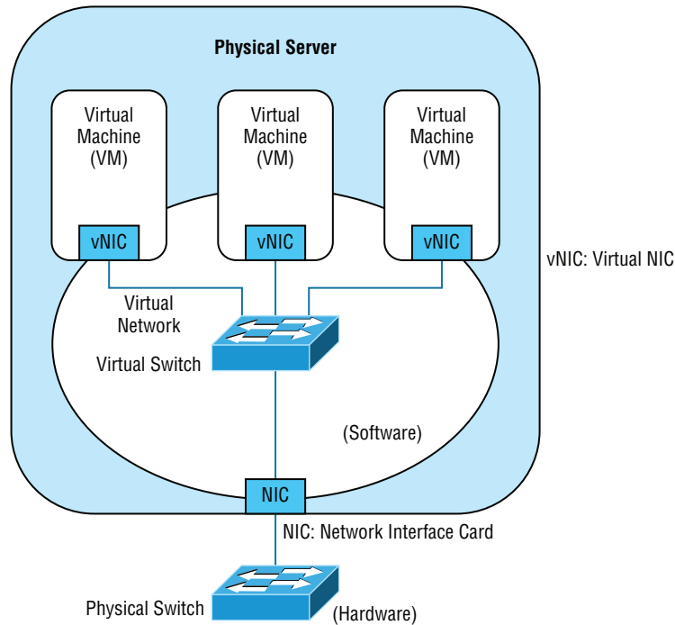
FIGURE 20.11 Virtualization
