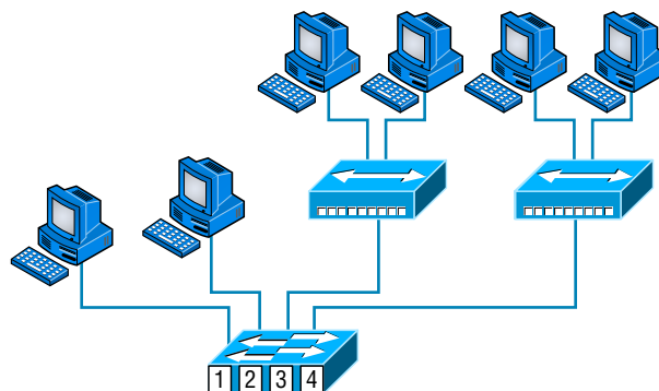
FIGURE 5.29 A switch in an internetwork
