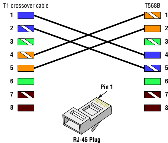
FIGURE 3.26 A T1 crossover cable
