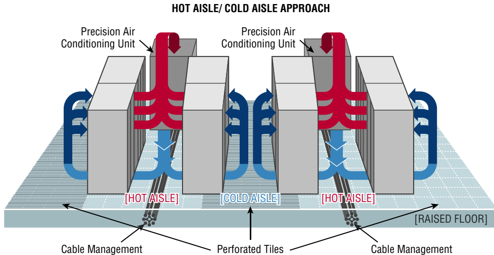
FIGURE 20.9 Hot and cold aisles
