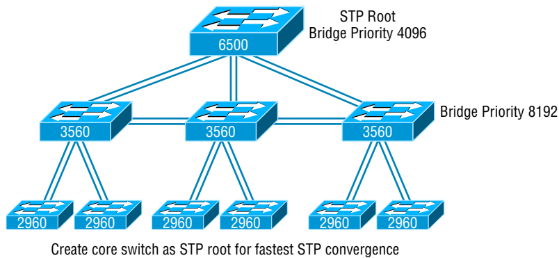
FIGURE 11.11 An optimal hierarchical switch design
