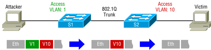
FIGURE 14.7 VLAN hopping
