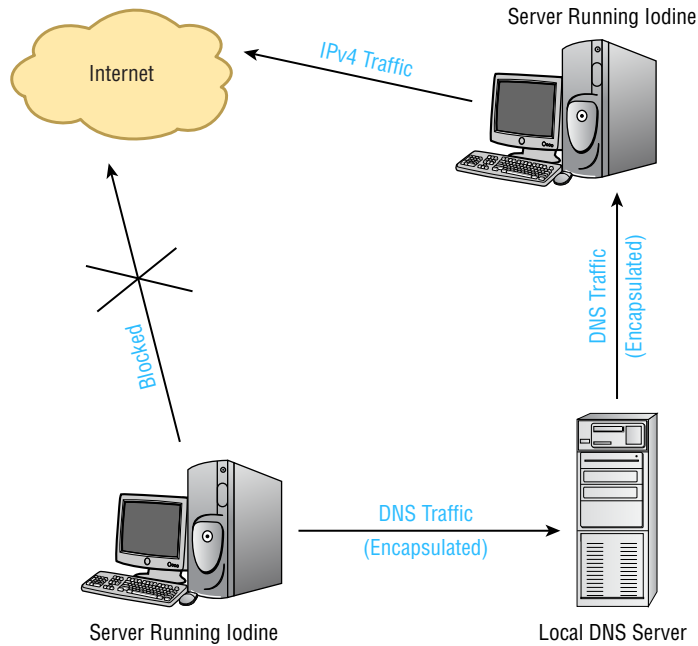
FIGURE 14.6 IPv4 packets tunneled in DNS
