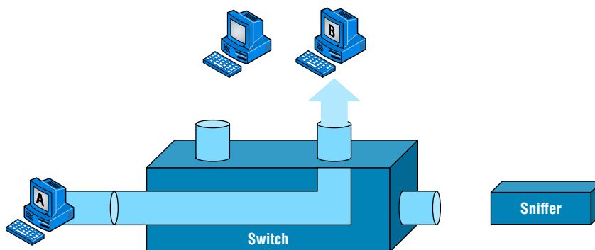
FIGURE 11.24 Switches send frames out the destination port only
