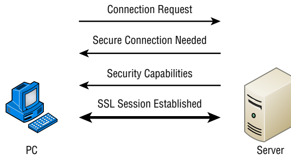
FIGURE 13.4 The SSL connection process
