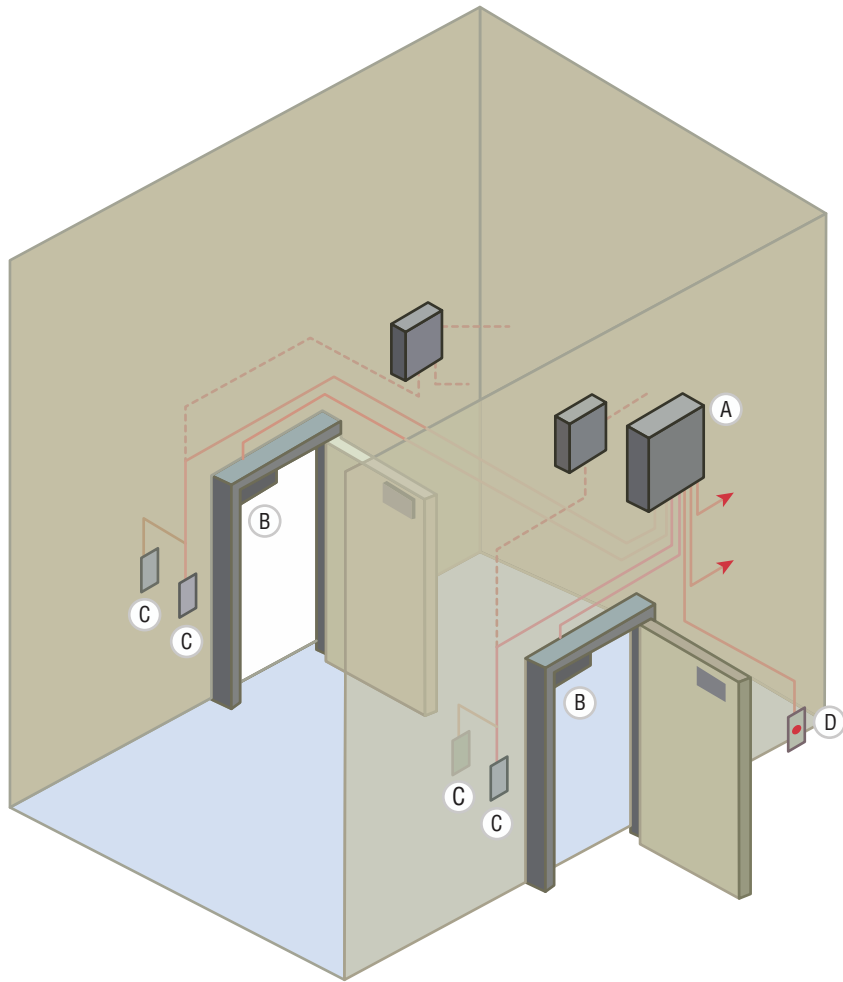
FIGURE 15.17 Mantrap
