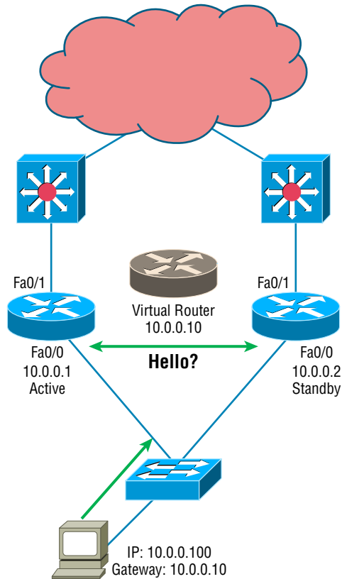
FIGURE 10.14 HSRP Hellos
