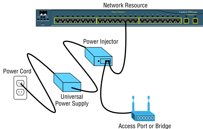
FIGURE 11.22 An external power injector used for PoE
