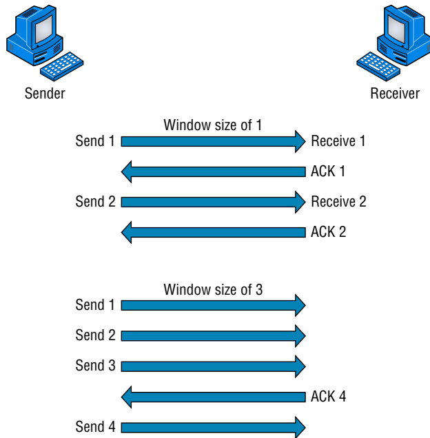
FIGURE 2.6 Windowing
