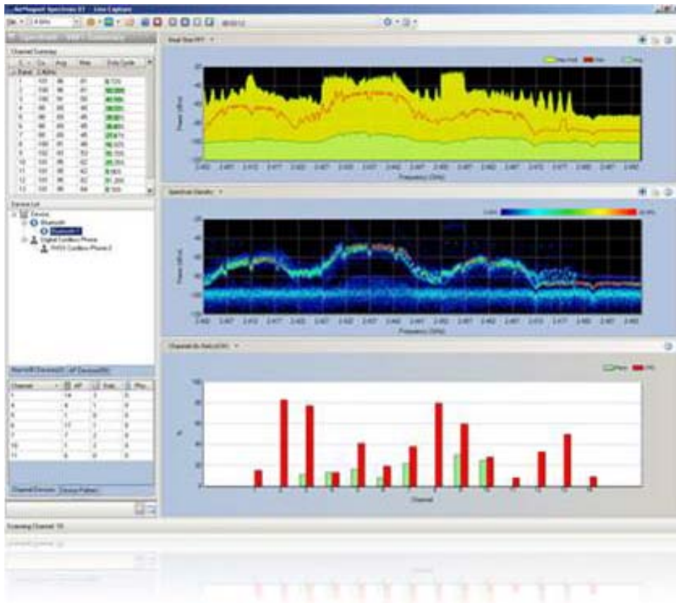
FIGURE 18.6 Wireless analyzer
