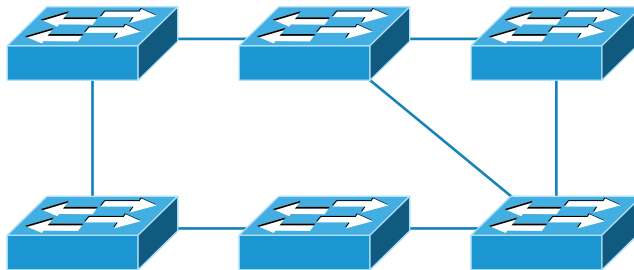
FIGURE 11.10 A switched network with switching loops
