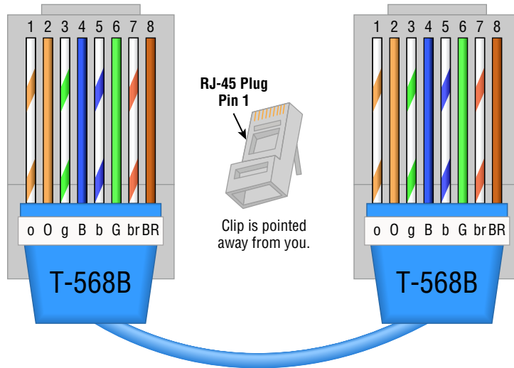
FIGURE 3.20 568B wired standard
