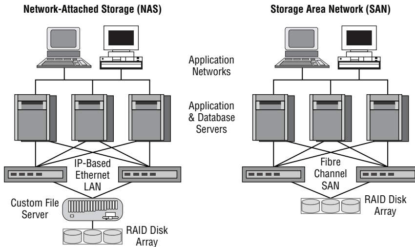
FIGURE 20.13 NAS and SAN
