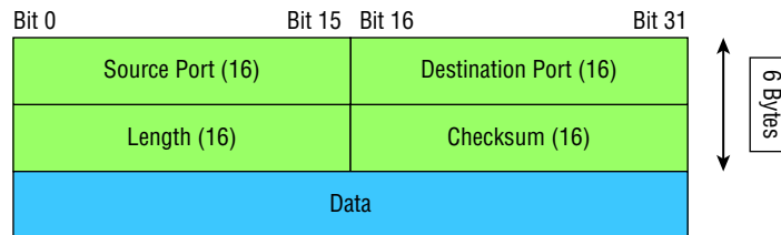
FIGURE 6.5 UDP segment
