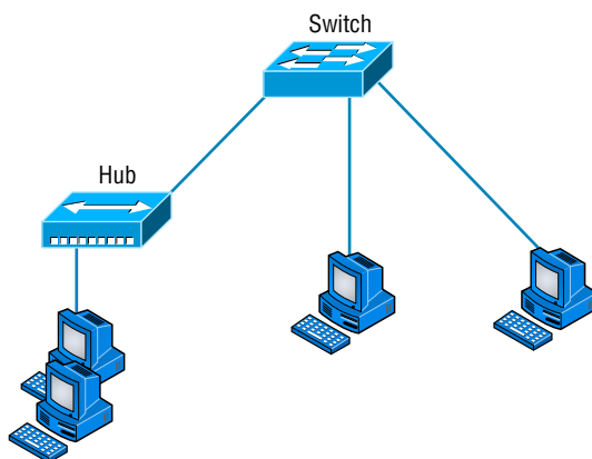
FIGURE 5.24 A switch can replace the hub, breaking up collision domains.
