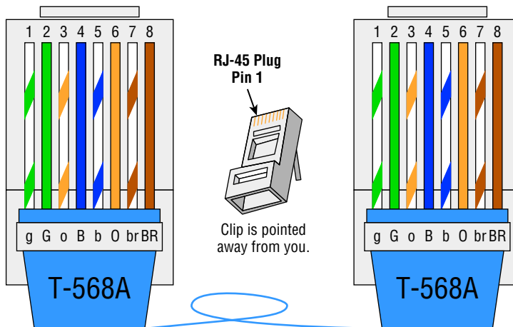
FIGURE 3.19 568A wired standard
