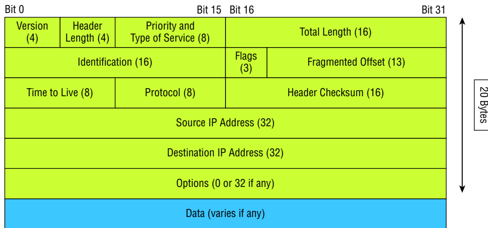
FIGURE 6.7 IP header
