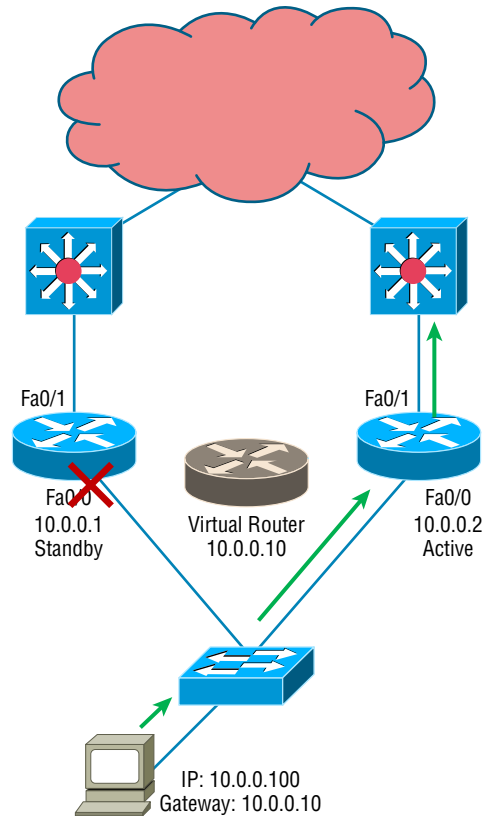
FIGURE 10.13 Example of HSRP active and standby routers swapping interfaces
