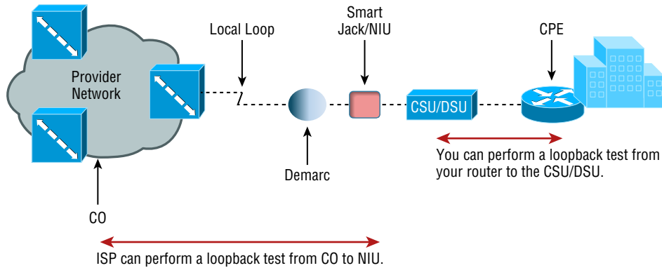
FIGURE 16.10 WAN troubleshooting spots
