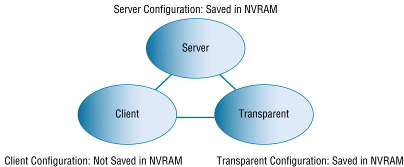
FIGURE 11.18 VTP modes
