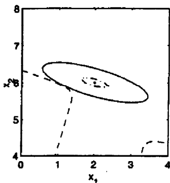
Figure 4.2: Exercise 4.29. The dotted line is the contour of \dot{V}(\bar{x}) = 0 , the dash-dot line is the contour of V(\bar{x}) = 0.007 , and the solid line is the contour of V(\bar{x}) = 0.1 .
