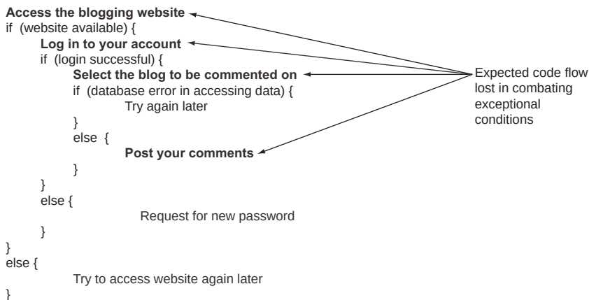
Figure 7.5 Expected code flow lost in combating exception conditions, without separate exception handlers
