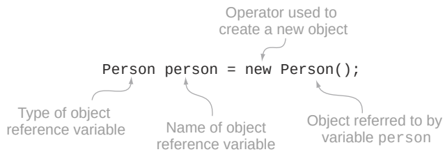
Figure 2.10 The creation and assignment of a reference variable
