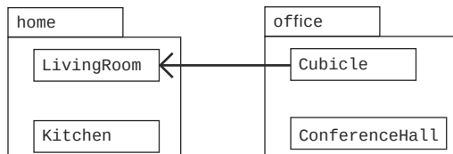
Figure 1.17 A UML representation of classes LivingRoom and Cubicle , defined in separate packages, with their associations
