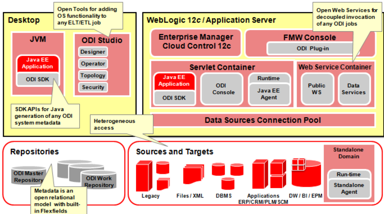
Figure 1-1 Oracle Data Integrator Component Architecture
