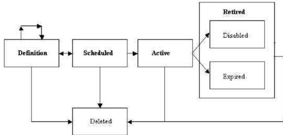
Figure 29-5 SLA Lifecycle
