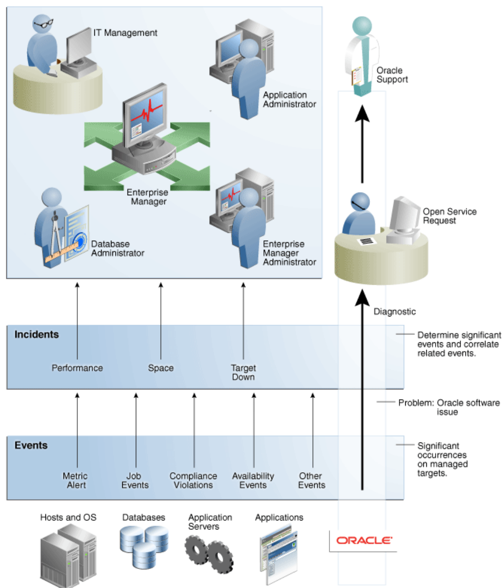
Figure 2-4 Event/Incident/Problem Flow
