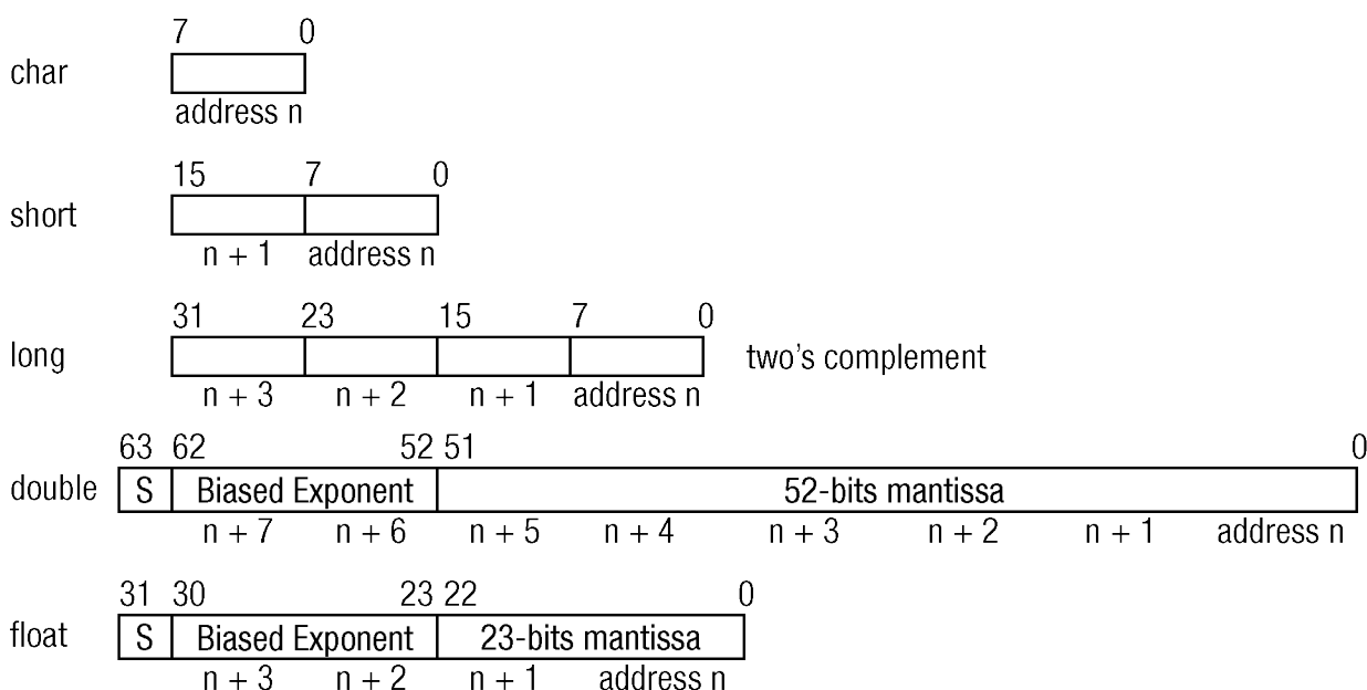
Figure 1: Byte Arrangements
