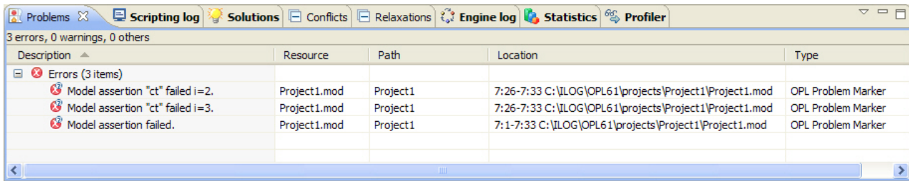
Figure 4. Labeled assert
