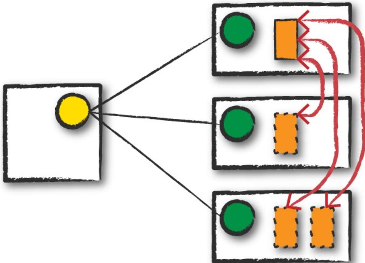
Figure 15-6. Application execution
