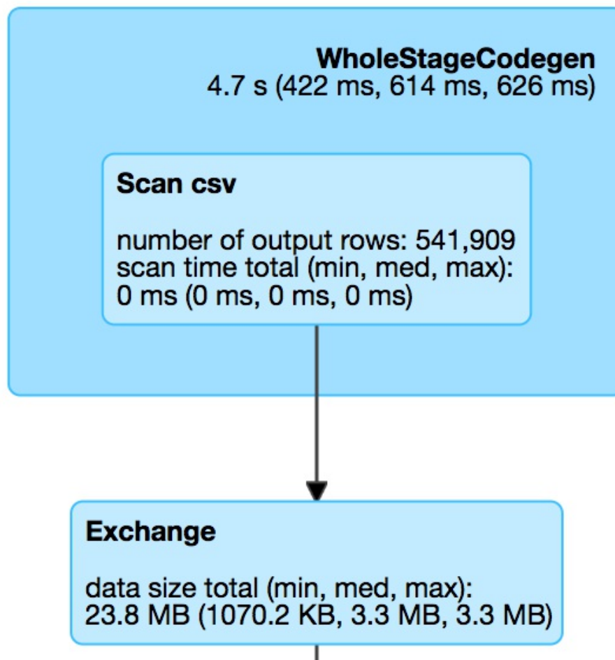
Figure 18-4. Stage one
