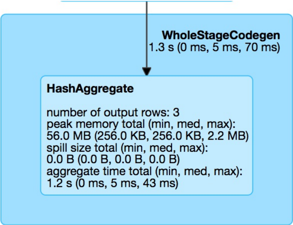
Figure 18-6. Stage three
