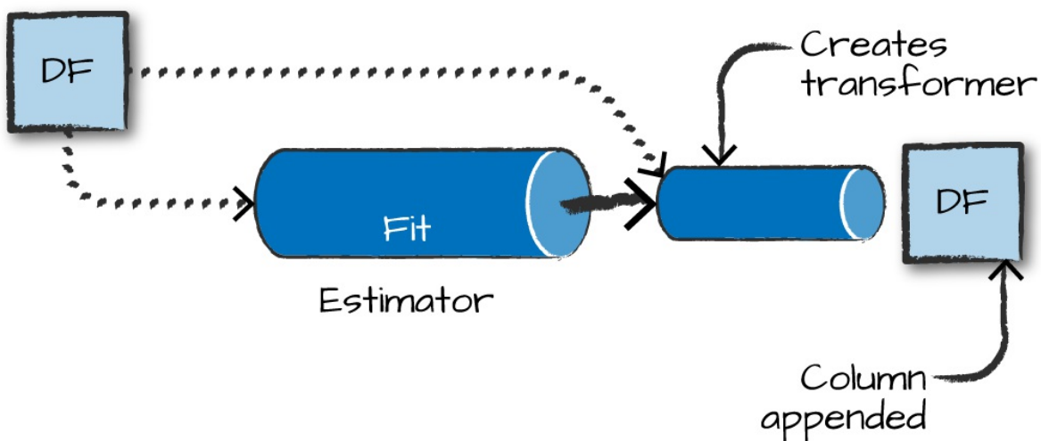
Figure 25-2. A Spark estimator
