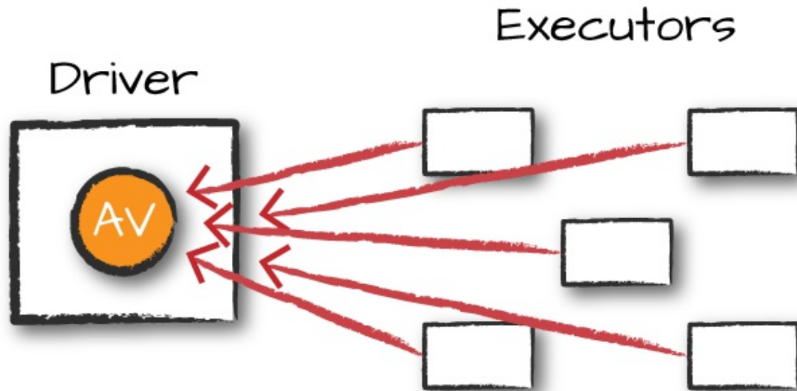
Figure 14-2. Accumulator variable
