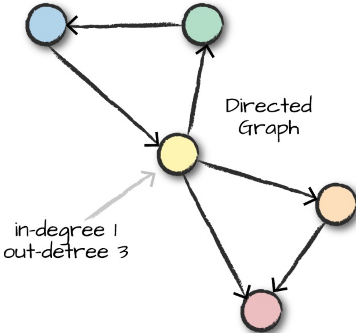
Figure 30-4. In-degree and out-degree
