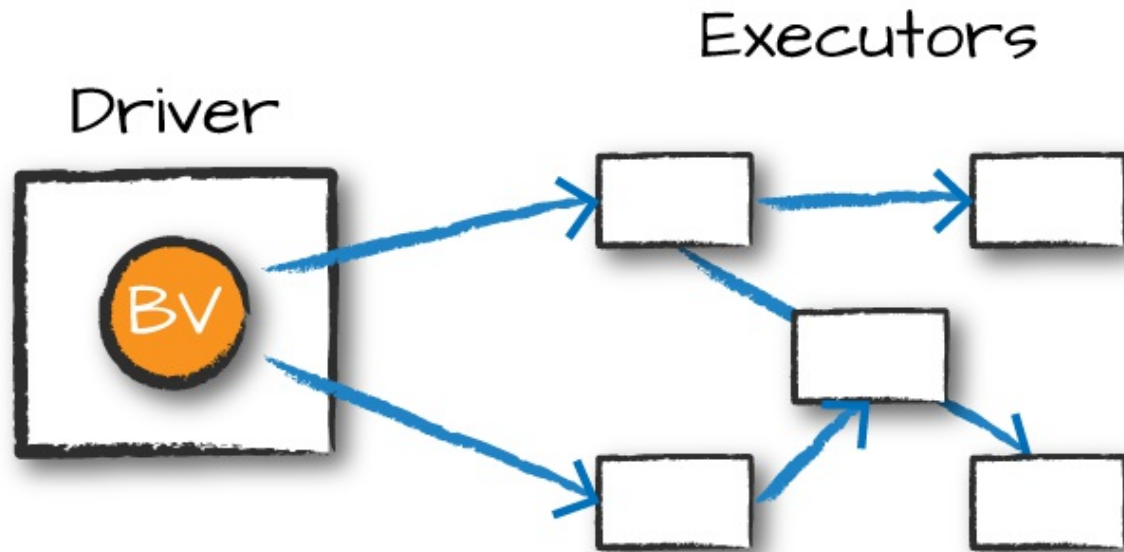
Figure 14-1. Broadcast variables
