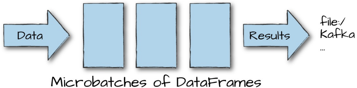
Figure 20-2. Micro-batch
