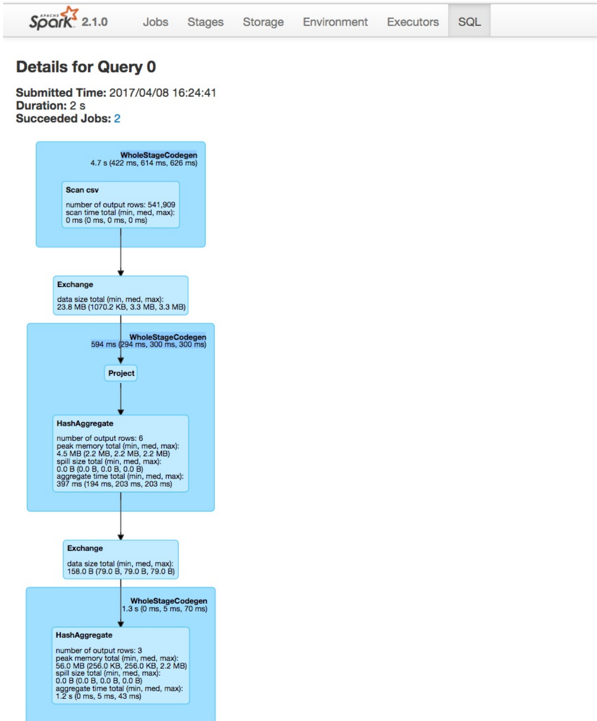
Figure 18-3. The SQL tab
