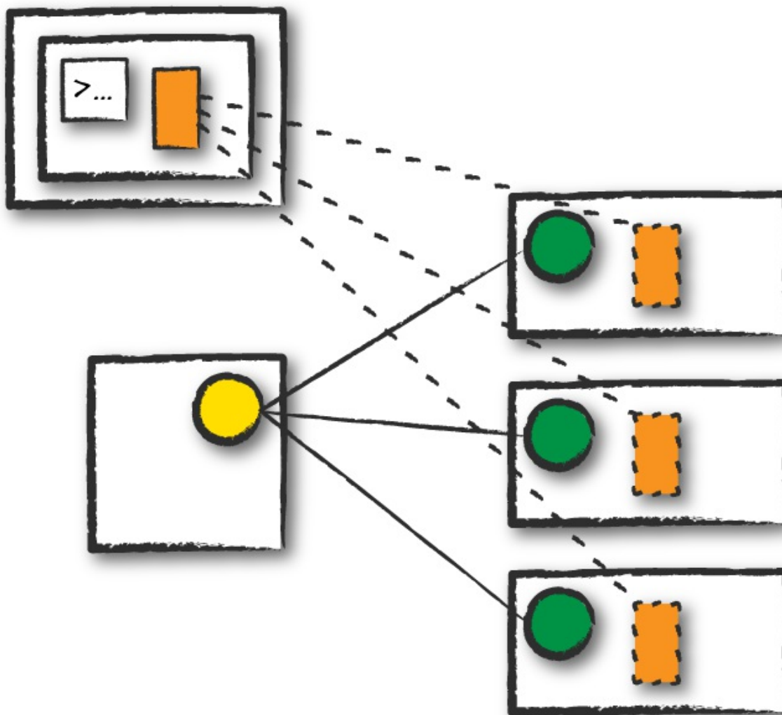
Figure 15-3. Spark's client mode
