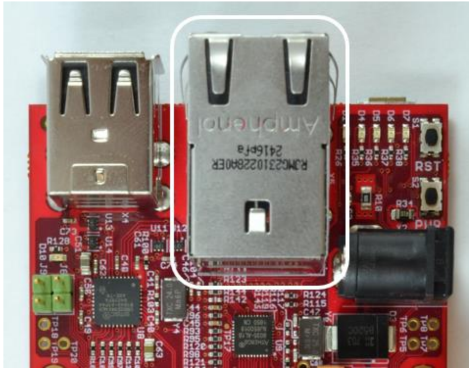
Figure 30: Ethernet port
