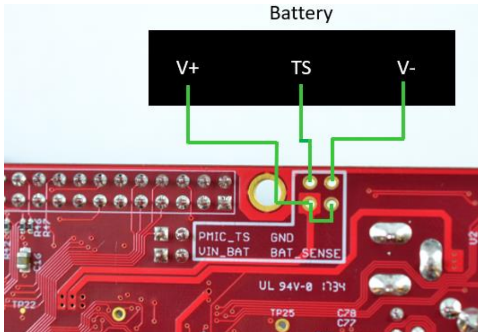
Figure 40: Battery hookup
