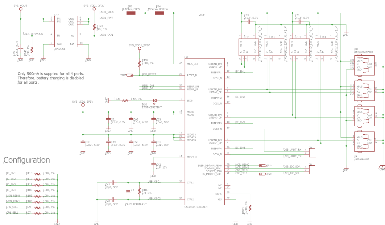
Figure 54: OSD3358-SM-RED USB host hub circuit
