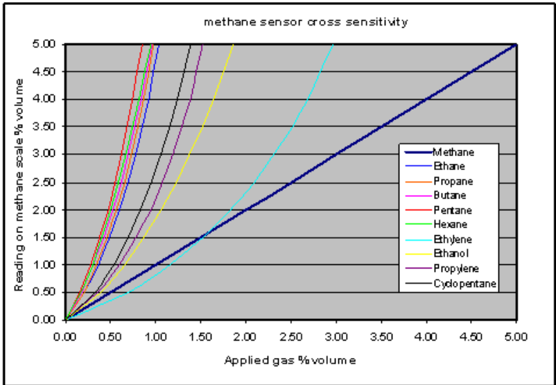
Figure 9-1 Cross-sensitivity chart for OLCT 200Methane IR Sensor.
