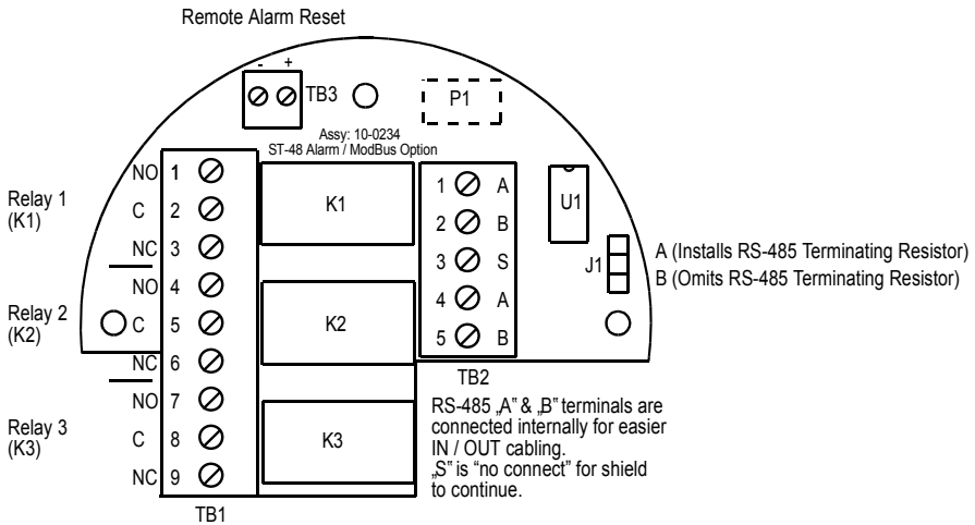
Figure 2-10: 10-0234 Alarm Relays / Modbus Option
