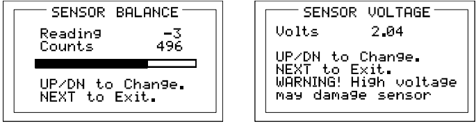
Figure 7-2: Catalytic Bead BALANCE & SENSOR VOLTS Adjust Menus
