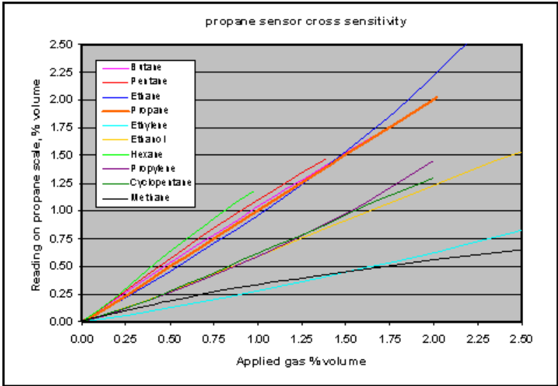
Figure 9-2 Cross-sensitivity chart for OLCT 200 Propane IR Sensor.
