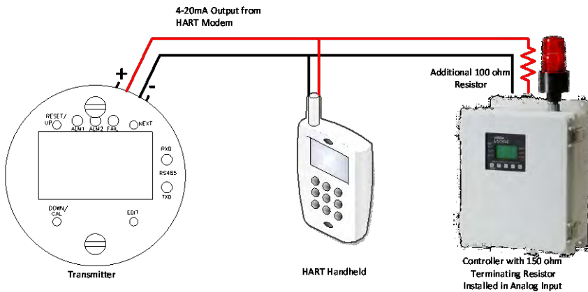
Figure 2-15: Example of OLCT 200 HART Wiring
