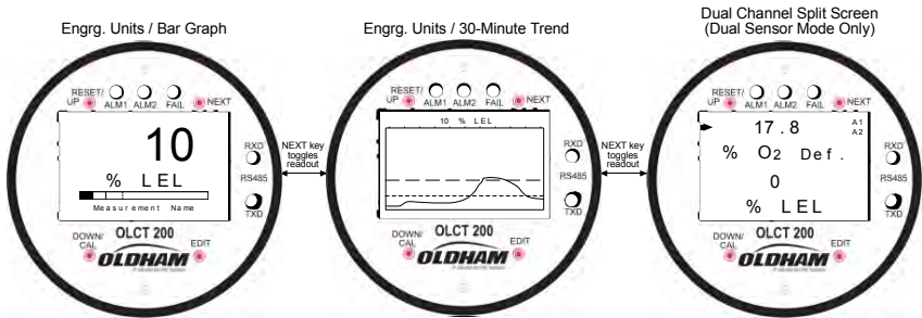
Figure 2-1a: Data Displays – 2 Wire and 3 Wire Models
