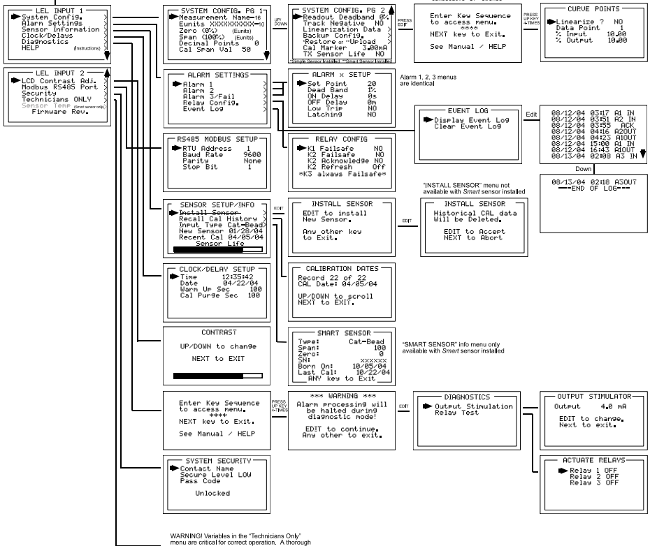
Figure 5-1a: Configuration Menu Tree-Wired Models
