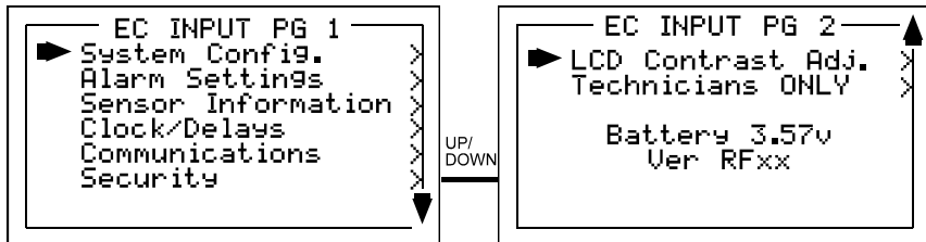
Figure 5-2b: Setup Menu Entry – Wireless Models
