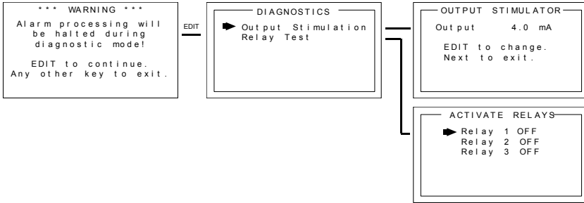
Figure 5-11: Diagnostics Menus
