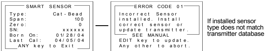
Figure 2-17: Smart Sensor Info / ERROR Screens
