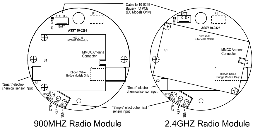
Figure 2-6: 10-0291 900MHZ / 10-0325 2.4GHZ RF Modules
