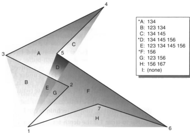
Figure 14-2 Concave Polygon
