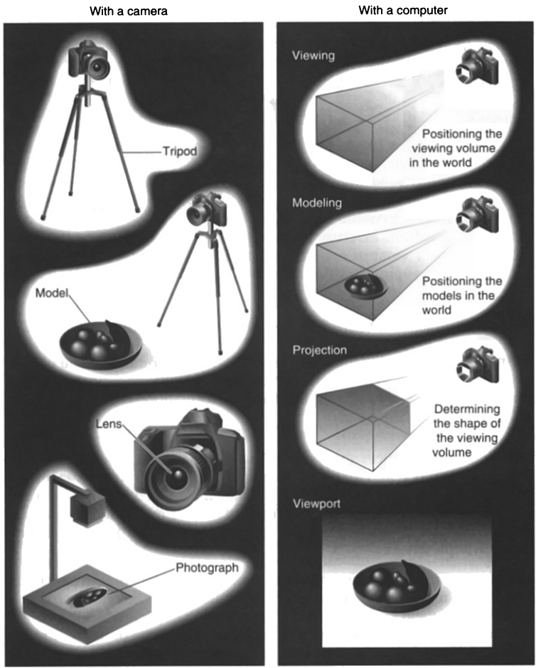
Figure 3-1 The Camera Analogy
