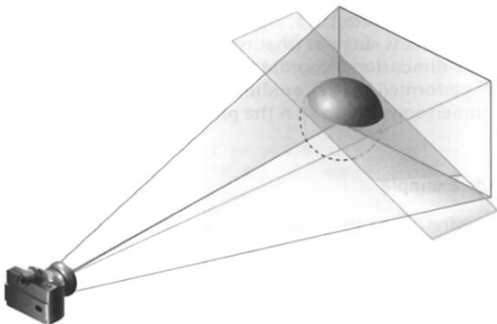
Figure 3-22 Additional Clipping Planes and the Viewing Volume
