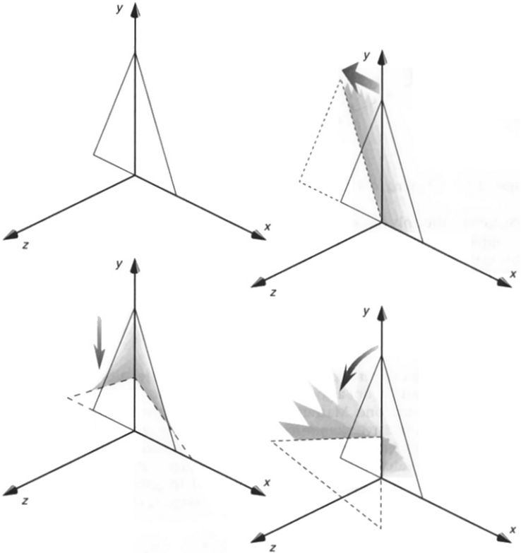
Figure 3-8 Modeling Transformation Example
