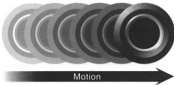
Figure 10-2 Motion-Blurred Object
