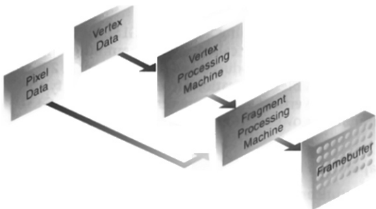
Figure 15-1 Overview of the OpenGL Fixed-Function Pipeline
