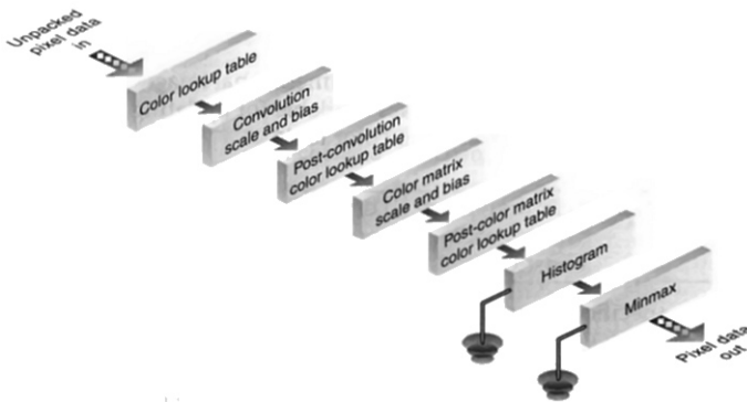
Figure 8-14 Imaging Subset Operations
