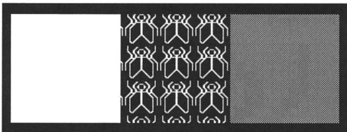
Figure 2-11 Stippled Polygons
