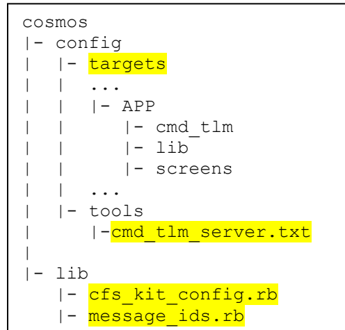
Figure 3-4 – COSMOS Directories
