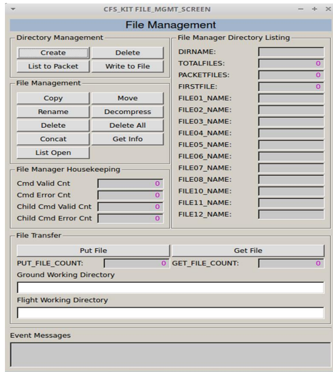
Figure 2-6 – File Management
