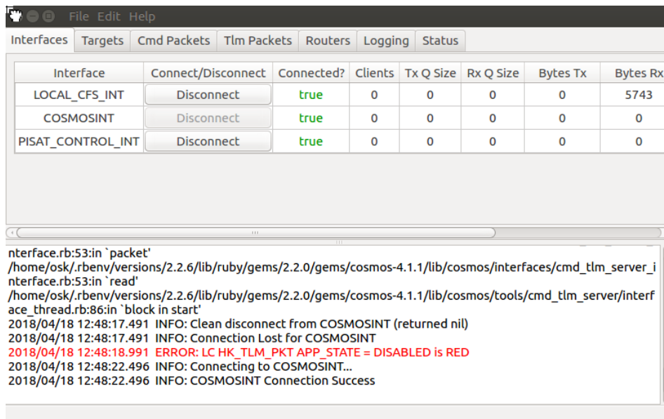
Figure 2-4 – COSMOS Command and Telemetry Server
