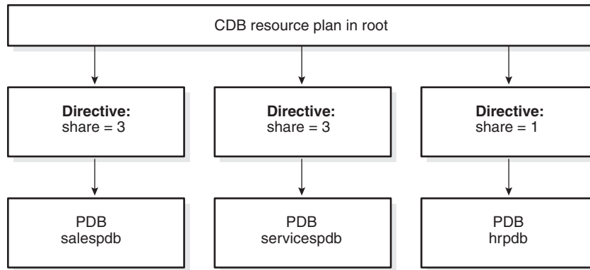
Figure 44–1 Shares in a CDB Resource Plan
