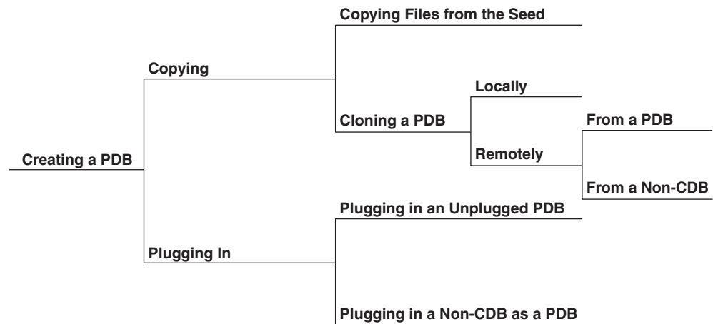
Figure 38–1 Options for Creating a PDB
