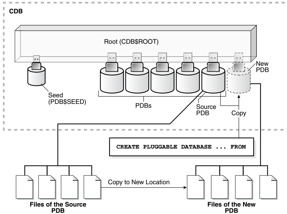
Figure 38–3 Clone a Local PDB
