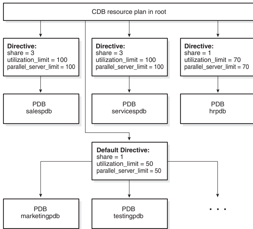
Figure 44–3 Default Directive in a CDB Resource Plan
