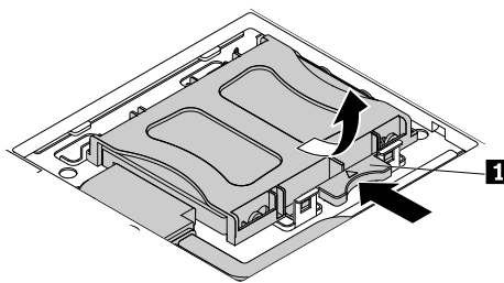
Figure 23. Removing the storage drive bracket and the storage drive
