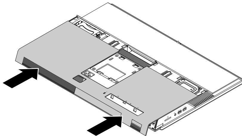
Figure 27. Installing the back cover
