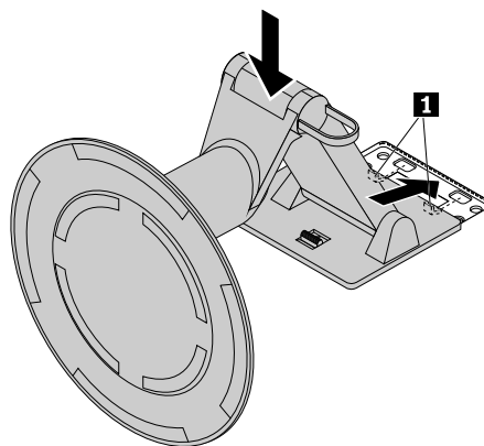
Figure 17. Installing the transformer stand to the computer cover
