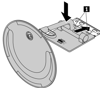
Figure 15. Installing the tilt-only monitor stand to the computer cover
