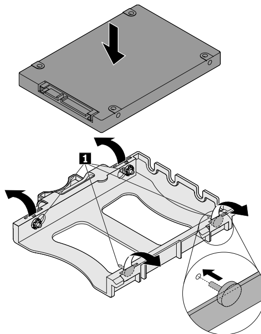
Figure 25. Installing the storage drive into the bracket
