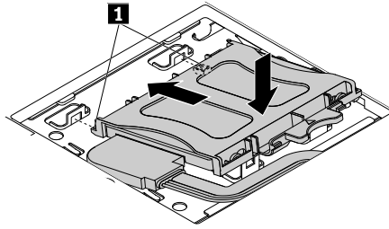
Figure 26. Installing the storage drive bracket and the storage drive
