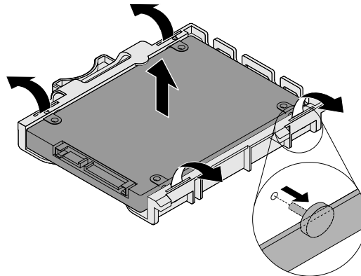
Figure 24. Removing the storage drive from the bracket
