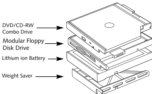
Figure 2-17 Flexible Bay Devices
