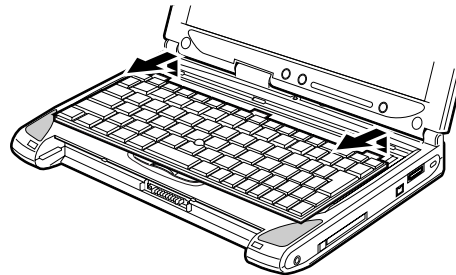
Figure 4-5 Sliding the keyboard
