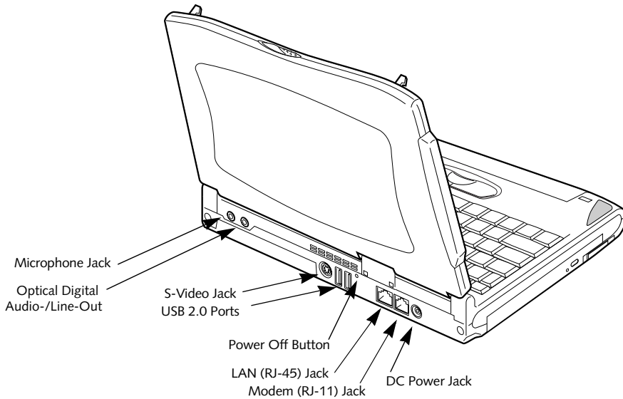
Figure 2-7 LifeBook notebook back panel
