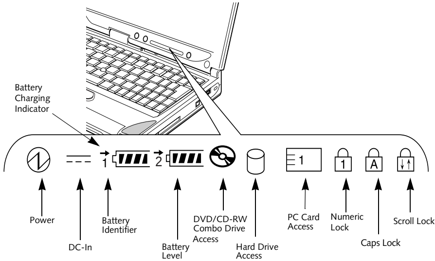
Figure 2-9 Status Indicator Panel
