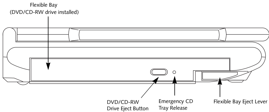
Figure 2-5 LifeBook notebook left-side panel
