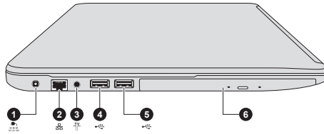
Figure 3-2 The left side of the computer
