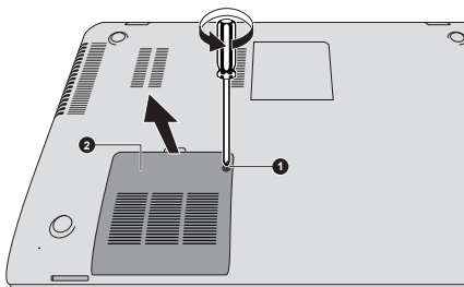
Figure 4-11 Removing the memory module cover
