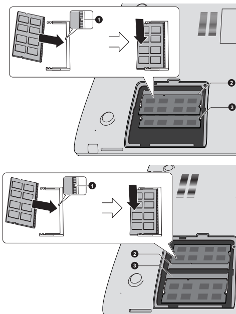
Figure 4-12 Seating the memory module
