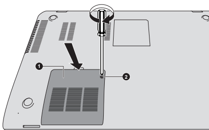
Figure 4-13 Seating the memory module cover
