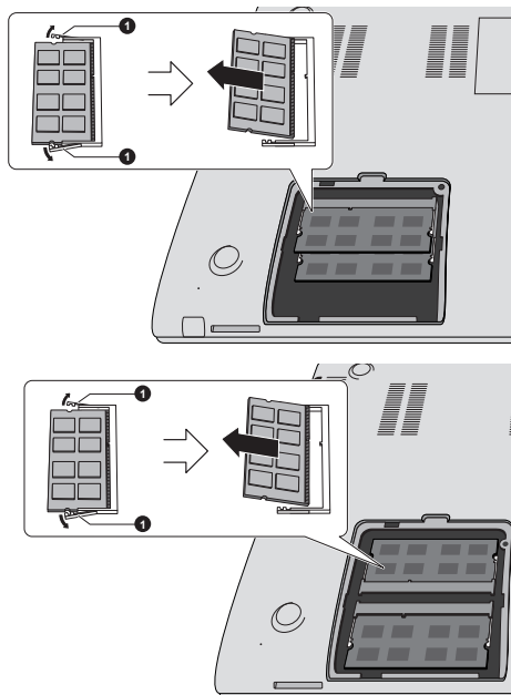
Figure 4-14 Removing the memory module
