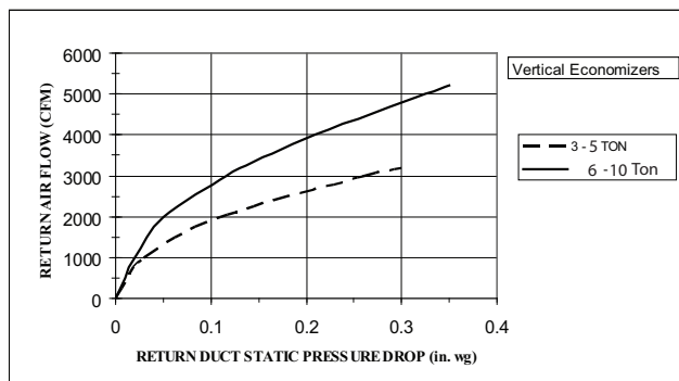
Fig. 18 - Return Air Pressure Drop-Vertical 3-10 Ton
