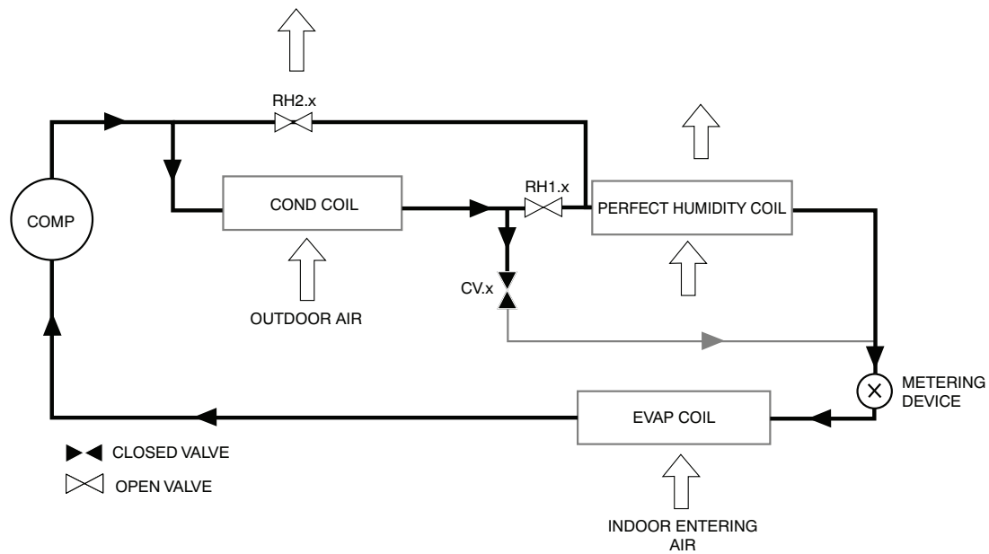
Hot Gas Reheat Mode (Reheat2) - Perfect Humidity System (581J04-14)
