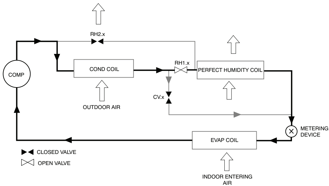
Subcooling Mode (Reheat 1) - Perfect Humidity System (581J04-14)
