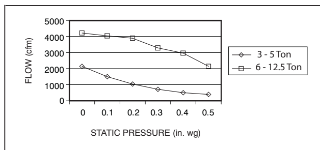
Fig. 19 - Vertical Power Exhaust Performance
