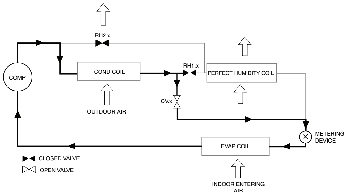
Normal Cooling Mode - Perfect Humidity System (581J04-14)
