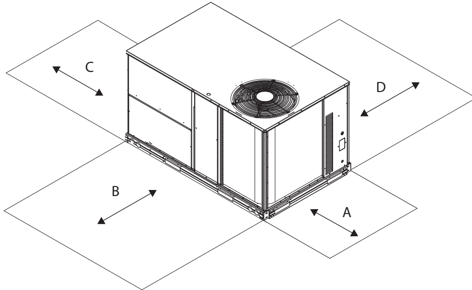
Fig. 11 - Service Clearance
