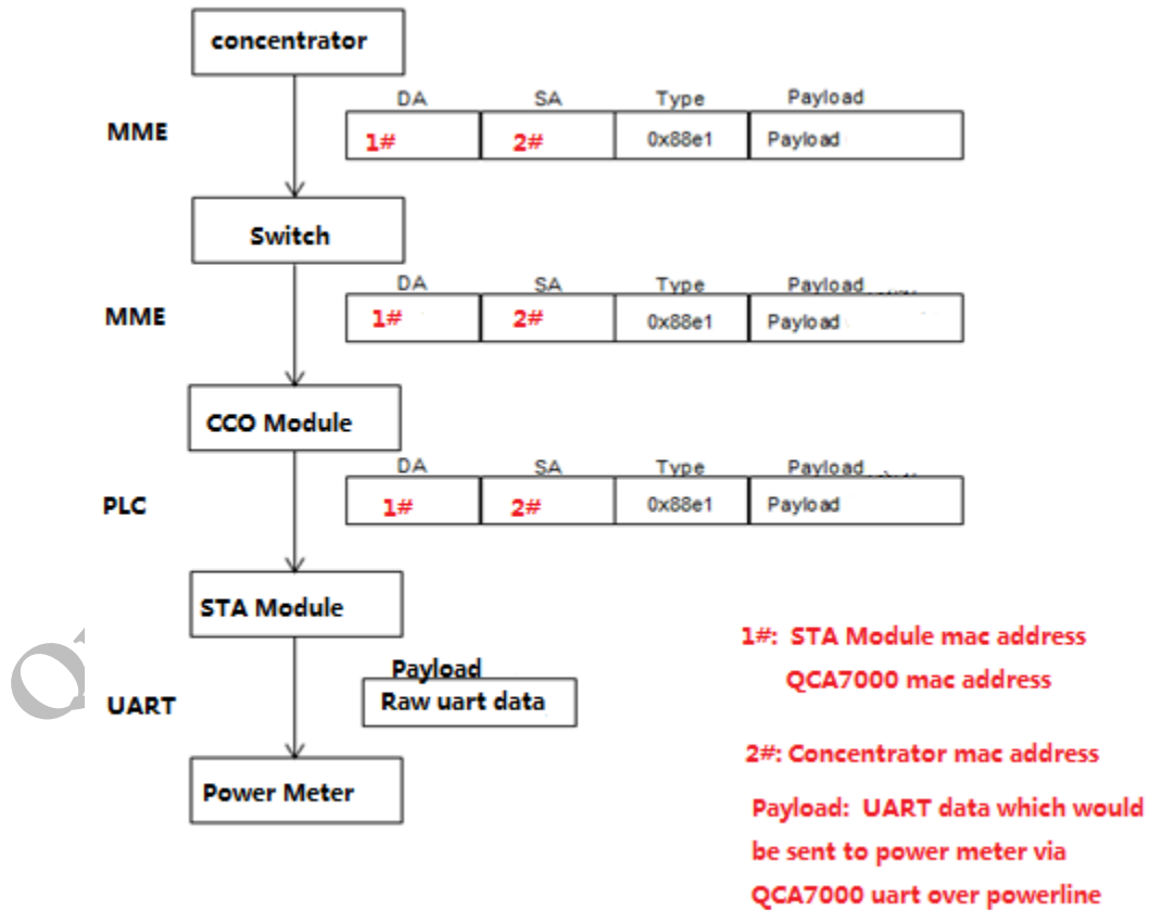
Figure 3-1: UART data transparently transmit
