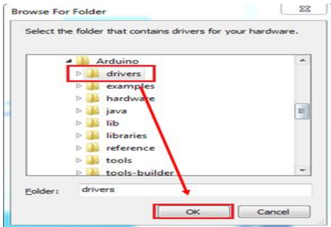
Figure 4-6 install driver
