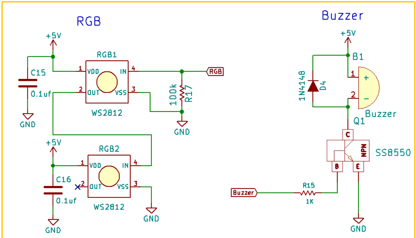
Figure 9-3 RGB LED and buzzer schematic
