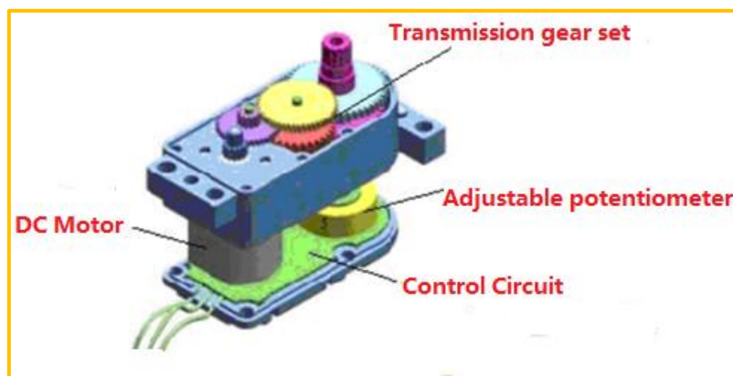
Figure11-1 Diagram of Servo
