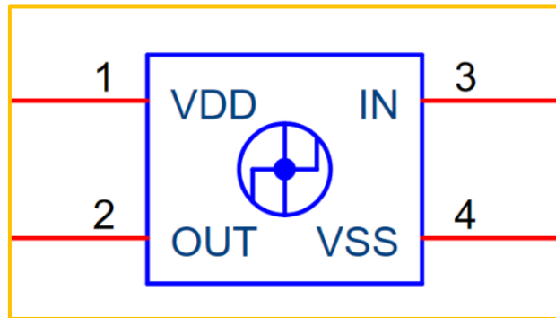
Figure 9-1 Schematic diagram of the pin function of the WS2812 chip
