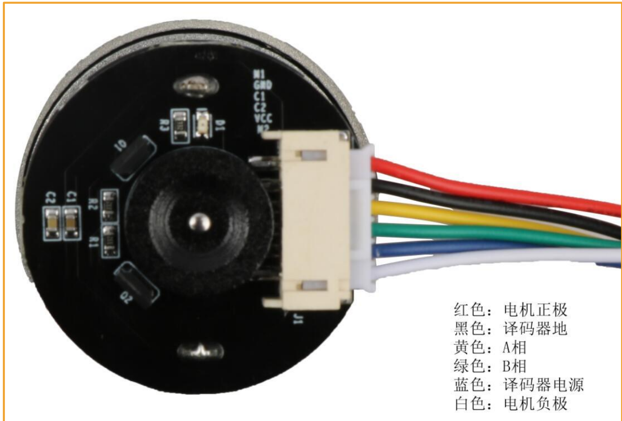
Figure 8-2 Encoder wiring diagram
