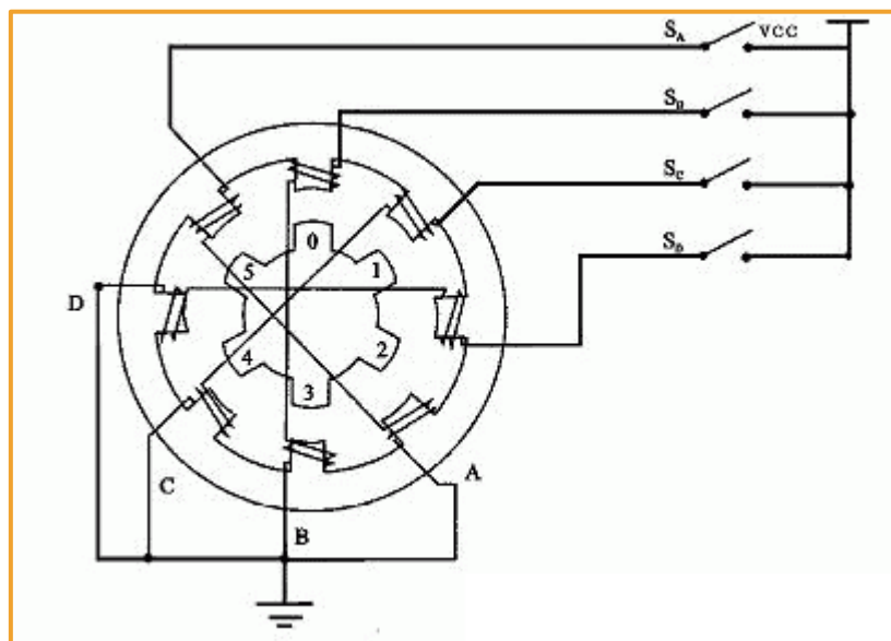
Figure 7-1 stepper motor schematic
