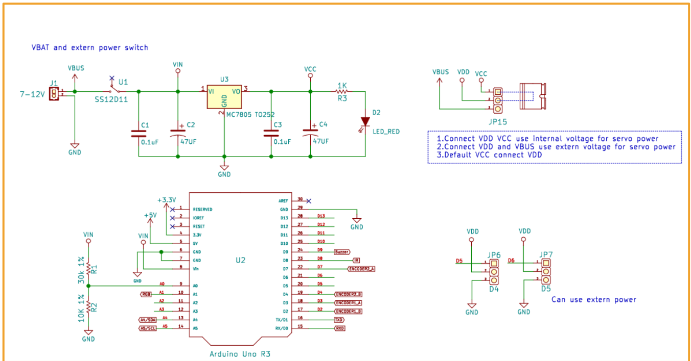
Figure 5-1 Power schematic
