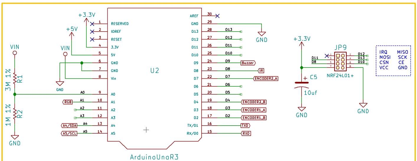
Figure 16-3 Schematic diagram of the Nrf24l01+ connection
