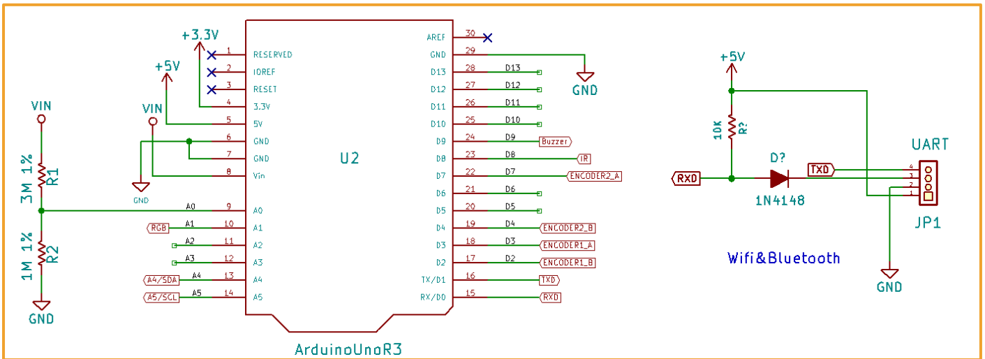
Figure 12-3 Schematic diagram of ultrasonic connection
