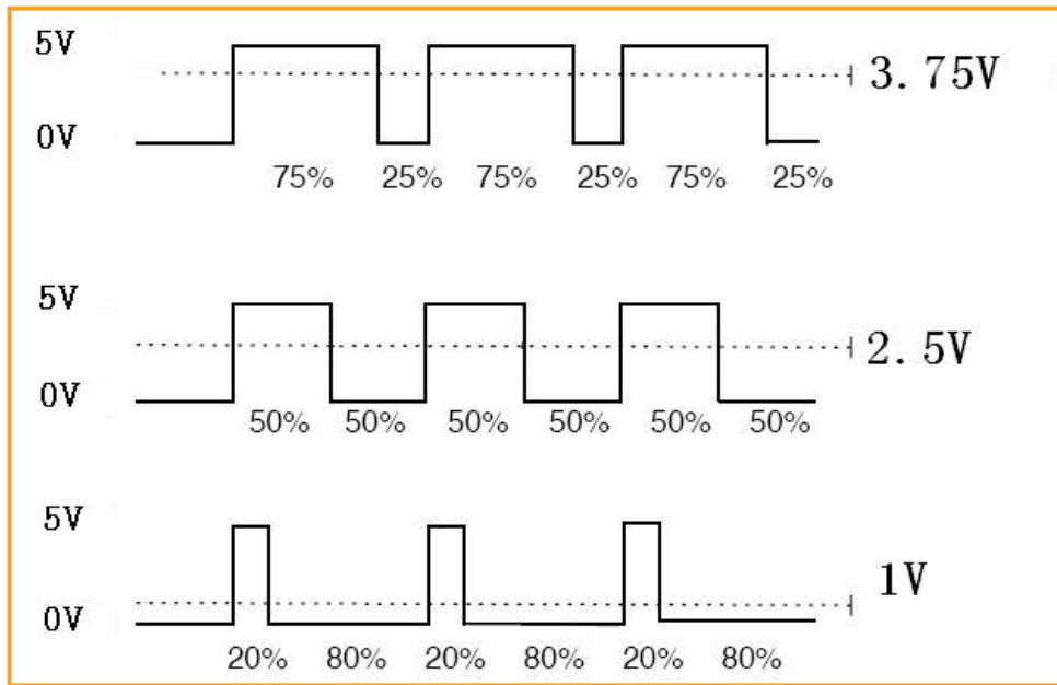
Figure 6-2 Diagram of pulse and voltage
