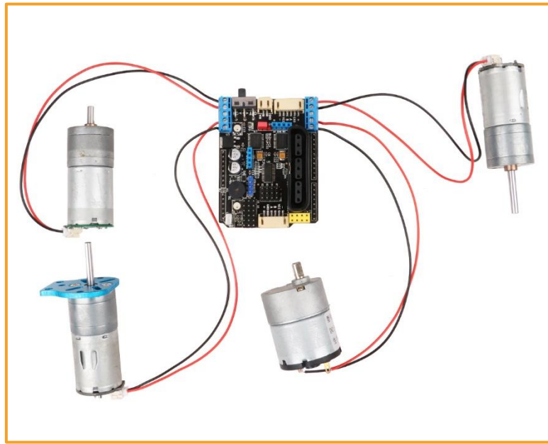
Figure 6-3 DC Motor connection diagram
