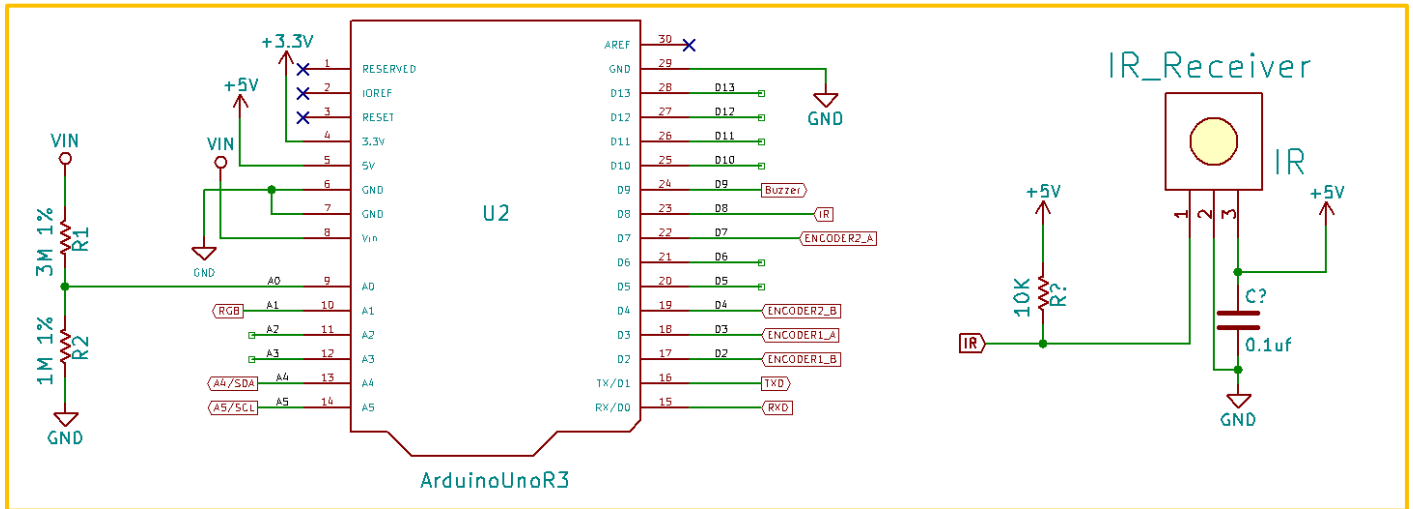
Figure 14-3 Schematic diagram of the infrared receiver connection
