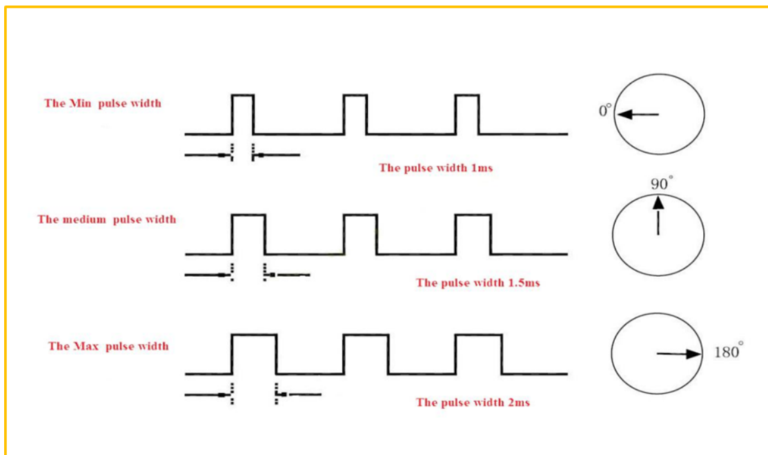
Figure 11-3 Relationship between servo output angle and input pulse
