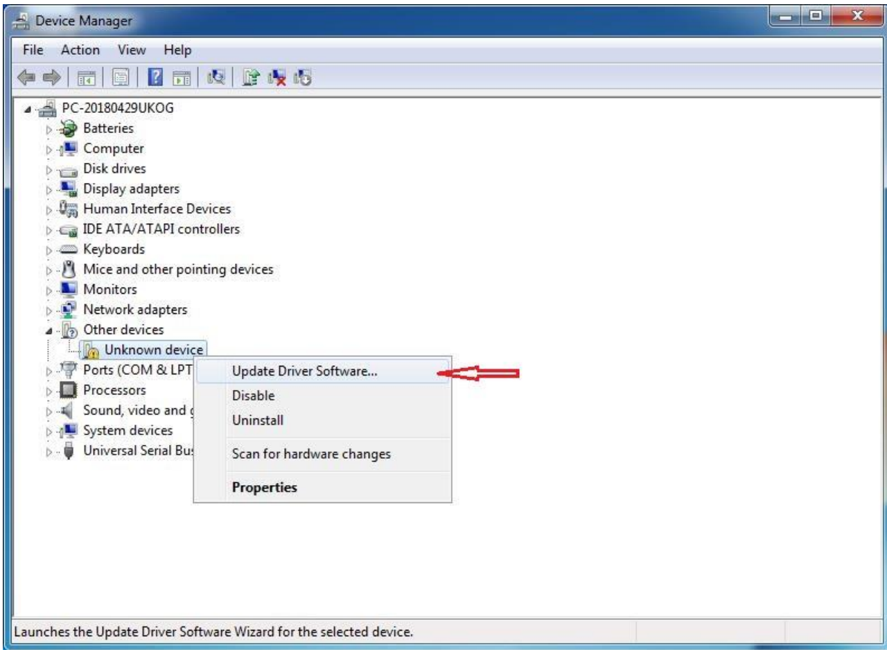
Figure 4-3 Update Driver
