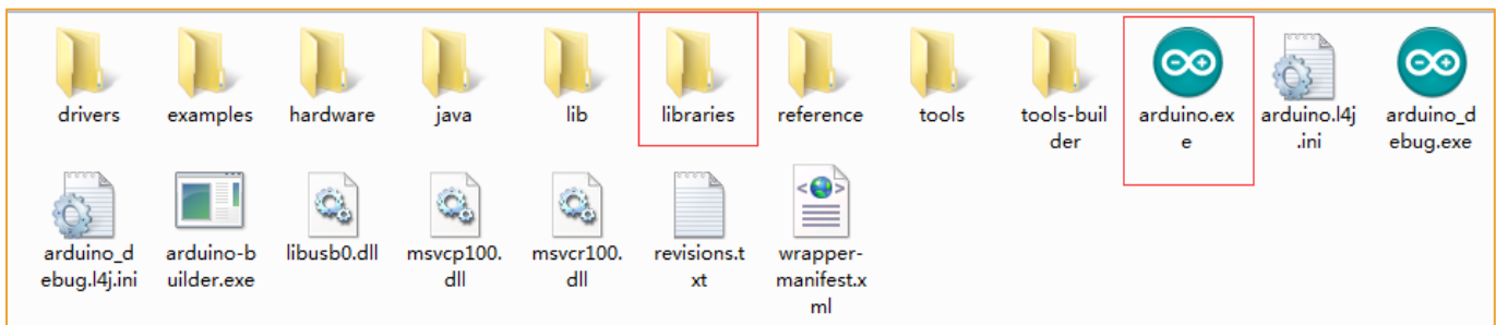
Figure 4-9 Software catalog
