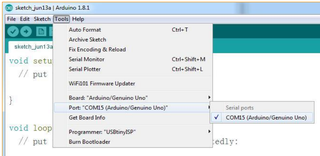
Figure 4-12 Tools interface
