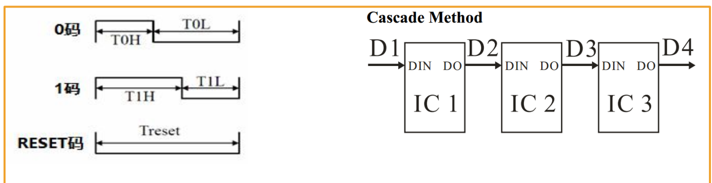
Figure 9-2 Waveform timing diagram and connection method
