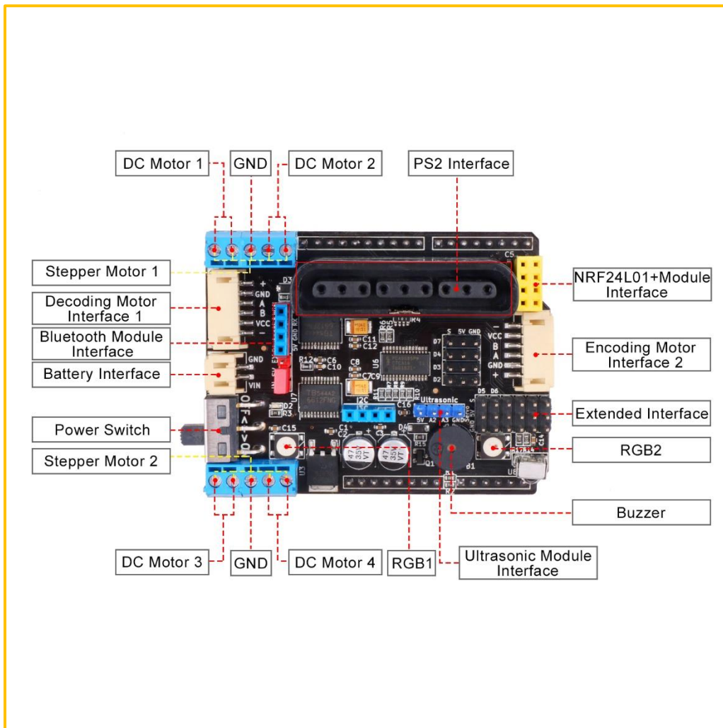
Figure 3-1 PS2X&Motor Driver Board Introduction
