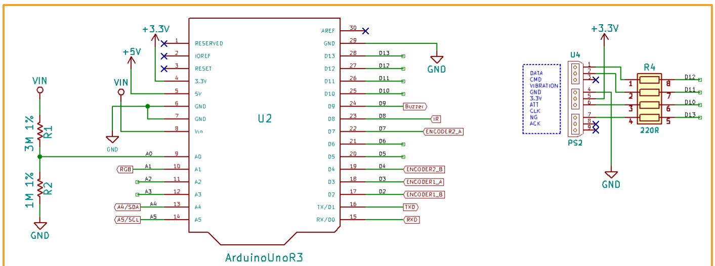
Figure 15-2 PS2 Control
