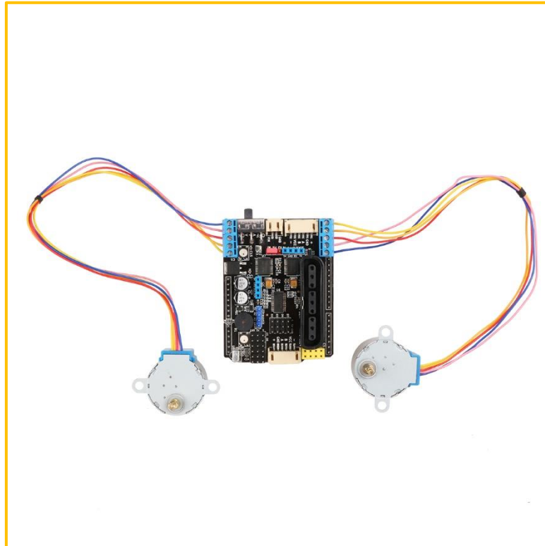
Figure 7-2 Stepper motor connection diagram
