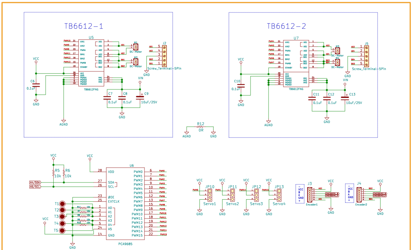
Figure 6-4 Motor drive schematic
