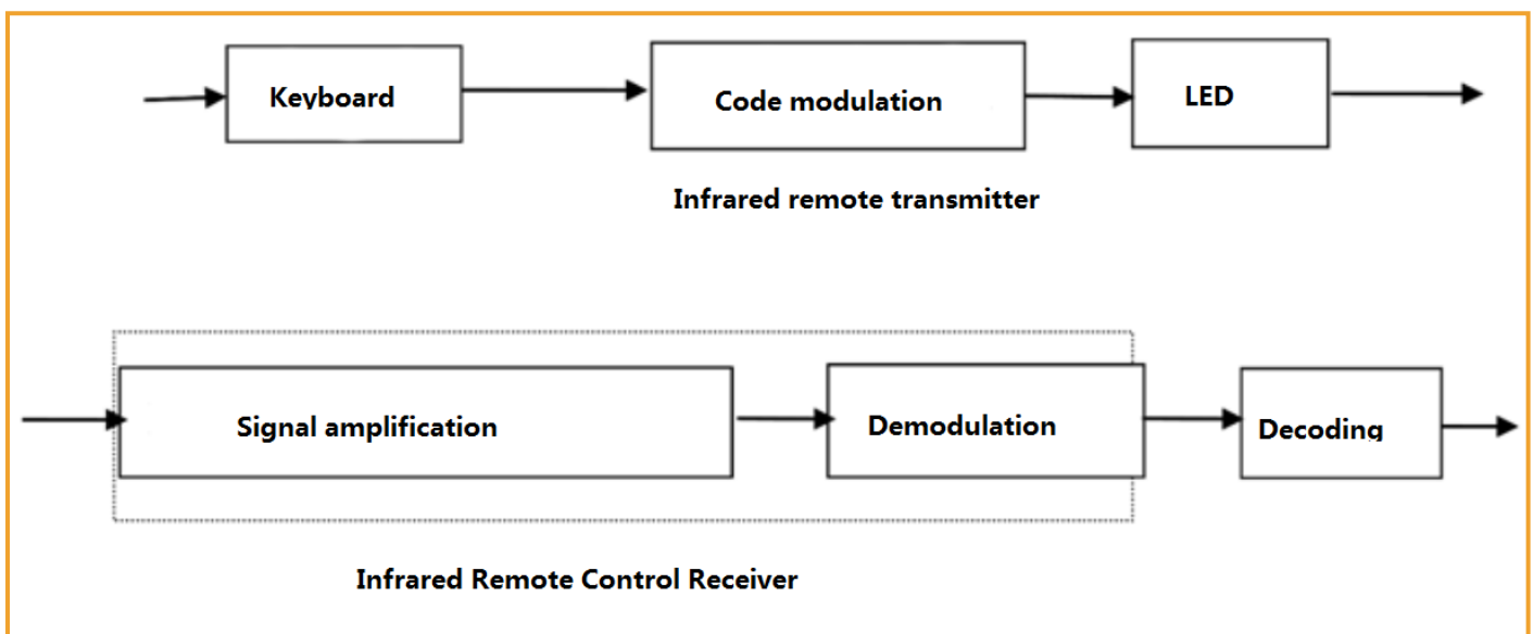
Figure 13-2 Block diagram of the infrared transmitting and receiving system
