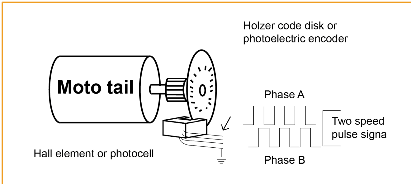
Figure 8-1 Schematic diagram of the Coded Motor
