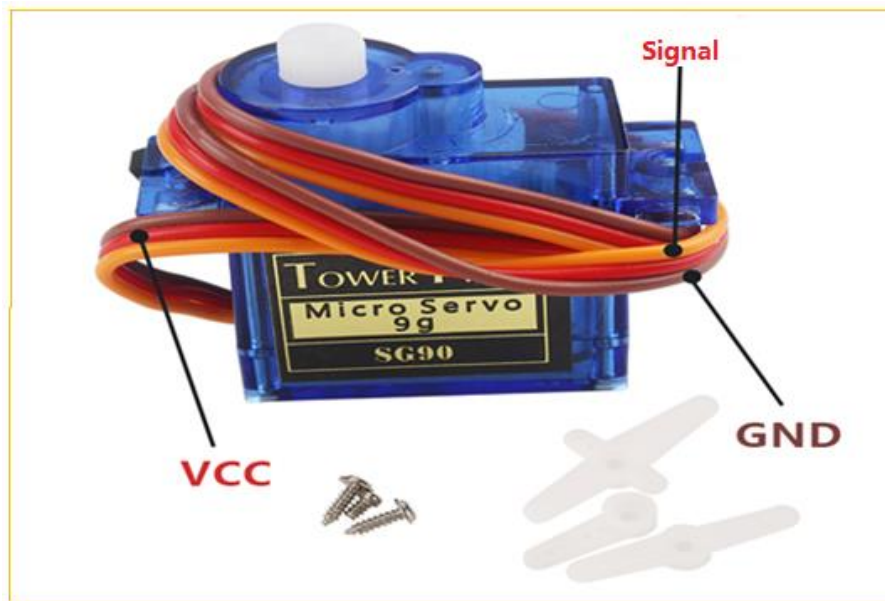
Figure 11-2 Physical diagram of the servo
